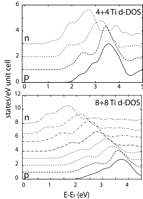
FIG. 4. Unoccupied Ti d DOS calculations for the (4+4) and the (8+8) system. For each type, n -type and p -type interfaces are indicated. Note the presence of a band gap for the (4+4) case while for (8+8) the interface remains metallic and a small Ti valency change is expected. Each layer is offset by 1 for better visibility.
