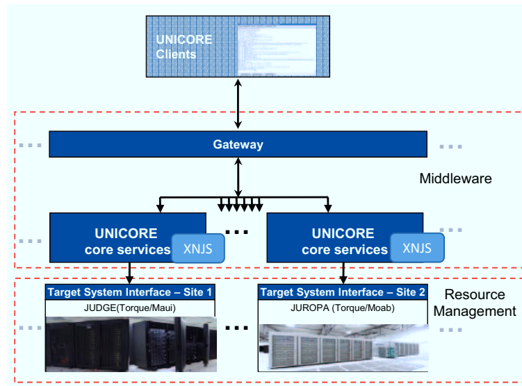
FIG. 2.1. Basic UNICORE architecture with example deployments of two HPC systems in Juelich (JUDGE and JUOPA).
