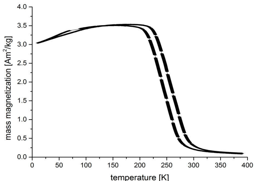
Figure 27. Isofield curve of \text{Mn}_{1.5}\text{Fe}_{3.5}\text{Si}_3 at 0.01 T.
