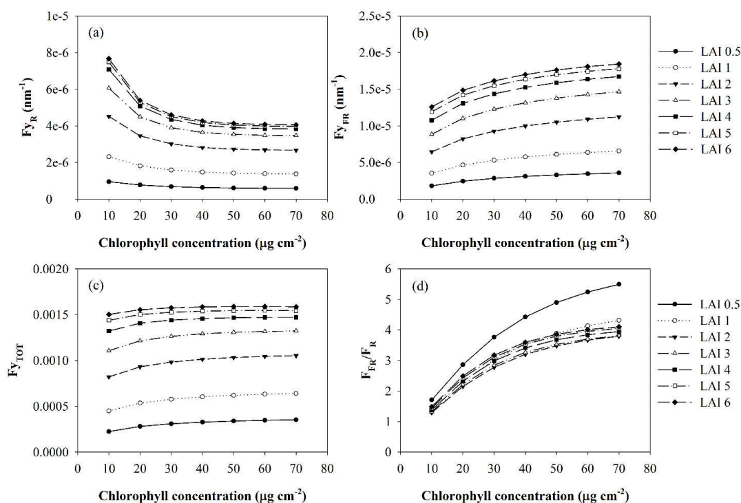
Figure 7. Simulated data. Relationships between the leaf chlorophyll concentration ( \mu\text{g cm}^{-2} ) and: (a) F_{yR} ( \text{nm}^{-1} ); (b) F_{yFR} ( \text{nm}^{-1} ); (c) F_{yTOT} ; and (d) the F_{FR}/F_R ratio. F_y is derived from SCOPE simulations for different LAI values. Values for incoming shortwave radiation were set to 1000 \text{ W m}^{-2} .
