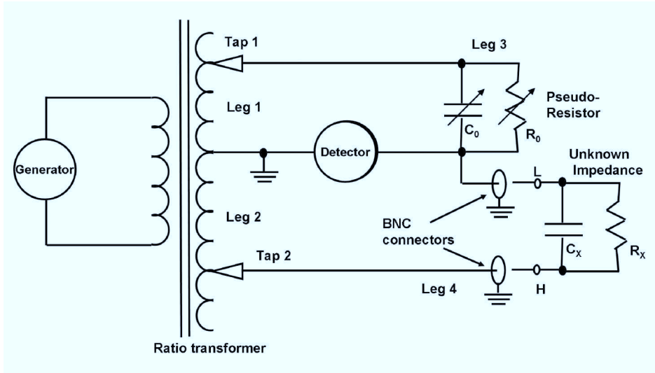
Figure 3.4: AH2700A basic bridge circuit.
