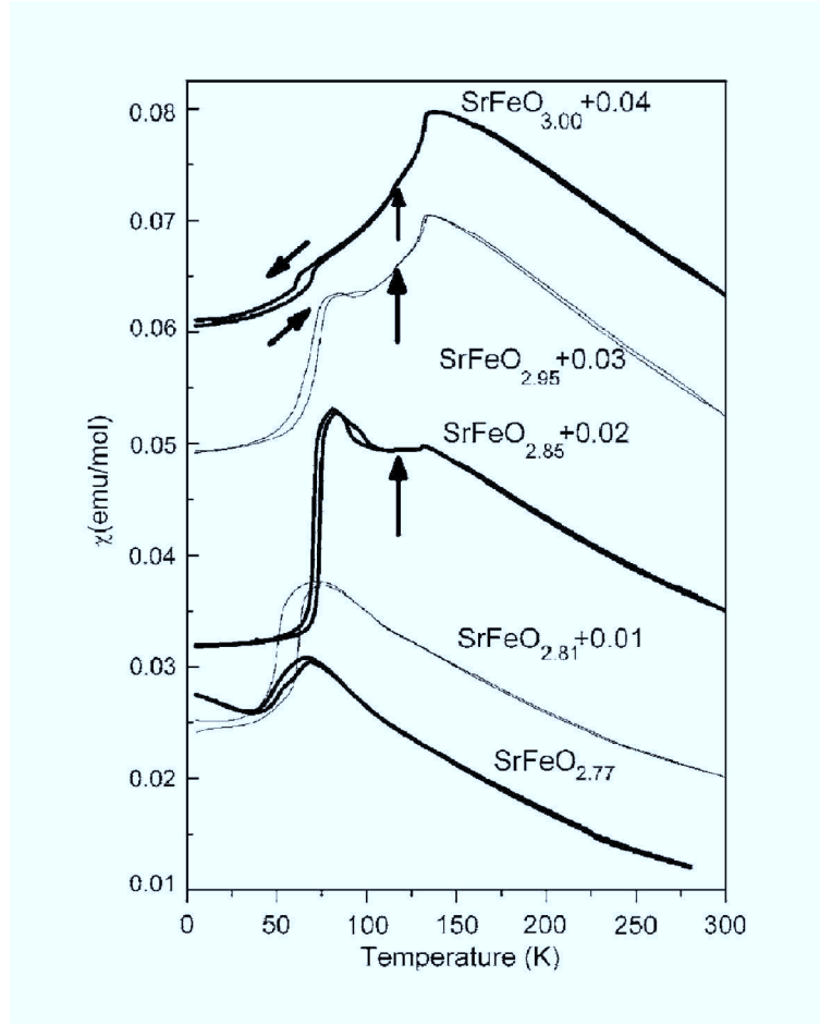
Figure 6.4: Magnetic susceptibility measurement: measured in both cooling and heating with 1 T magnetic field, taken from reference [158].
