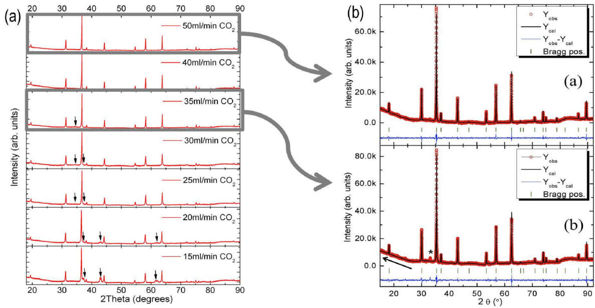
Figure 4.8: (a) Powder XRD patterns of polycrystalline \text{Fe}_3\text{O}_4 synthesized with different flow rates of \text{CO}_2 and fixed 50ml of 96% \text{Ar}/4\% \text{H}_2 (arrows indicate impurity peaks). (b) Rietveld refinement of the powder XRD patterns of (a) pure sample and (b) sample with impurities ( \text{Fe}_2\text{O}_3 impurity peak is denoted by star).
