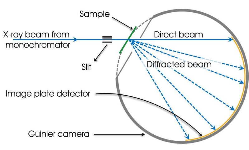
Figure 2.9: A schematic view of the powder diffractometer in Guinier geometry.
