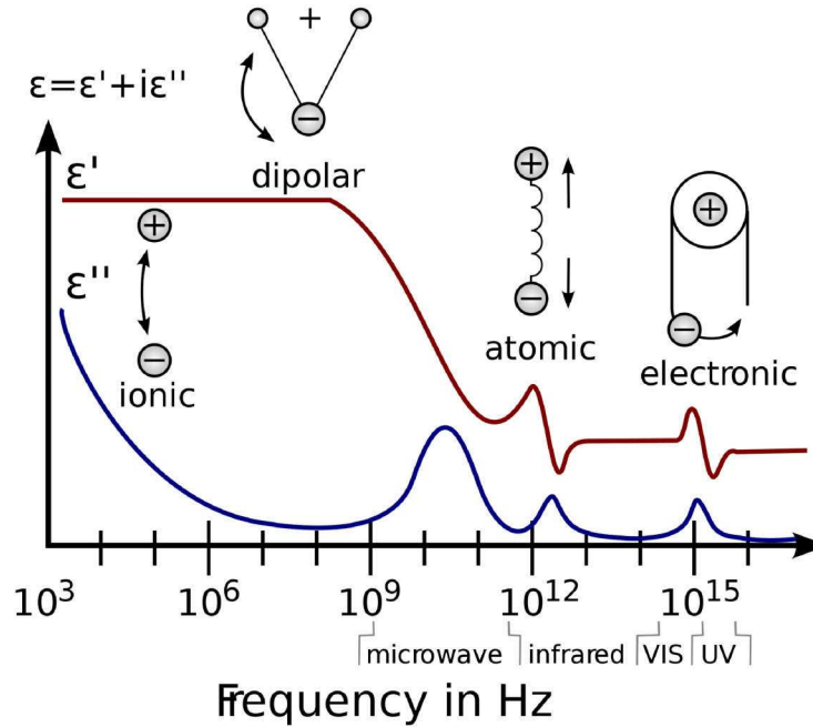
Figure 3.2: Frequency response of dielectric mechanisms.
