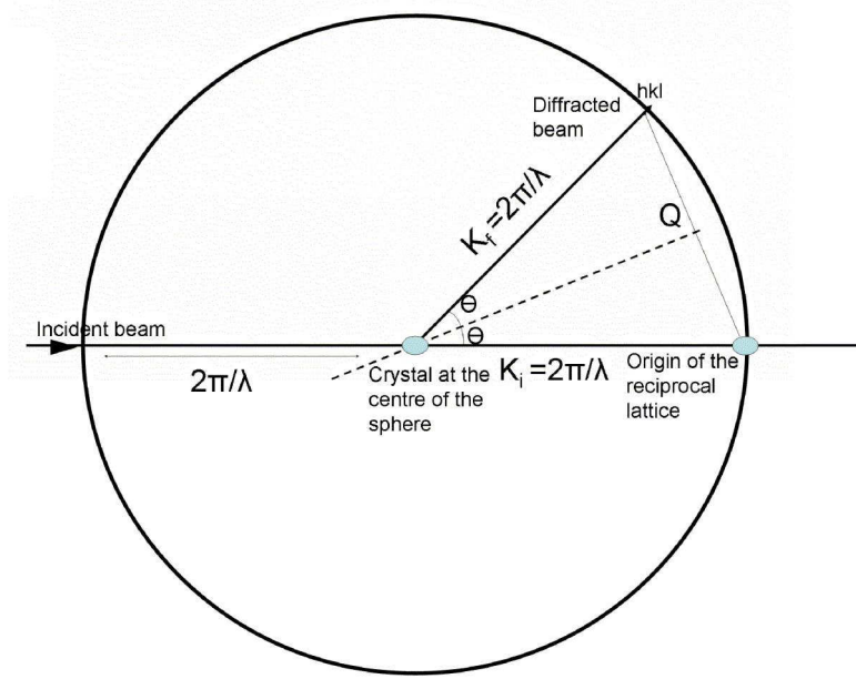
Figure 2.7: Ewald construction
