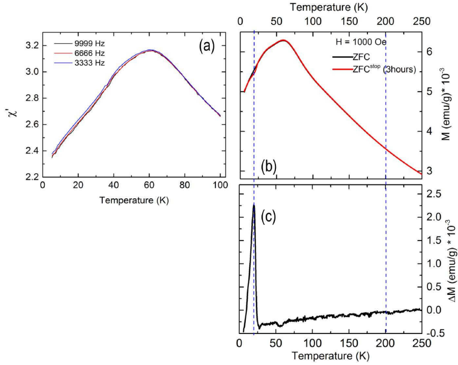
Figure 6.14: (a) Real component of the AC-susceptibility vs temperature at different frequencies. (b) Memory effect observed in the ZFC magnetization measurement. The black line represents the reference curve and the red line represents the curve measured with stop and waiting for 3 hours at 20 K and 200 K while cooling. (c) Plot of difference curve ZFC-ZFC No-Stop vs temperature.
