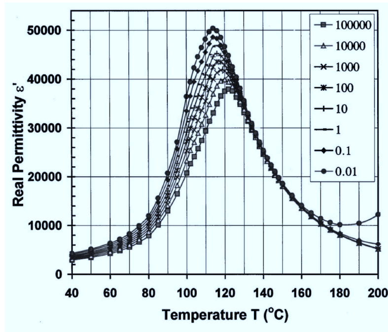
Figure 4.11: Temperature dependencies of the real part of dielectric permittivity of 0.75PMN-0.25PT ceramics, taken from reference [129]
