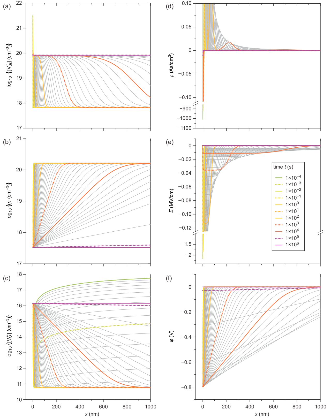
FIG. 5. Calculated equilibration of the Sr sublattice after a p\text{O}_2 jump from 10^{-10} to 10^5 Pa at 1500 K for 1 at % donor-doped \text{SrTiO}_3 . (a) Time evolution of the Sr vacancy density for t = 10^{-4} s to t = 10^6 s, referring to time range (iii) in the main text. (b) Time evolution of the electron density showing how the metal-insulation transition driven by in-diffusion of Sr vacancies proceeds into the bulk. (c) Time evolution of the O vacancy density illustrating the increase in oxygen vacancy concentration after the very strong initial depression (cf. Fig. 4). (d–f) Shows time evolution of the space charge density, the electric field, and the electrostatic potential, respectively.
