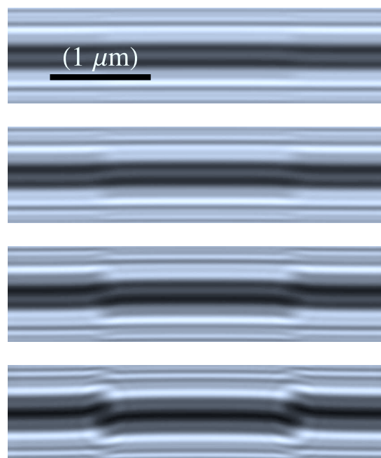
FIG. 3. Simulations of Fresnel defocus images of an opaque magnetic bar of width 90 nm at 15 mm defocus for an enclosed magnetic flux that results in a phase shift of \pi/8 , \pi/4 , \pi/2 , and \pi from the top to the bottom.
