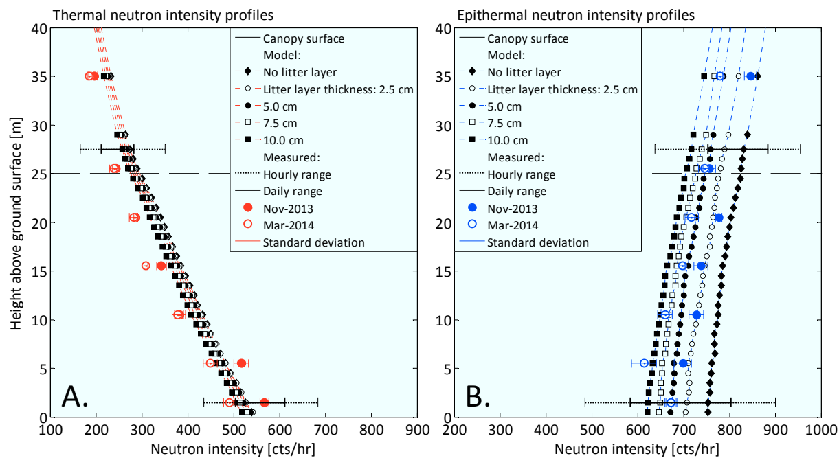
Figure 8 - Sensitivity to litter layer thickness (Model Tree trunk , Foliage , Air ). Measured and modeled (A.) thermal and (B.) epithermal neutron intensity profiles at Gludsted Plantation. Hourly and daily ranges of variation of thermal and epithermal neutron intensities at ground and canopy level for the period 2013–2015.
