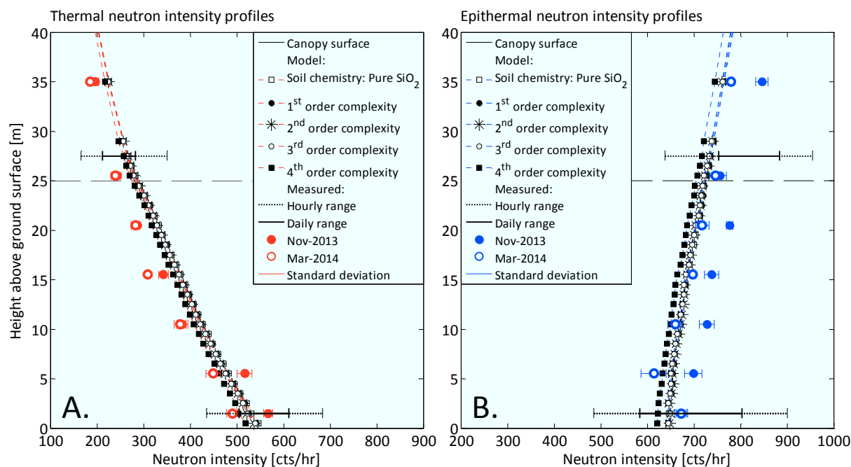
Figure 7 - Sensitivity to soil chemistry complexity ( Model Tree trunk, Foliage, Air ). Measured and modeled (A.) thermal and (B.) epithermal neutron intensity profiles at Gludsted Plantation. Five models of increasing complexity in soil chemistry are shown: 1) Pure \text{SiO}_2 , 2) First order complexity; site specific soil chemistry of the major elements (XRF), 3) Second order complexity; XRF and a Gadolinium (Gd) concentration of 0.51 ppm, 4) Third order complexity; XRF, Gd and an assumed below ground dry biomass of 25 \text{ t ha}^{-1} (roots), and 5) Fourth order complexity is the reference model shown in Fig. 3 and includes XRF, Gd, roots and measured soil organic matter. Hourly and daily ranges of variation of thermal and epithermal neutron intensities at ground and canopy level for the period 2013–2015.
