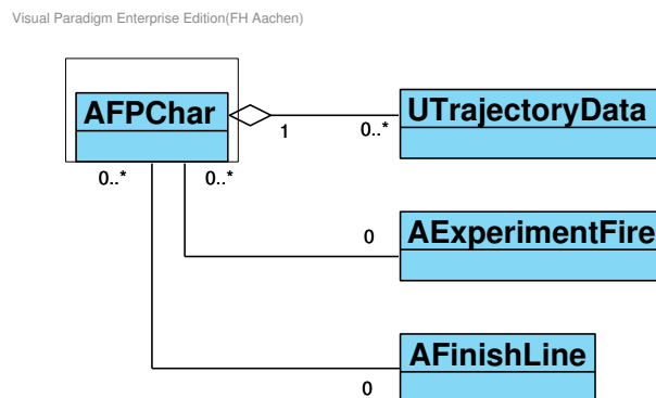
Figure 3.9: Simplified class diagramm for the experiment level
