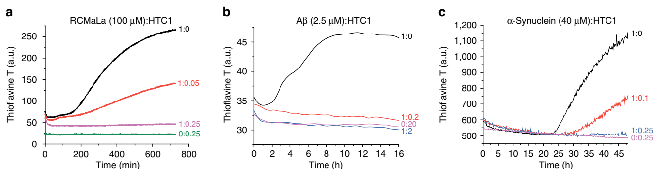
Figure 4 | HTC1 aggregation inhibition. HTC1 prevents amyloid formation of RCMaLa (a) A\beta_{1-40} (b) and \alpha -synuclein (c), as measured by thioflavin T (ThT) fluorescence at 490 nm.
