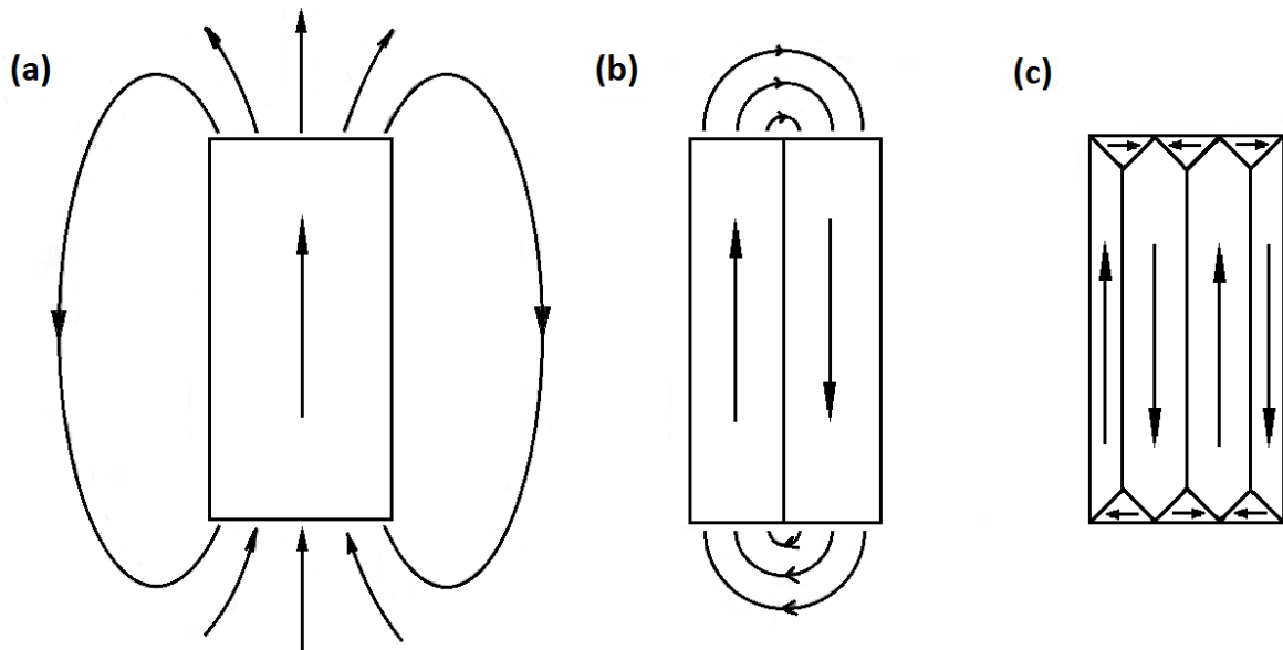
Figure 1: Different domain structures for ferromagnetic material: (a) single domain state, (b) two domains, (c) closure domains state.
