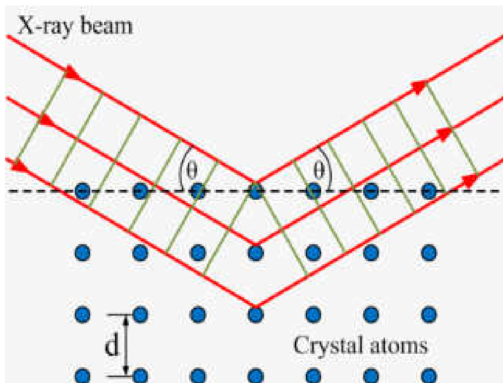
Figure 10: X-ray diffraction scheme. This shows that the difference in path length between X-ray beams incident on a stack of atomic planes is 2d \sin\theta . The condition for constructive interference of two waves is that they must be shifted by an integral number of wavelengths. Picture taken from http://ssp.physics.upatras.gr/x-ray diffraction.
