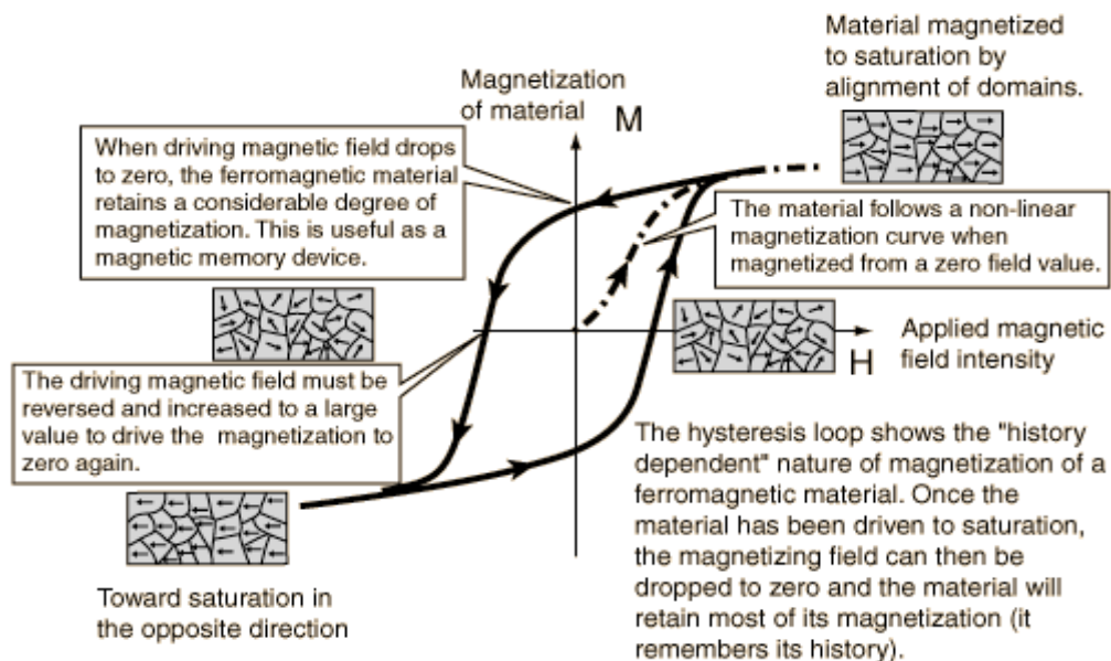
Figure 2: Hysteresis loop. Ref: [ http://hyperphysics.phy-astr.gsu.edu/hbase/solids/imgsol/hyloop.gif ]
