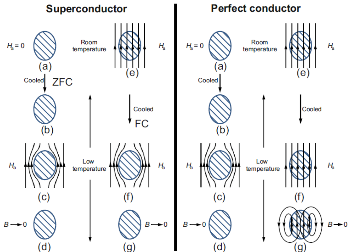
Figure 4: Schematic behavior of applied field H_a and magnetic flux density B in field-cooled and zero-field-cooled experiments on a type I superconductor and non-superconducting material with perfect conductivity.
