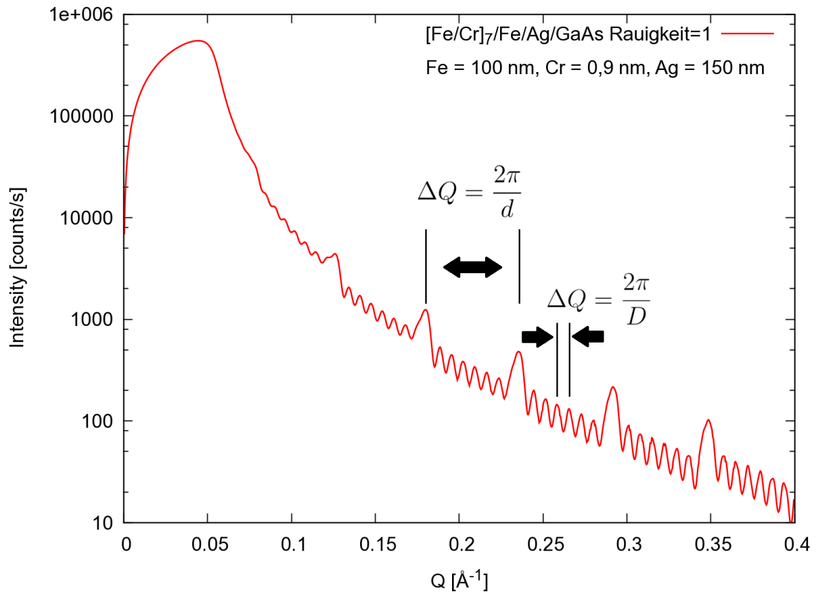
Figure 8: Simulation of a reflectivity measurement of a multilayer Fe/Cr-system. Picture taken from [2]
