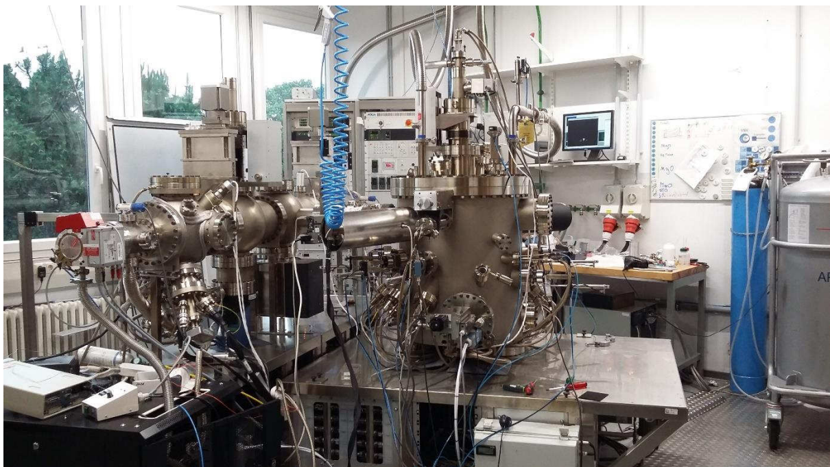
Figure 12: Molecular Beam Epitaxy Machine for Sample Preparation in Juelich Research Centre
