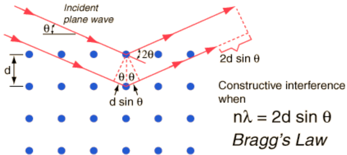
Figure 7: Schematic of Bragg scattering condition. Picture taken from http://hyperphysics.phy-astr.gsu.edu/hbase/quantum/bragg.html
