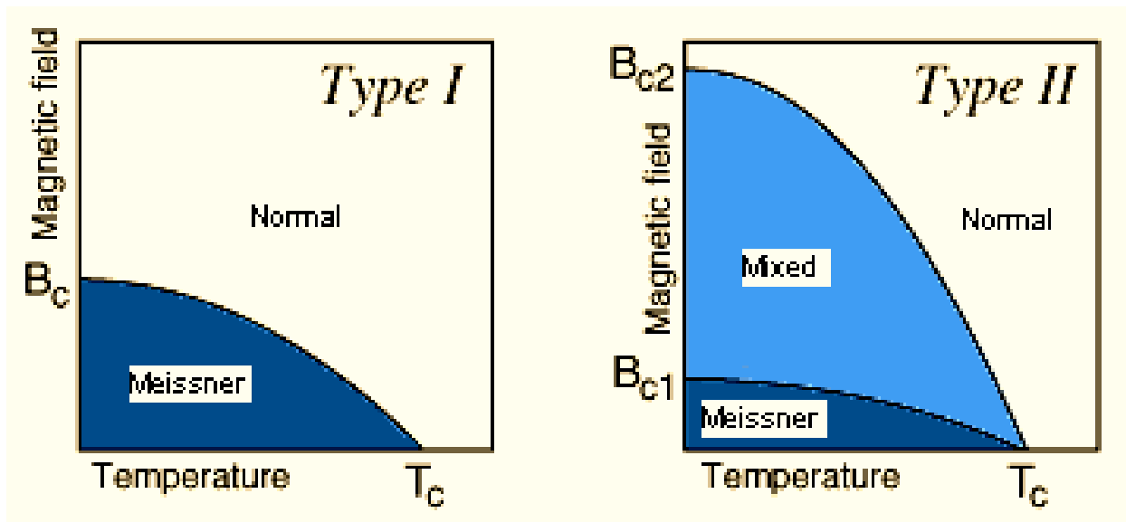
Figure 5: Phase diagram of type I and type II superconductors. Ref: Hays, Aryn M.; Bechtel, Lindsay; Turbeville, Colton; Johnsen, Anthony; and Tanner, Chris A. (2013) "Electrical and Magnetic Properties of High Temperature Superconductors Using Varying forms of Data Acquisition," Journal of the Advanced Undergraduate Physics Laboratory Investigation : Vol. 1: Iss. 1, Article 3.
