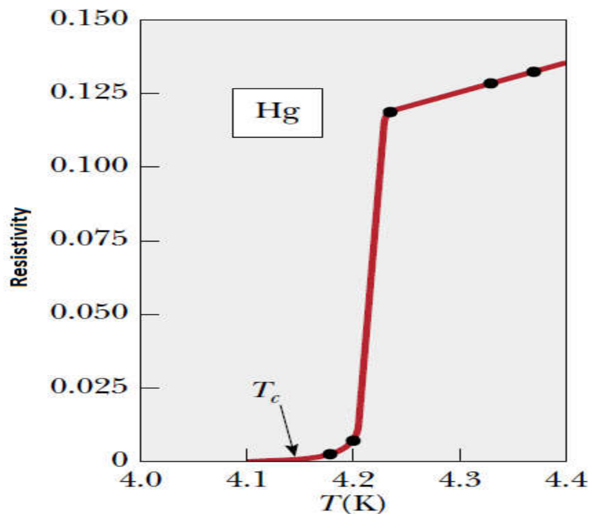
Figure 3: Plot of resistance versus temperature for a mercury. Note that the resistance of mercury follows the path of a normal metal above the critical temperature, T_c , and then suddenly drops to zero at the critical temperature, which is 4.15 K for mercury. Ref: Raymond Serway modern physics chapter 12_page486
