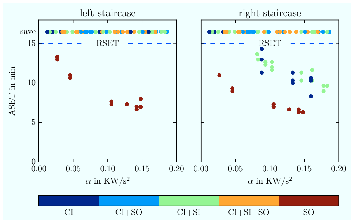
Figure 3: Correlation plots for the ASET as a function of the fire growth \alpha and the smoke extraction strategy for both staircases. An RSET of 15 minutes is assumed here and all scenarios with a longer ASET are marked as save. Color figures available in online version.
