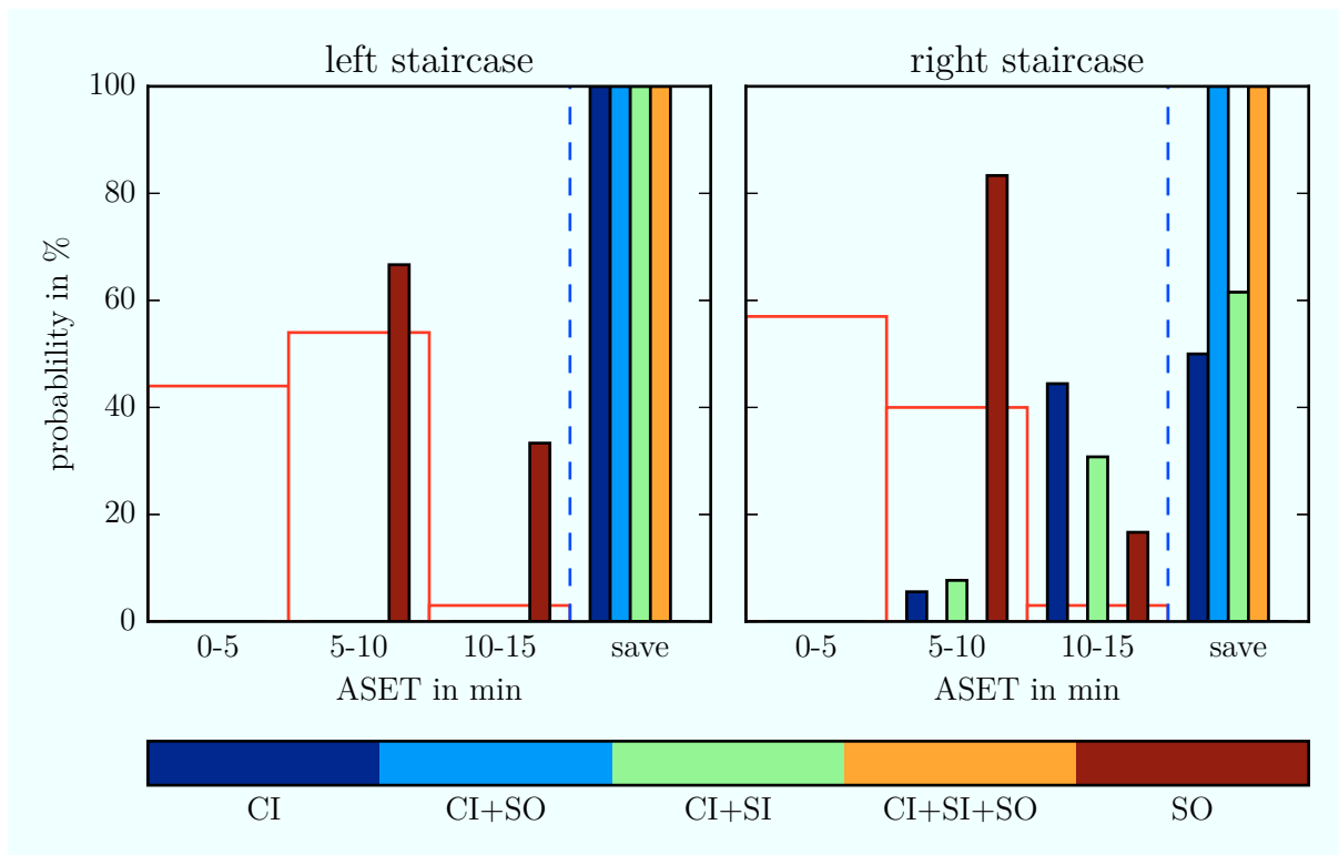
Figure 4: Probability of an extraction strategy to achieve a ASET range for each staircases. The red bars in the background indicate the according probabilities for an unventilated case, which never satisfies a save condition. Color figures available in online version.
