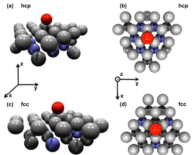
FIG. 2. Atomic structures of Fe impurity adsorbed on an hcp site [(a) side view and (b) top view] or an fcc site [(c) side view and (d) top view] of a Pt(111) surface. Pt atoms (blue) are the switching atoms, which make a large contribution to the MAE.
