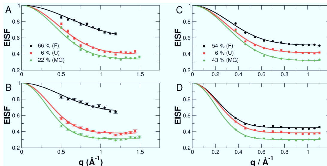
Fig. 7 EISF determined on (A) and (B) IRIS, (C) and (D) IN5. The sample temperatures are (A) 284 K, (B) 320 K, (C) 283 K and (D) 313 K. The \alpha -helical content of the native folded (F), partially folded molten globule (MG), and unfolded (U) states is given in the legend.
