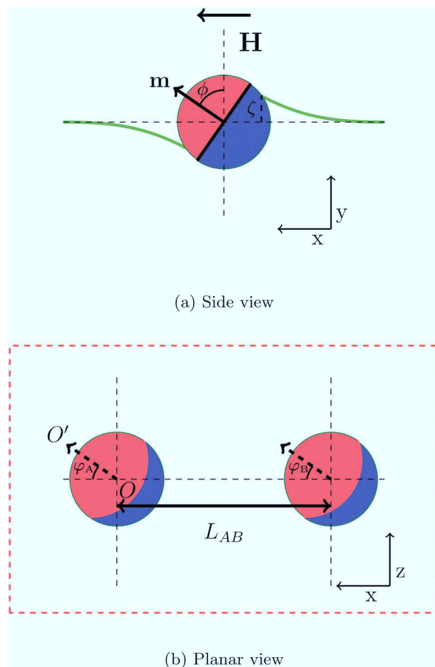
Fig. 1 (a) Side view of a single particle and (b) planar view of both particles. The Janus particle consists of an apolar and a polar hemisphere. The particle's magnetic dipole moment m is orthogonal to the Janus boundary, and the external magnetic field, H , is directed parallel to the interface. The tilt angle \phi is defined as the angle between the particle's dipole moment and the undeformed interface normal. The bold green line represents the deformed interface and \zeta is the maximal interface height at the contact line. The bond angle \varphi = \varphi_A = \varphi_B is defined as the angle between the projection of orientation of magnetic dipole on the undeformed interface (arrow OO' ) and center-to-center vector of particles. L_{AB} is pair separation.
