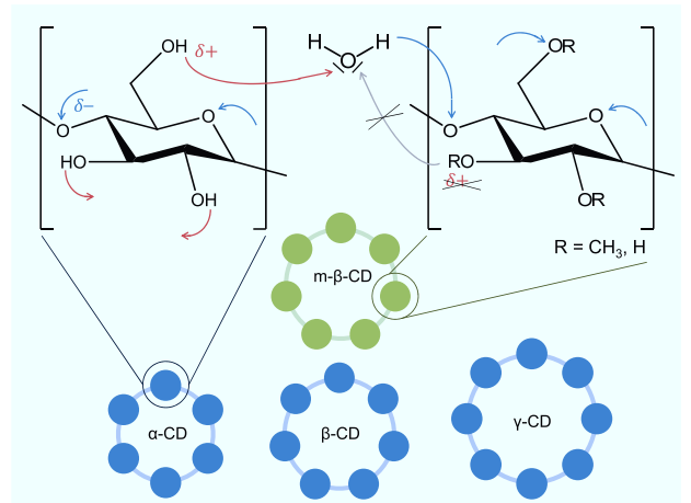
Fig. 2. Sketch of the investigated cyclodextrins and chemical structure of unmethylated (left) and methylated (right) glycopyranose units. Red and blue arrows show hydrogen bond donor and acceptor sites, respectively. In methyl- \beta -CD 55% of the hydroxyl-H are substituted with methyl group. These sites will not form hydrogen bonds (grey arrow). Further explanations are in the text.
