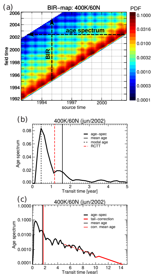
Figure 3. (a) BIR map from CLaMS pulse tracers at 400 K and 60^\circ N, plotted only for part of the full simulation period. Arrows highlight vertical and horizontal cuts through the BIR map representing BIR (vertical) and age spectrum (horizontal), respectively (cf. Haine et al., 2008). (b) The age spectrum for June 2002, corresponding to the horizontal cut in (a). Vertical lines show mean age (solid), modal age (black dashed), and the residual circulation transit time (red dashed, see text). (c) Same as (b), but including a correction for the finite spectrum tail using an exponential fit (see text). The red vertical line shows mean age for the tail-corrected spectrum, the black line for the uncorrected case (note the larger transit time range and logarithmic y axis).
