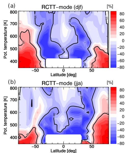
Figure 11. Difference between RCTT and modal age (RCTT - \text{mode})/RCTT in percent for (a) December–February, and (b) June–August. The black line highlights the 30% contour. The tropical lowest stratosphere (below 420 K) is left white as relative differences become arbitrarily large there due to small transit times.
