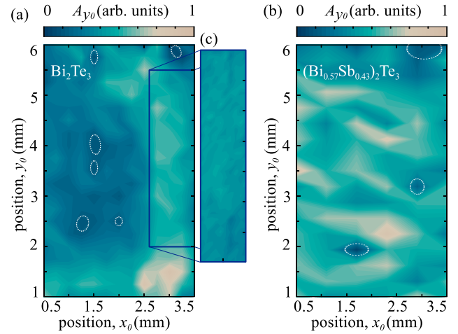
FIG. 4. Colour-coded photocurrent amplitude A_{y_0} as a function of coordinate, obtained for f=28\text{ THz} and beam spot of about 30\text{ }\mu\text{m} by a two-dimensional scan in two samples (a) \text{Bi}_2\text{Te}_3 and (b) (\text{Bi}_{0.57}\text{Sb}_{0.43})_2\text{Te}_3 . The scans are obtained in a rough scan mode with steps of 250\text{ }\mu\text{m} . Areas with vanishingly small photocurrent signals are indicated by white circles. Panel (c) shows the fine scan image obtained with steps of 100\text{ }\mu\text{m} . All data are obtained at room temperature.
