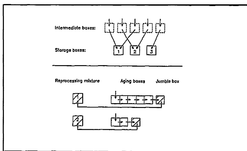
Fig. 6: Out of Pile Fuel Positions
