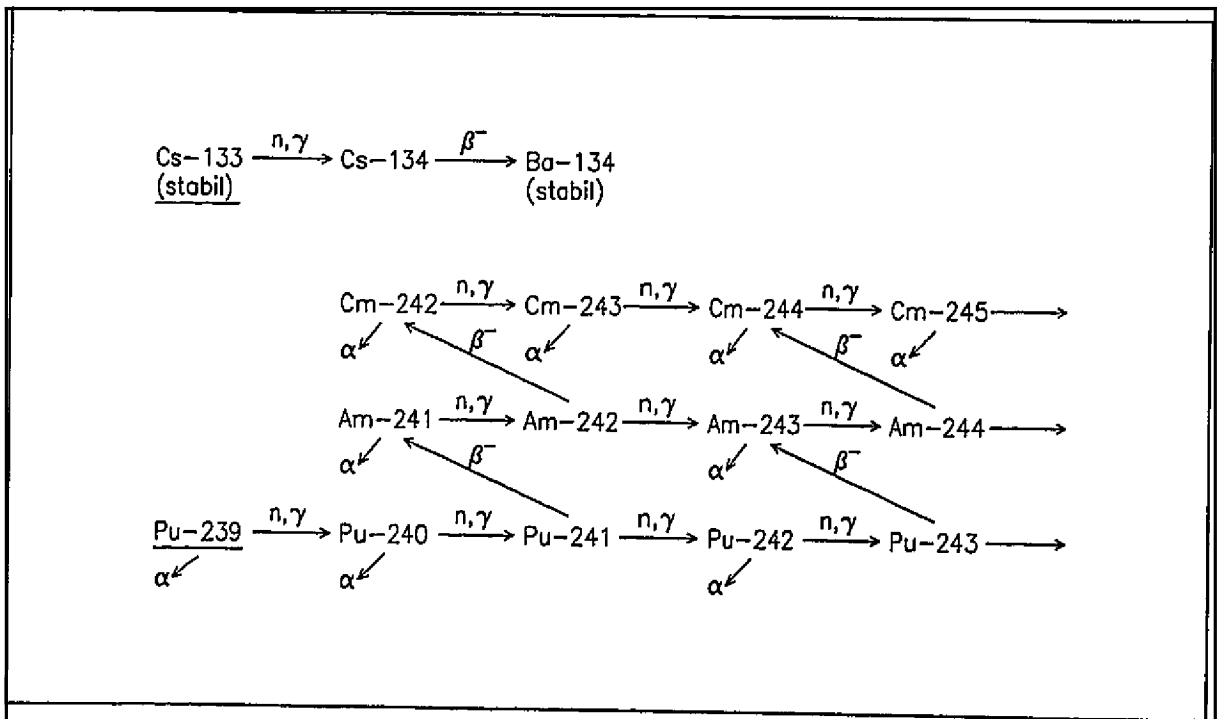
Fig. 11: Neutron Capture in Fission Products and in Actinides
