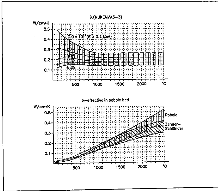
Fig.10: Thermal Conductivity
