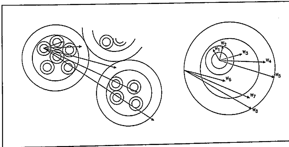
Fig. 4: Break Down of the Neutron Escape Probability.
