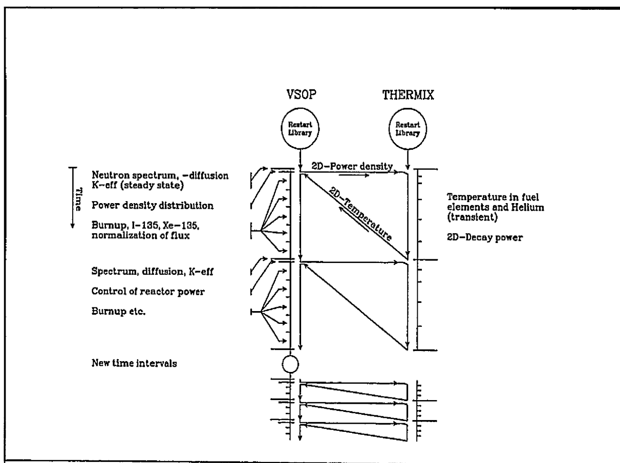
Fig. 8: Coupling between Neutronics and Thermal Hydraulics
