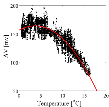
Figure 5. Second-order polynomial function fitted to the relationship between soil temperature and the difference between the first and second voltage measurements.
