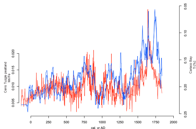
Figure 5. Comparison of the Mn / Fe ratio sequence of the CTP data set with reversed Ti values (Haug et al., 2001) at cross-correlation values > 95 % CI at a lag of 174 years, showing a correlation of r = 0.50 .
