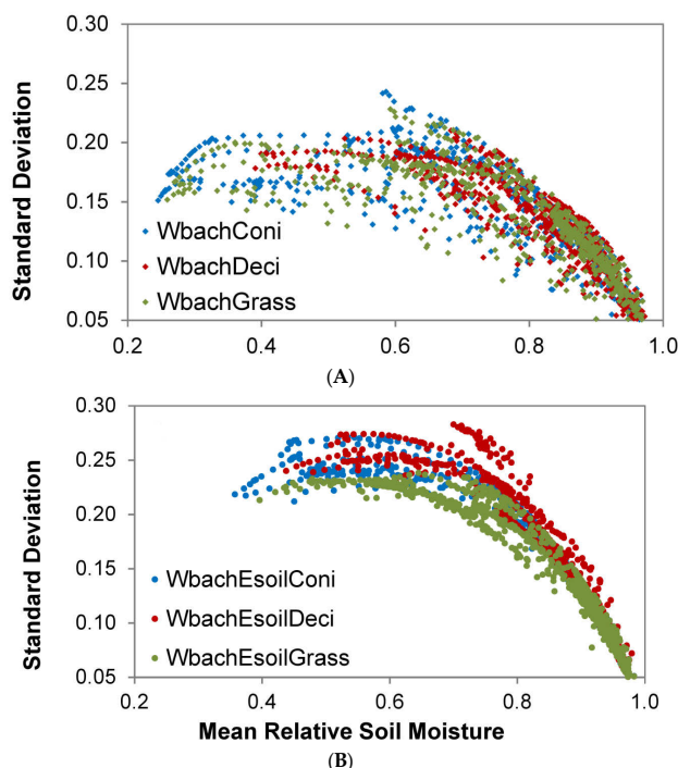
Figure 5. Relationship between mean soil moisture and its standard deviation for Wüstebach simulations at 5 cm depth with (A) Wüstebach and (B) Erkersruhr soil data.
