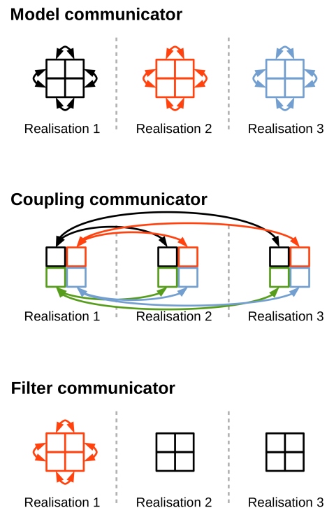
Figure 2. Communicators in PDAF for a parallel set-up with three ensemble members and four processors per ensemble member. Colours indicate the membership of the respective processors and arrows exemplify the parallel communication between the different processors.
