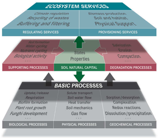
Fig. 1. Link between soil processes, soil natural capital and ecosystem services from a soil modeling perspective (adapted after Dominati et al., 2010). The gray arrows indicate the controls exerted by the soil processes on the supporting and degrading processes. The red arrows show the control of supporting and degrading processes on inherent soil processes, which in turn affect key soil processes. The green arrow indicates the impact of the soil natural capital on regulating and provisioning ecosystem services. The dots indicate that this list is not exhaustive.
