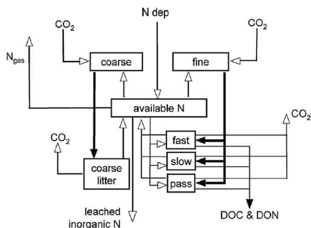
Fig. 2. Schematic diagram of N14C, showing carbon (black arrows) and nitrogen (white arrows) stocks and flows in soil and vegetation. Plants are considered to consist of two types of material, coarse or fine; soil organic matter is considered to consist of three pools with first-order rate constants of 0.25 \text{ yr}^{-1} (fast), 0.025 \text{ yr}^{-1} (slow), or 0.0005 \text{ yr}^{-1} (passive). From N14C (Tipping et al., 2012).
