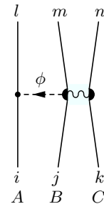
FIG. 2. Generic one-meson exchange diagram. The wiggly line symbolized the four-baryon contact vertex, to illustrate the baryon bilinears.
