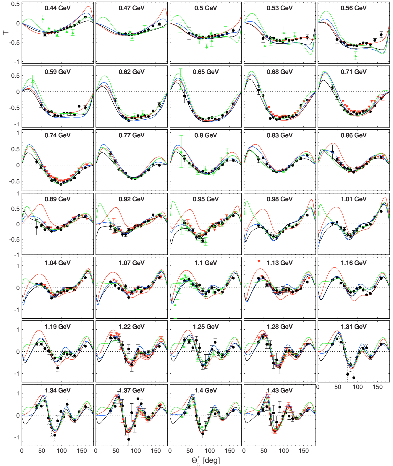
FIG. 6. Target asymmetry T . Our experimental data shown by the filled circles are compared to older data (green triangles) from [20] as well to the latest CBELSA/TAPS data [4] (red triangles). Theoretical predictions of MAID 2007 [21], SAID PR15 [2,22], BG2014-2 [23], and JuBo2015-B [25] models are shown by the red, blue, black, and green lines, respectively. The energy label in each panel indicates the central photon energy for each energy bin. Only statistical uncertainties are given for all data points.
