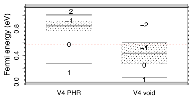
FIG. 16. (Color online) Levels of V_{4,\text{hex}} (stable) and V_{4,\text{void}} (A3). Dilute limit. Boxes indicate the inaccuracy of level determination.
