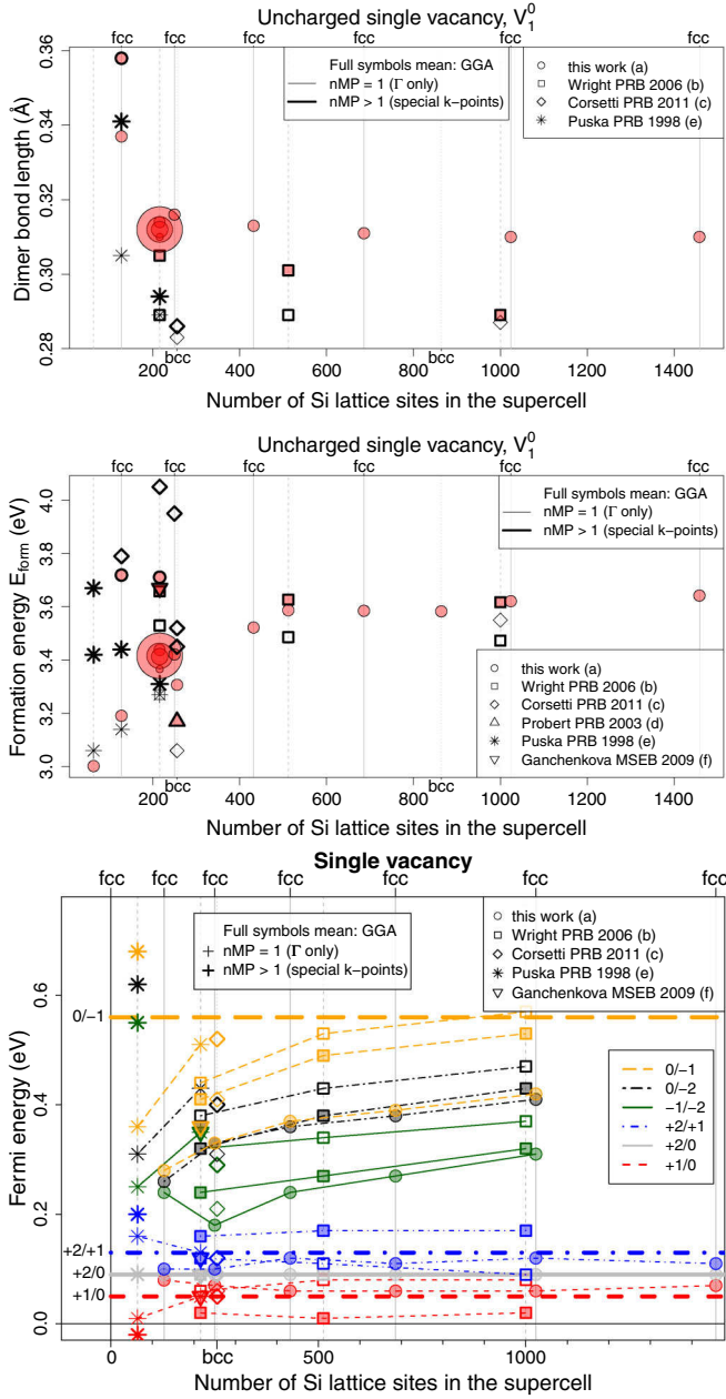
FIG. 4. (Color online) Dependence of various vacancy parameters on the cell size, the basis set (8–20 Ry for sc cell with 216 sites; circle size reflects the basis set size), Bravis superlattice (sc, fcc, bcc), and BZ sampling ( \Gamma , 2^3 MP), and comparison to literature. (a) V_1^0 dimer length. (b) E_{\text{form}}(V_1^0) . (c) Gap levels, aligned as in Table III. References: b, [28]; c, [30]; d, [24]; e, [21]; f, [29].
