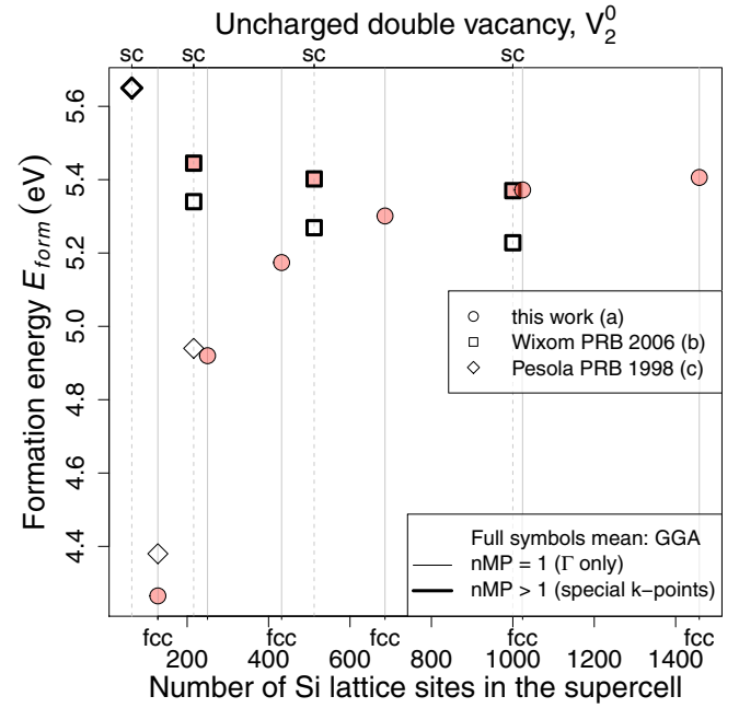
FIG. 6. (Color online) E_{\text{form}} of uncharged V_2 , compared to Refs. [53] (labeled b) and [51] (labeled c).
