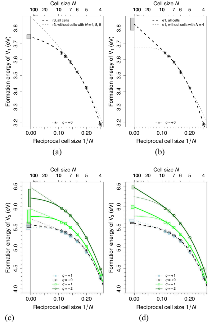
FIG. 13. (Color online) Extrapolated E_{\text{form}} . Boxes are the standard errors of the best fits. (a) The r3 and (b) the e1 models, applied to V_1^0 for all cells and with some cell sizes ignored. E_{\text{form}}(V_2^q) at E_F = E_{\text{VBM}}^{\text{GGA}} for the two best (c) four-parameter and (d) three-parameter models.
