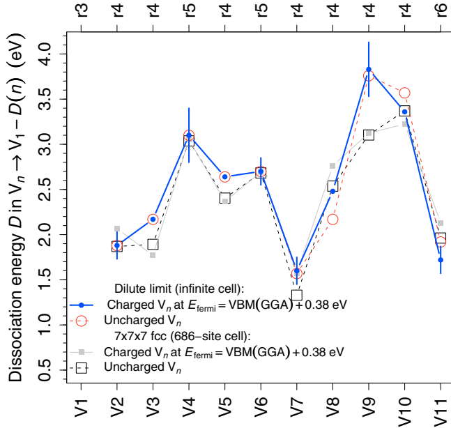
FIG. 15. (Color online) V dissociation energies computed with the 7 \times 7 \times 7 cell (686 sites) and extrapolated to infinite supercells by the best \Gamma model [Eq. (9)] for each defect. See Table VIII.
