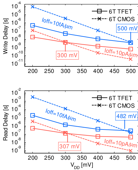
FIGURE 9. Comparison of write and read delays as a function of V_{DD} of the 6T O-AT TFET and 6T CMOS cells implemented with devices whose I_{OFF} was aligned at either 10 pA/μm or 10 fA/μm (Fig. 3).
