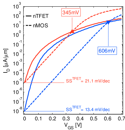
FIGURE 3. I_D – V_{GS} characteristics of the n-type TFET and MOSFET aligned at I_{OFF} = 10 pA/ \mu m and at I_{OFF} = 10 fA/ \mu m. V_{DS} = 0.5 V.
