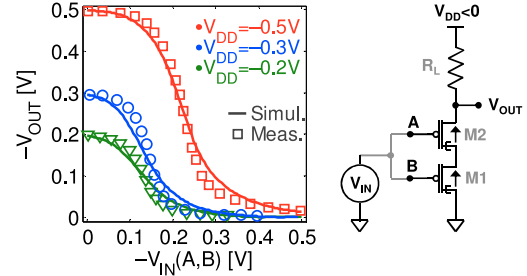
FIGURE 14. Measured [22] and simulated VTCs of a p-NAND logic gate (the two inputs A and B are tied together). R_L = 500 k \Omega (2 M \Omega ) for the VTC traced with V_{DD} = -0.5 V (-0.3 V and -0.2 V).
