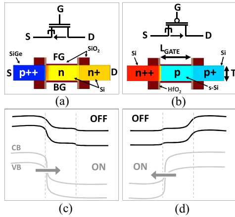
FIGURE 1. Symbols and structures of (a) SiGe/Si/Si NTFET and (b) Si/strained-Si/Si PTFET. L_{\text{GATE}} = 30 nm, T = 10 nm, EOT = 1.1 nm. Details of the device design are provided in [4]. Sketches of band diagrams along the device in both OFF and ON states for (c) NTFET and (d) PTFET.
