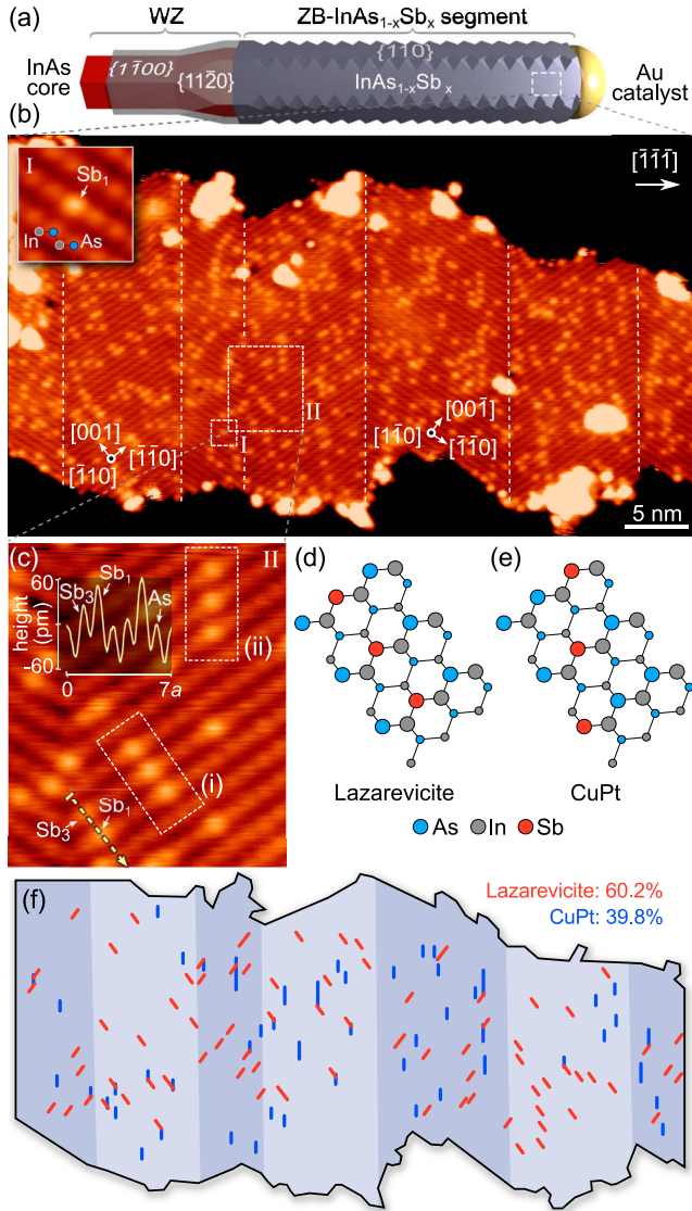
FIG. 1. (a) Schematic of a [1\bar{1}\bar{1}] grown \text{InAs}_{0.90}\text{Sb}_{0.10}/\text{InAs} nanowire. (b) Atomically resolved constant-current STM image of the sidewall surface measured at 77 K ( -3 V sample voltage and 10 pA tunnel current). The image shows the filled dangling bond states above the surface anions. The bright atomically localized contrast features arise from Sb atoms incorporated on anion sites. Twin boundaries are marked by dashed vertical lines. The inset [marked I in (b)]: high-resolution STM image ( -2 V, 700 pA) of one \text{Sb}_{\text{As}} atom in the surface layer. The location of the atomic zigzag chain of alternating anion and cations is indicated by a ball model. (c) High-resolution STM image ( -2 V, 700 pA) of area II in (b). Sb atoms in the first layer ( \text{Sb}_1 ) and third layer ( \text{Sb}_3 ) are visible. Local lazarecivite- [12] and CuPt-type ordered areas are labeled (i) and (ii), respectively. (d) and (e) illustrate the respective atomic models. (f) Spatial distribution of CuPt (blue) and lazarecivite (red) SROs.
