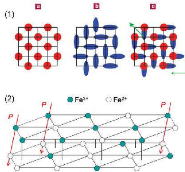
Figure 1.9: Schematic diagram of (1) (a) site-centered and (b) bond-centered charge order (b) intermediate ferroelectric state (lack of inversion symmetry) due to the presence of both site and bond centered charge order simultaneous. Arrow indicate the resulting polarization, taken from reference [63]. (2) View of proposed charge redistribution within bilayer of the \text{FeO}_2 triangular lattices in \text{LuFe}_2\text{O}_4 . The interlayer charge-ordering inducing electric polarization is indicated by red arrow, taken from reference [62].
