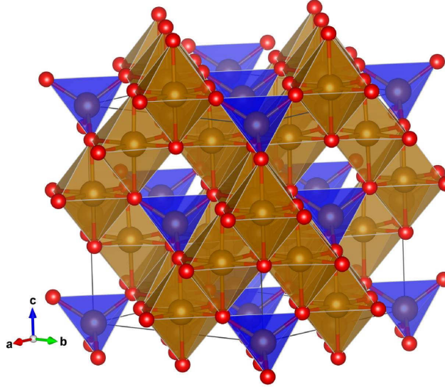
Figure 4.1: Room temperature structure of Magnetite
