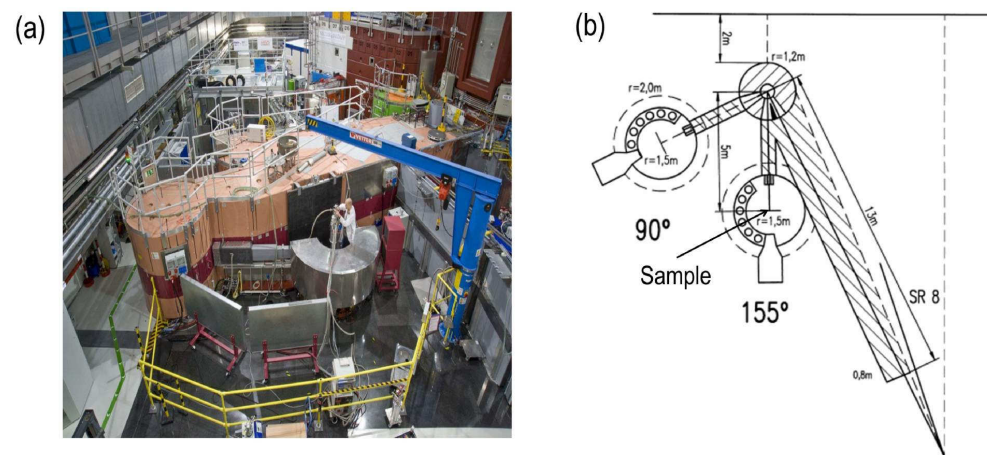
Figure 2.12: (a) The instrument SPODI, taken from reference [88] and (b) its schematic sketch taken from reference [87]. 90^\circ and (mainly used) 155^\circ are monochromatic angles.
