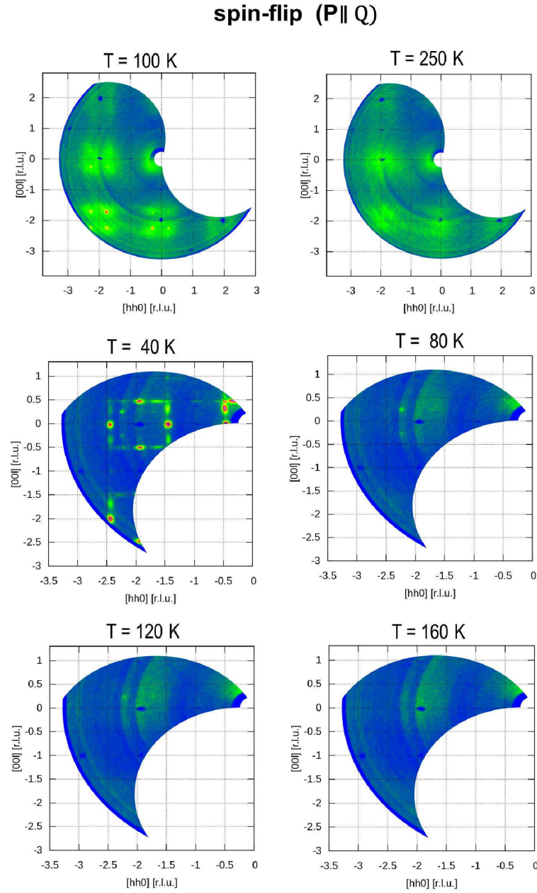
Figure 6.20: Scattered intensity in spin-flip channel with P \parallel x i.e., approximately \parallel to Q , measured in hhl - plane at different temperatures.
