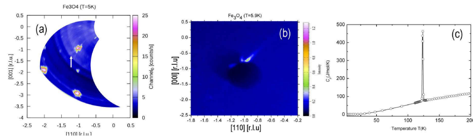
Figure 4.15: (a) Neutron Diffuse neutron scattering in (hhl) plane at 5 K (b) Diffuse scattering by high energy X-rays in (hhl) plane at 6 K. (c) Specific heat, C_P of the crystal measured at zero magnetic field ( T_V=123\text{ K} ).
