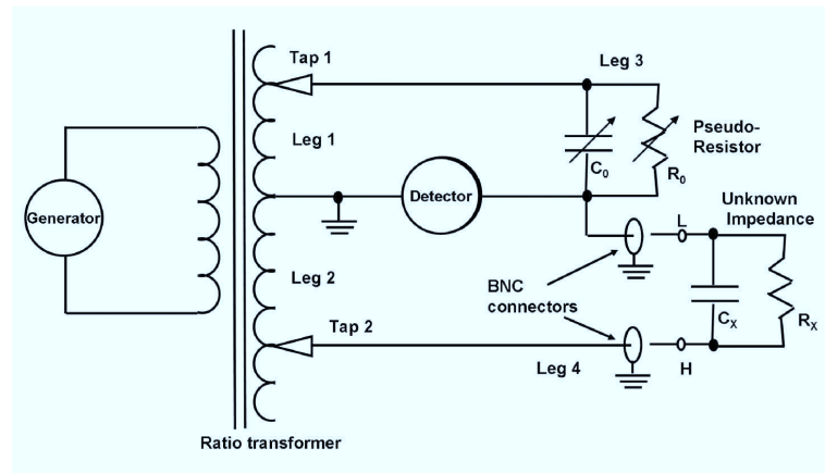
Figure 3.4: AH2700A basic bridge circuit.
