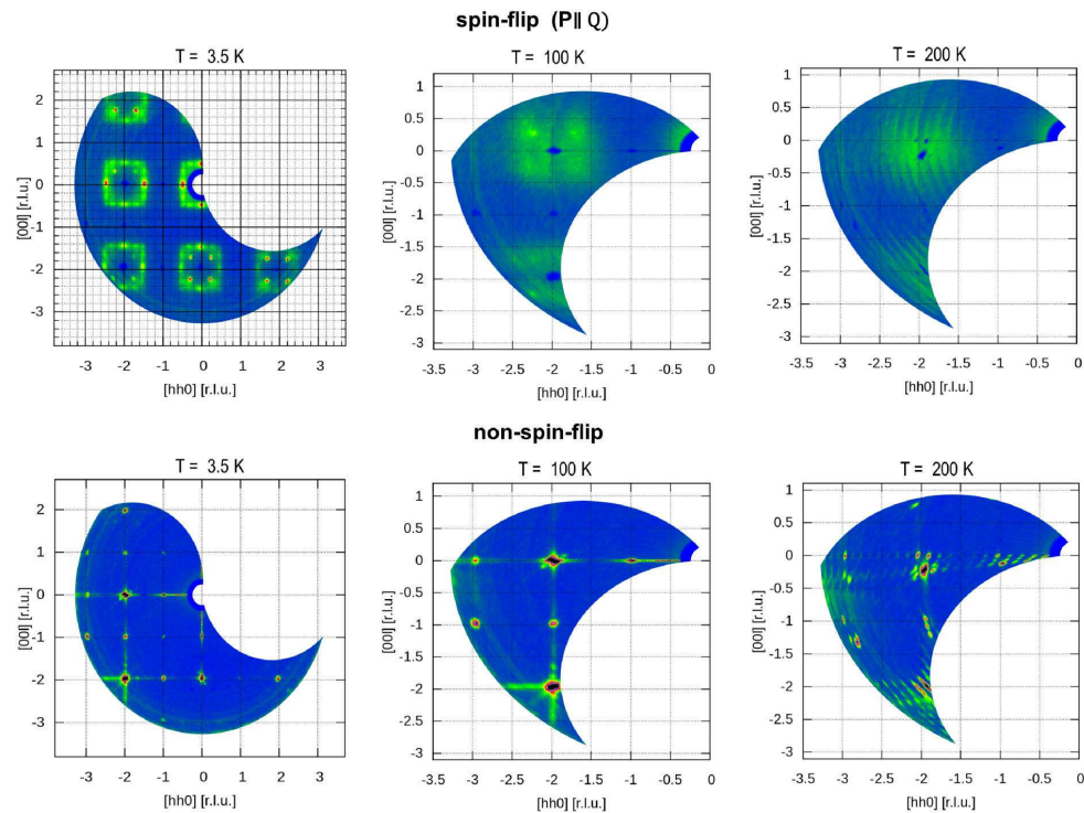
Figure 6.25: Polarization analysis with P \parallel Q , measured in hhl - plane at 3.5 K, 100 K and 200 K. Upper panel represents hhl -plane in spin-flip channel and the lower panel represents hhl -plane in non-spin-flip channel.
