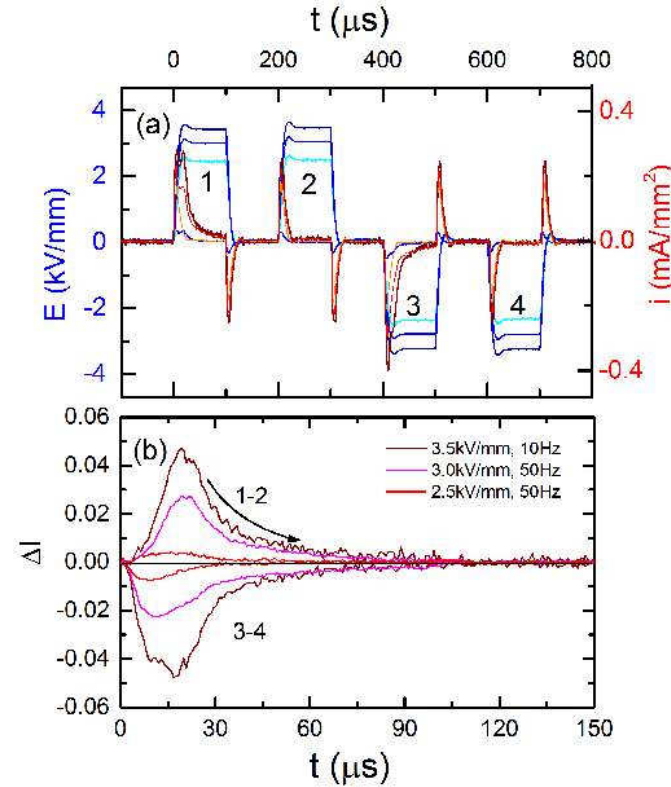
Figure 5.4: (a) Result of PUND measurement on a high quality magnetite single crystal at T = 5 K. The delay time between pulses was 100\mu\text{s} . (b) Difference between the measured currents for the 1st and 2nd, as well as 3rd and 4th pulses.
