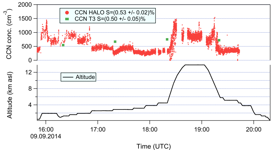
FIG. 15. Time series plot of CCN concentrations and altitude during flight AC08. The green markers represent the CCN measurements performed at the T3 measurement site near Manacapuru. Particle number concentrations have been normalized to standard air pressure (1000 hPa) and temperature (273.15 K).
