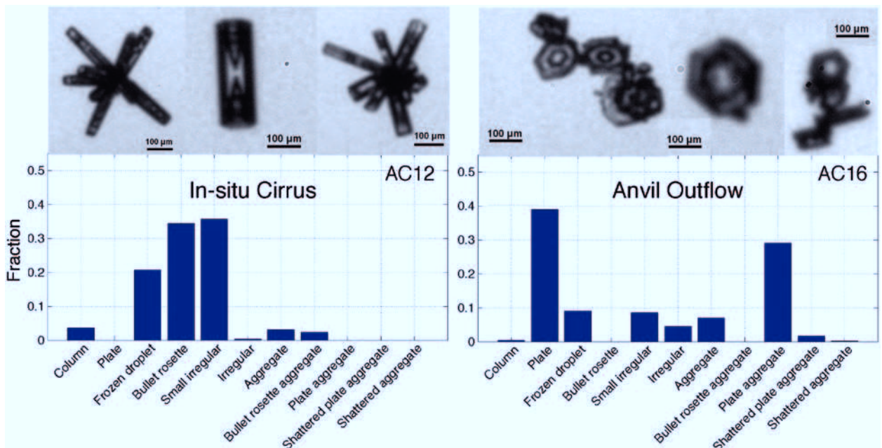
FIG. 14. Statistical analysis of the ice microphysical properties of ambient in situ cirrus sampled during flight AC12 and of an anvil outflow of a tropical convective system sampled during flight AC16. The analysis is based on stereoscopic images taken by the PHIPS-HALO probe, which was newly developed for HALO.
