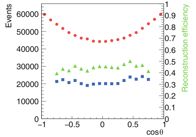
Fig. 13. Angular distribution for \bar{p}p \rightarrow e^+e^- at p_{lab} = 3.3 GeV/c of generated (red circles) and reconstructed and identified (blue squares) electrons. The reconstruction efficiency (green triangles) corresponds to the y -axis scale on the right.
