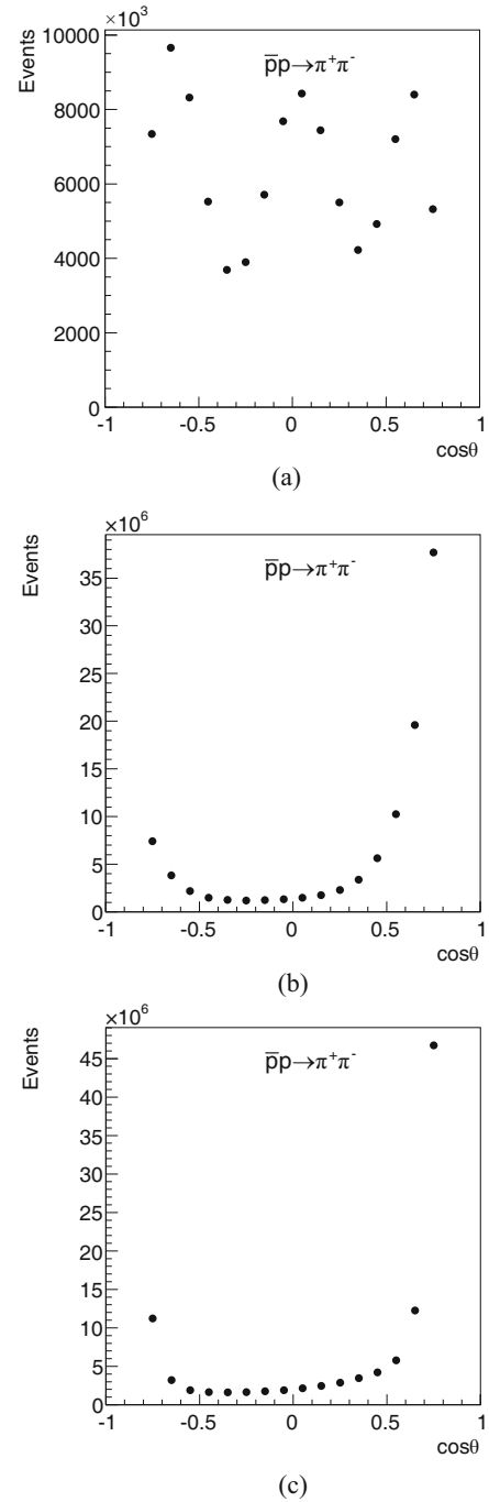
Fig. 7. Angular distribution of \pi^- from the \bar{p}p \rightarrow \pi^+\pi^- events generated using the model from ref. [46] for different p_{lab} values: (a) 1.7 GeV/c, (b) 3.3 GeV/c, and (c) 6.4 GeV/c.
