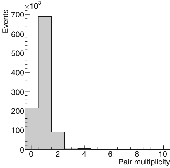
Fig. 12. Multiplicity distribution of the number of reconstructed pairs of particles. 10^6 signal events were generated at a beam momentum of p_{lab} = 3.3 GeV/c.
