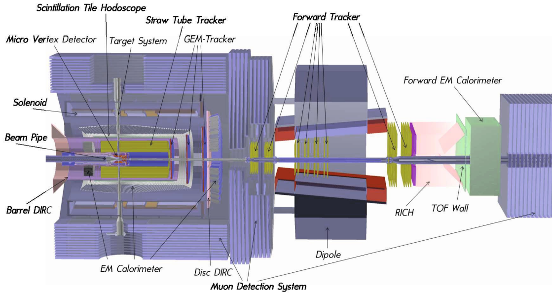
Fig. 5. View of the \bar{\text{P}}\text{ANDA} detector.
