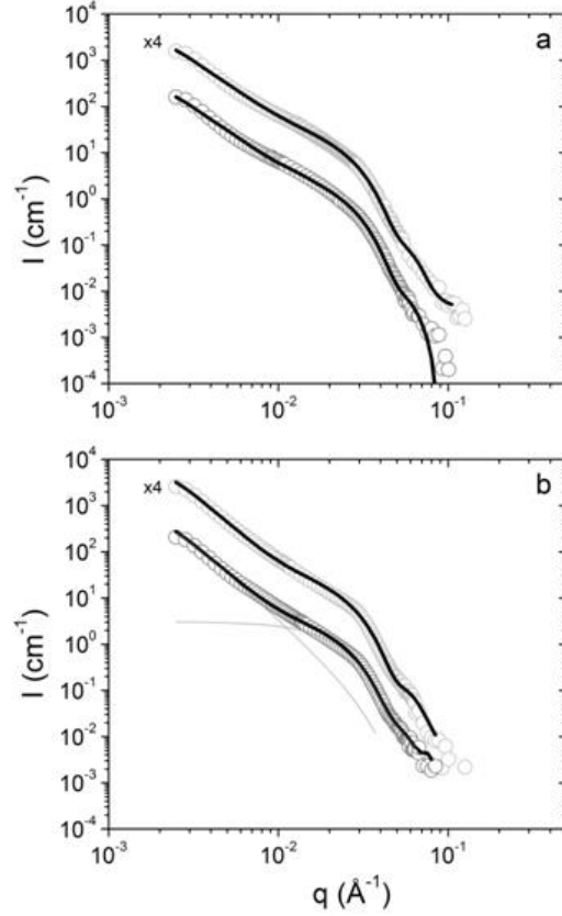
Figure 3: SANS profiles from PnBA-b-PAA-1 aqueous solutions 1 ( \circ ) and 3 ( \odot ) mg/ml at pH7, 0.01M NaCl (a) and 0.15M NaCl (b). Continuous lines are fits to the experimental data. The separate contributions of micelles and aggregates are shown in b.
