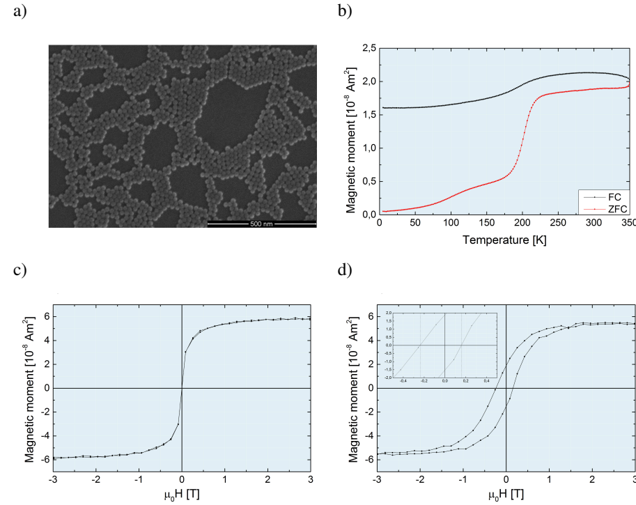
Figure 4.11: Sample 3-02: a) SEM image b) ZFC (red) and FC (black) curve measured at \mu_0 H = 0.005 \text{ T} exhibiting a metastable state during the phase transformation of wustite to maghemite c) Hysteresis loop at 300 K and d) 5 K showing superparamagnetic behavior and exchange bias.
