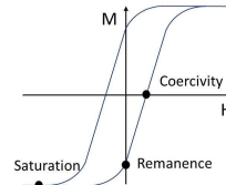
Figure 3.7: Characteristics of a typical major hysteresis loop.
