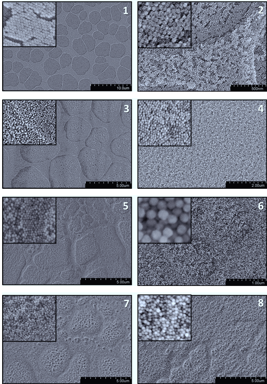
Figure 5.36: SEM images of the sample center after each preparation step consisting of nanoparticle deposition, surfactant removal and palladium deposition.
