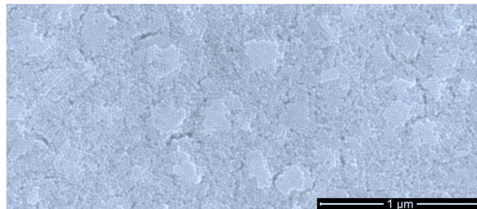
Figure 4.3: Sample 1-01: SEM image in the center of a silicon substrate on which the nanoparticles ( 9 \mu\text{l} dispersion with a concentration of 25 \text{ mg/ml} ) are deposited by spincoating (60 s at 3000 rpm).
