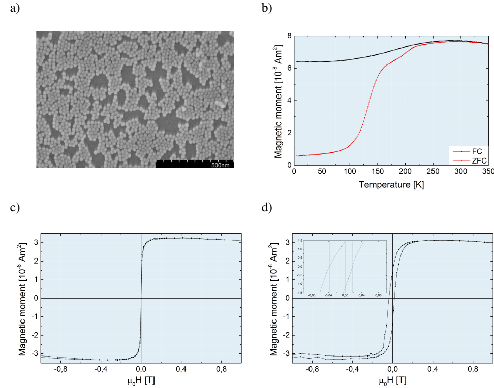
Figure 4.12: Sample 3-03: a) SEM image b) ZFC (red) and FC (black) curve measured at \mu_0 H = 0.005 T displaying a stable, partial phase transition c) Hysteresis loop at 300 K and d) 5 K exhibiting superparamagnetism and a slight exchange bias.
