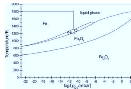
Figure 2.1: Phase diagram of the iron-oxygen system, reprinted with permission from [43].
