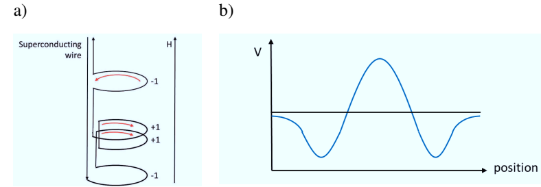
Figure 3.2: a) Pickup coil for Quantum Design MPMS systems. b) Example response curve.
