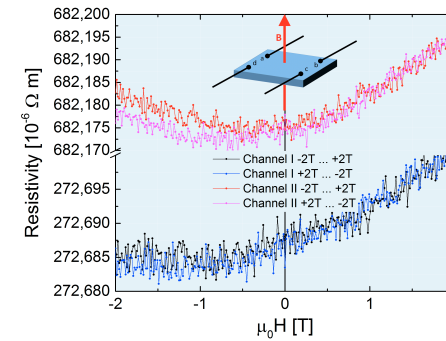
Figure 5.41: Nanoparticle/palladium multilayer: Resistivity in dependency of a magnetic field applied perpendicular to the sample plane, measured at 10 K.
