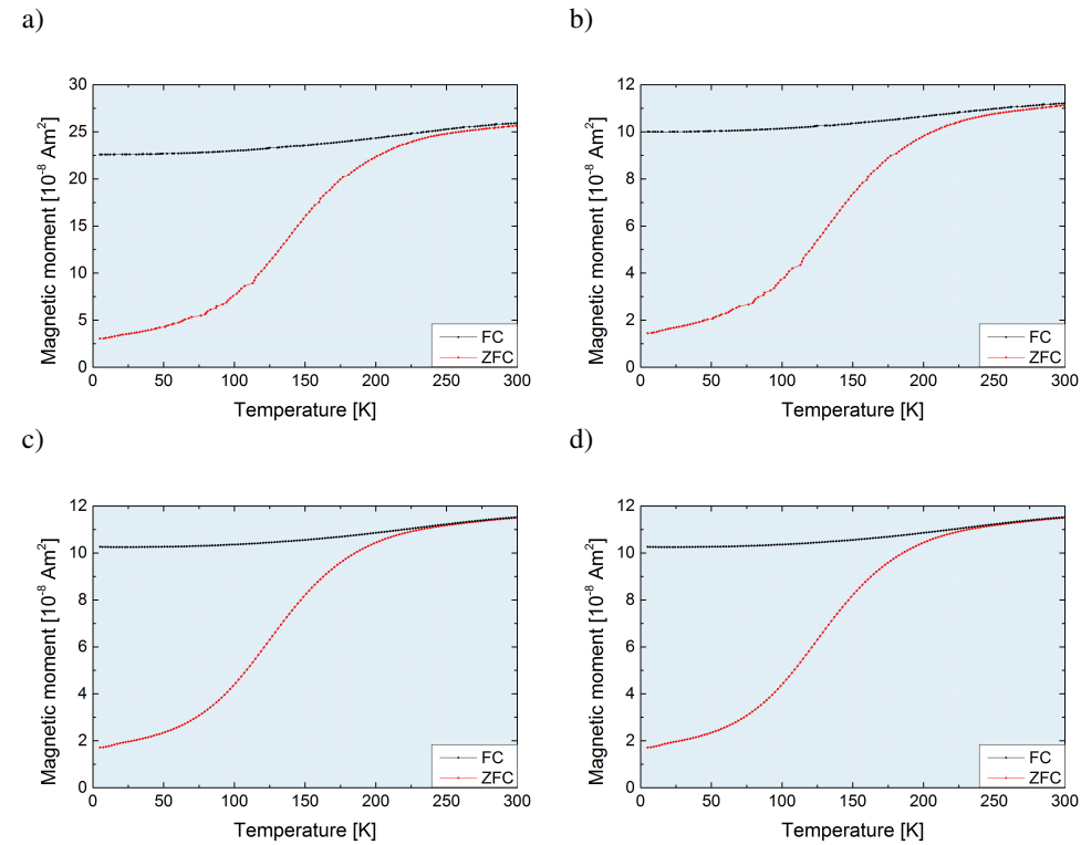
Figure 5.34: ZFC-FC measurements performed on single macrocrystals removed from samples prepared using batch O2 by centrifugation at a) 0°C at 21 000 x g, b) 20°C at 21 000 x g, c) 30°C at 21 000 x g and d) 10°C at 12 000 x g.
