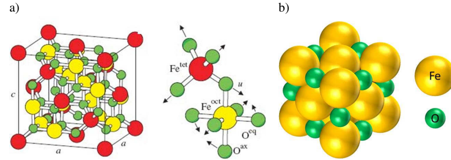
Figure 2.2: a) Inverse spinel (reprinted with permission from [48]) and b) rocksalt structure of wustite. Red and yellow spheres represent tetrahedrally and octahedrally coordinate iron ions, respectively. Green spheres are oxygen ions.
