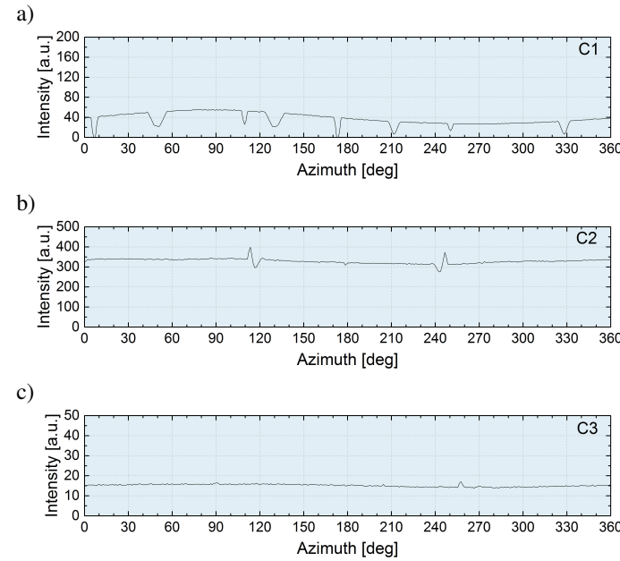
Figure 5.31: Intensities as function of the azimuthal angle integrated over a ring width of 0.04 \text{ \AA}^{-1} for the SAXS patterns shown in figure 5.32. a) Batch C1, b) batch C2, c) batch C3.
