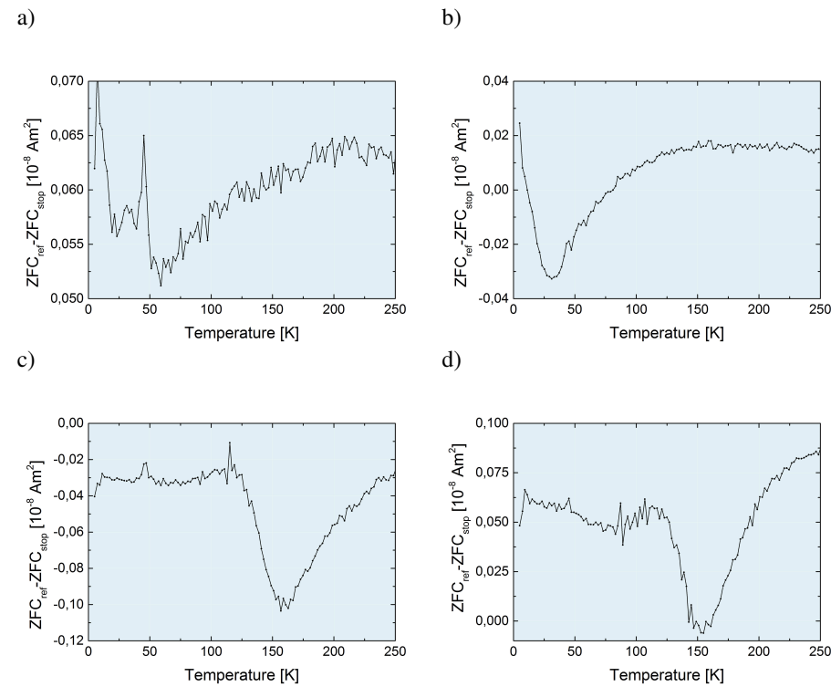
Figure 5.33: Memory effect measurements with an aging time of 10 000 s performed on single macrocrystals that were obtained after centrifugation at 10°C at 21 000 x g using a) batch C1, b) batch C2, c) batch O1 and d) batch O2. Hereby the aging stop was performed at 25 K for a) and b) or at 140 K for c) and d).
