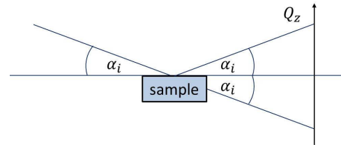
Figure 3.17: Determination of the origin of the Q_z axis using the incident beam and the specular reflection.
