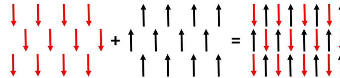
Figure 2.8: Illustration of antiferromagnetic order by two interpenetrating ferromagnetic sub-lattices.
