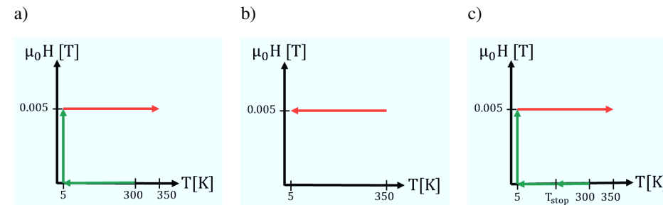
Figure 3.3: Measurement procedures for a) zero field cooling b) field cooling and c) memory effect, where red arrows mark the paths along which the magnetic moment is recorded.
