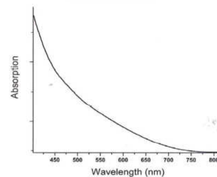
Absorption Spectra
