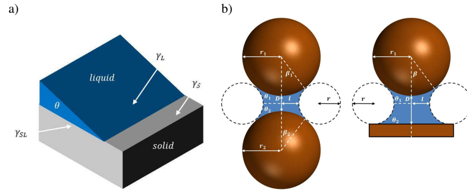
Figure 2.14: a) Illustration of the contact line for a liquid drop (blue) on a solid surface (gray) surrounded by gas. b) Meniscus formation between two bodies.
