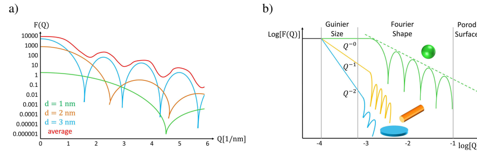
Figure 3.15: a) Form factors of three monodisperse samples (spherical nanoparticles with a diameter of 1 nm (green) / 2 nm (yellow) / 3 nm (blue)) and their sum (red) representing a polydisperse sample. b) Universal Guinier plot of the particle form factor for spherical (green), rod-like (orange) and lamellar shaped nanoparticles illustrating the domains of information, according to [118].
