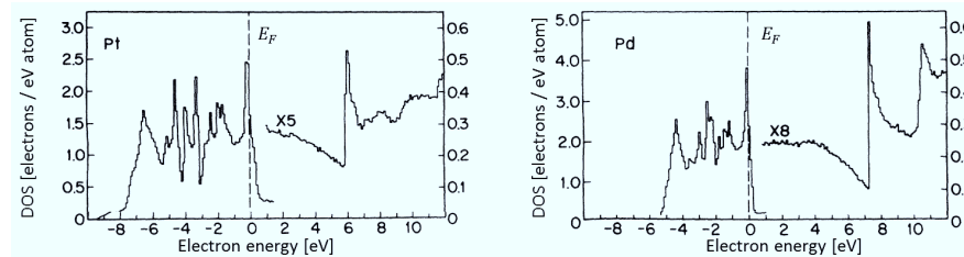
Figure 4.31: Density of states histograms for platinum and palladium, reprinted with permission from [152].
