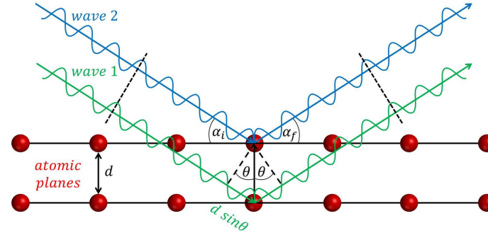
Figure 2.17: Schematic representation of Bragg's law.
