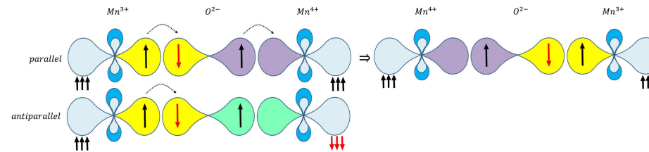
Figure 2.5: Double exchange interaction in manganese oxide: For parallel arrangement of manganese ions hopping is possible without excitation energy, according to [59].
