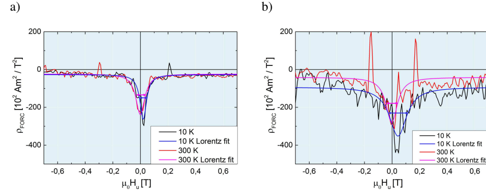
Figure 4.18: FORC density in dependency of the interaction field at zero coercive field and corresponding Lorentz fit for a) the platinum covered sample 4-01 and b) the palladium covered sample 4-02 at 300 K and 10 K, respectively. The arrows indicate the calculated FWHM.
