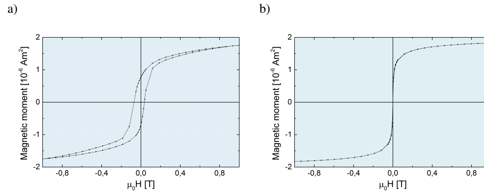
Figure 5.38: Hysteresis curves of the nanoparticle/palladium multilayer measured at a) 5 K and b) 300 K, revealing superparamagnetism and exchange bias.
