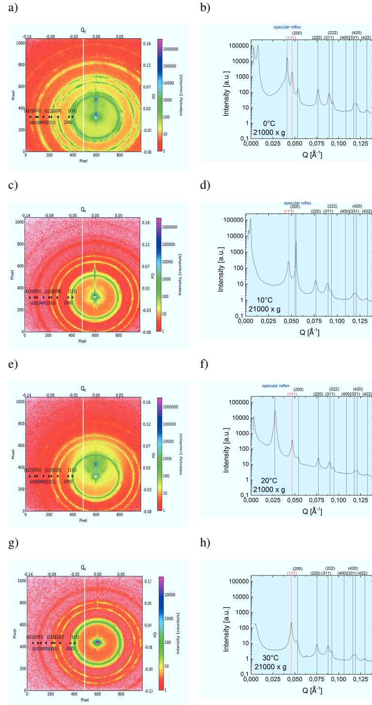
Figure 5.28: Batch O2: SAXS measurements performed on single macrocrystals removed from samples that were centrifuged at 21 000 x g (a,c,e,g) and radial integrated intensities (b,d,f,h). The measured (111) peak is labeled in red and further, calculated peak positions for a FCC lattice are shown in black. The specular reflex is highlighted in blue. The centrifugation temperature was a,b) 0°C, c,d) 10°C, e,f) 20°C, g,h) 30°C.
