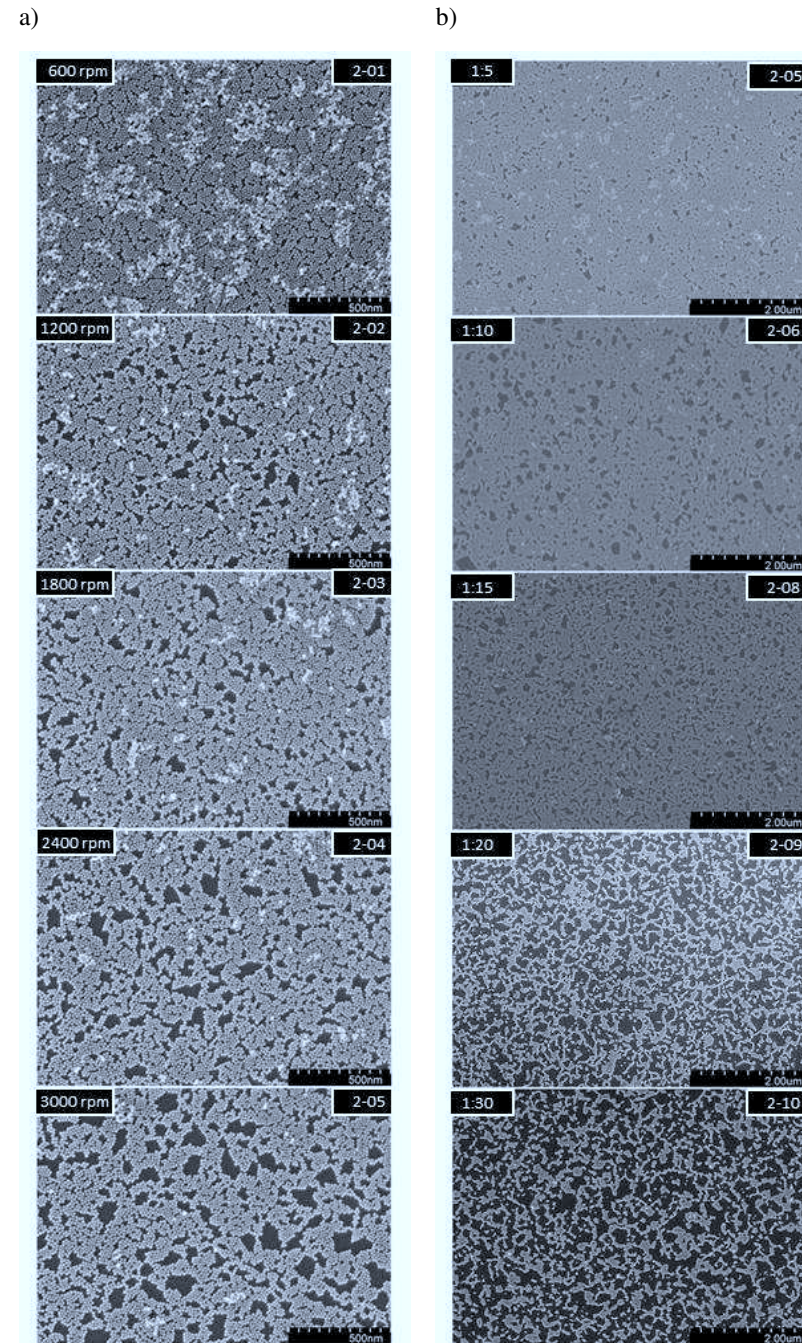
Figure 4.7: SEM images displaying the influence of variations in a) rotational speed (samples 2-01...2-05) and b) dilution with toluene (samples 2-05...2-10) for the fabrication of a (sub-) monolayer of nanoparticles by spin-coating on silicon substrates.
