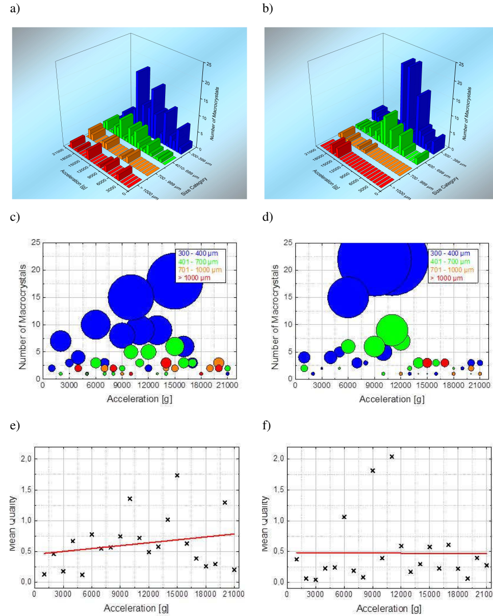
Figure 5.18: Number of macrocrystals per size category for all 21 samples centrifuged at 10°C a) without and c) with illustration of the score value S which corresponds to the dot size. e) Quality factor (black) and linear fit (red). b), d) and f) correspond to the reproduced samples.
