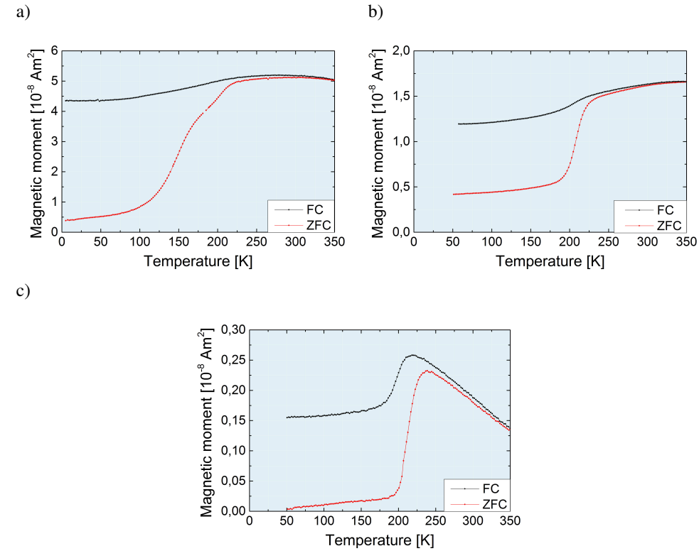
Figure 4.13: ZFC-FC curves measured at \mu_0 H = 0.005 \text{ T} showing a) the onset (sample 3-04) of phase transition after 30 s of plasma treatment and b) the longest plasma duration possible without phase transition (10 s, sample 3-05). c) Sample 3-06 reveals that hotplate treatment only has almost no influence on the magnetic behavior.
