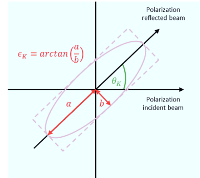
Figure 3.5: Schematic description of the Kerr rotation \theta_K and ellipticity \epsilon_K , which can be combined to the complex Kerr angle \Phi_K .
