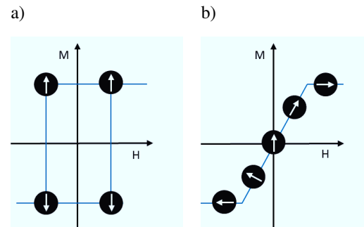
Figure 3.10: Hysterons for the theoretical behavior of an individual nanoparticle for a field applied along the a) easy or b) hard axis.
