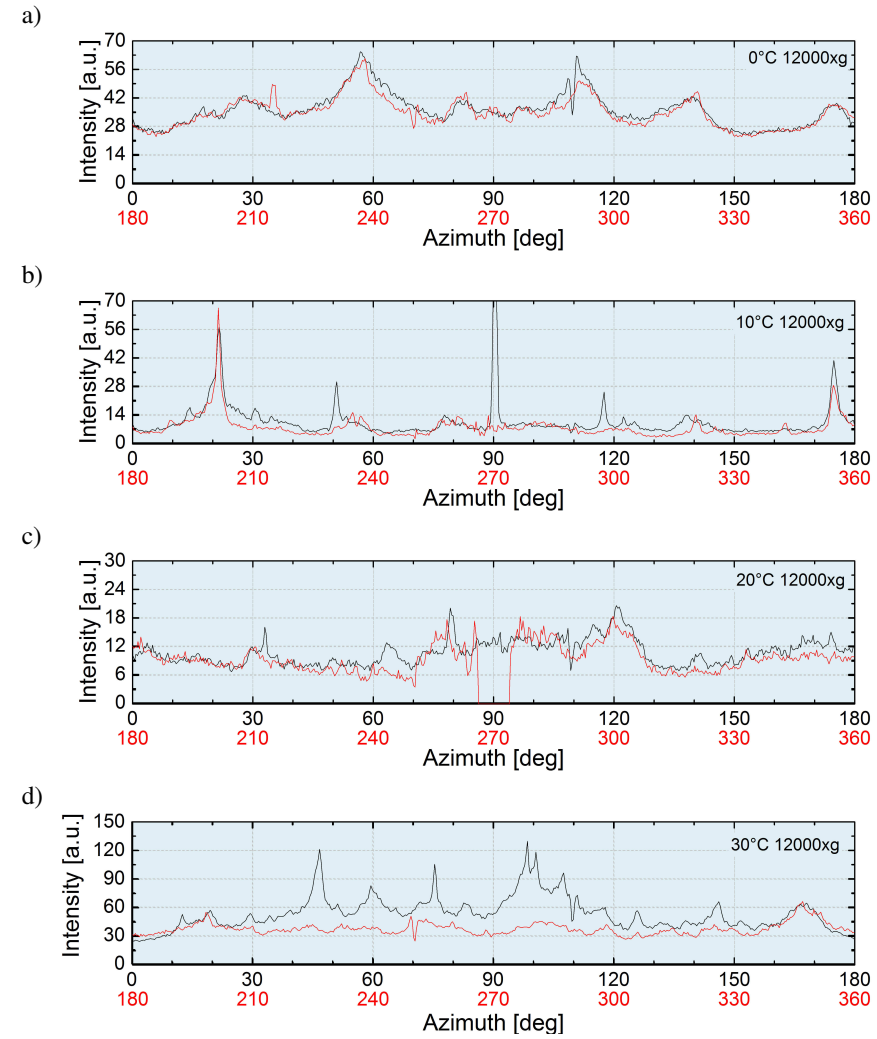
Figure 5.27: Intensities on the (220) powder ring as function of the azimuthal angle integrated over a ring width of 0.01 \text{ \AA}^{-1} for the SAXS patterns shown in figure 5.26 (batch O2).
