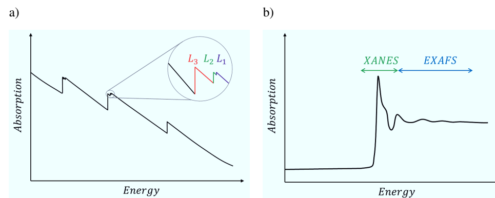
Figure 3.18: X-ray absorption spectrum: a) Complete spectrum showing three major transitions and splitting at higher resolution (inset) b) Schematic view of a single edge, according to [123].
