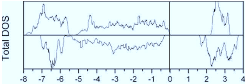
Figure 4.21: Electronic density of states for maghemite. Reprinted with permission from [149].
