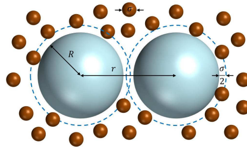
Figure 2.15: Two large spheres approaching each other and thus hindering the small ones to use the space in between. The resulting uncompensated osmotic pressure causes an attractive depletion force.
