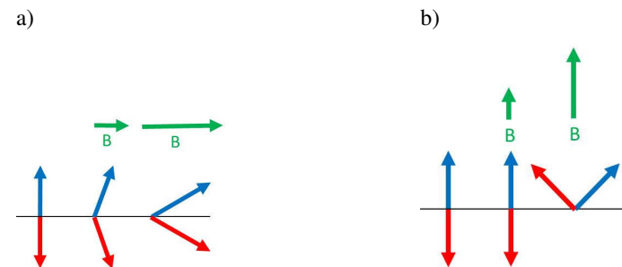
Figure 2.9: a) Antiferromagnetic spin canting if a magnetic field is applied perpendicular to the anisotropy axis. b) Spin-flop process for magnetic fields applied parallel to the anisotropy axis.
