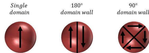
Figure 2.10: Examples for magnetization configurations in spherical ferromagnetic nanoparticles.
