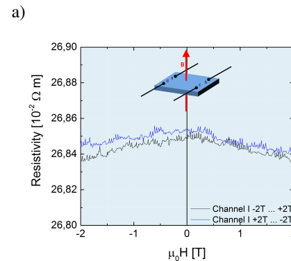
Figure 4.26: Sample 5-02 (NPs + 5 nm palladium): Resistivity measurements performed at 150 K according to the van der Pauw method with the magnetic field applied out-of-plane. The current flows between a and b (channel I).
