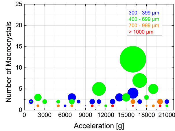
Figure 5.11: Number of macrocrystals per size category for all samples centrifuged at 0°C, where the dot diameter is proportional to the score value S.
