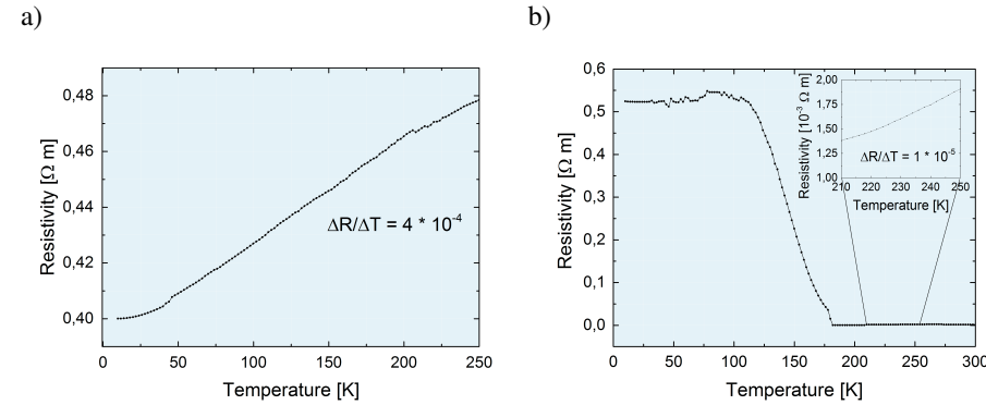
Figure 4.25: Temperature dependency of the resistivity for a) reference sample 5-01 (5 nm palladium only) and b) sample 5-02 (NPs + 5 nm palladium).
