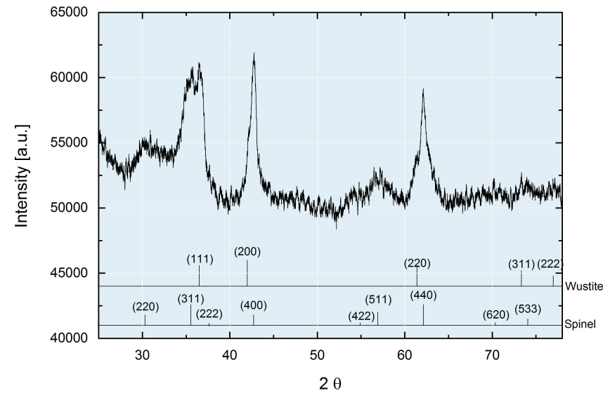
Figure 4.6: X-ray powder diffraction pattern of a nanoparticle multilayer after background subtraction revealing a mixture of wustite with a spinel (maghemite or magnetite). In the lower area of the graph the corresponding XRD patterns are indicated according to the data shown in [141].
