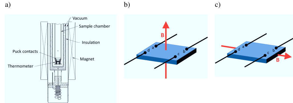
Figure 3.12: a) Schematic setup of the resistivity option of the Quantum Design PPMS system, taken from [113]. b) Sample geometry for resistivity measurements with a magnetic field applied out-of-plane or c) in-plane.
