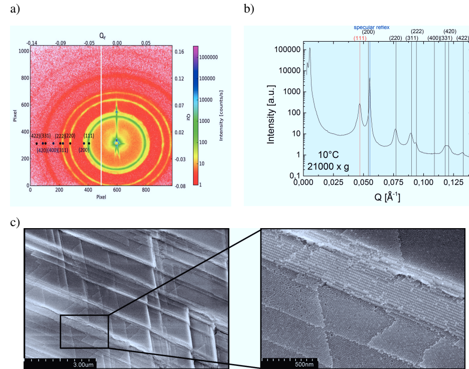
Figure 5.21: a) SAXS measurements performed on a single macrocrystal removed from the sample centrifuged at 10°C at 21 000 x g using batch O2 and b) radial integrated intensity. The measured (111) peak is labeled in red and further, calculated peak positions for a FCC lattice are shown in black. The specular reflex is highlighted in blue. c) SEM image of an FCC ordered grain at the macrocrystal surface.
