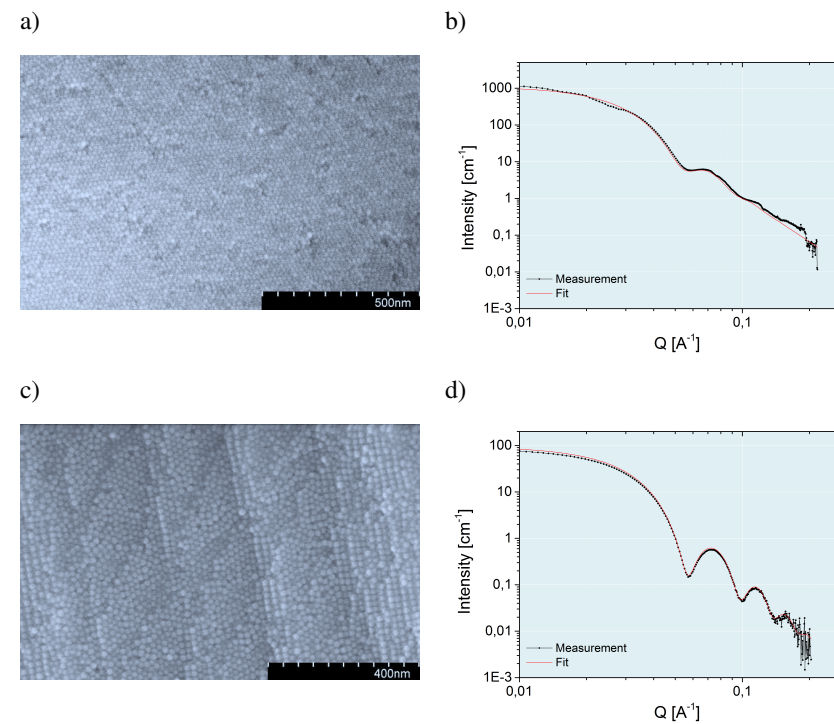
Figure 5.3: SEM images of iron oxide nanoparticles at the surface of macrocrystals for a) batch O1, c) batch O2 and Small Angle X-ray Scattering patterns of 25/30 mg NP / ml toluene dispersions obtained with GALAXI for b) batch O1, d) batch O2.
