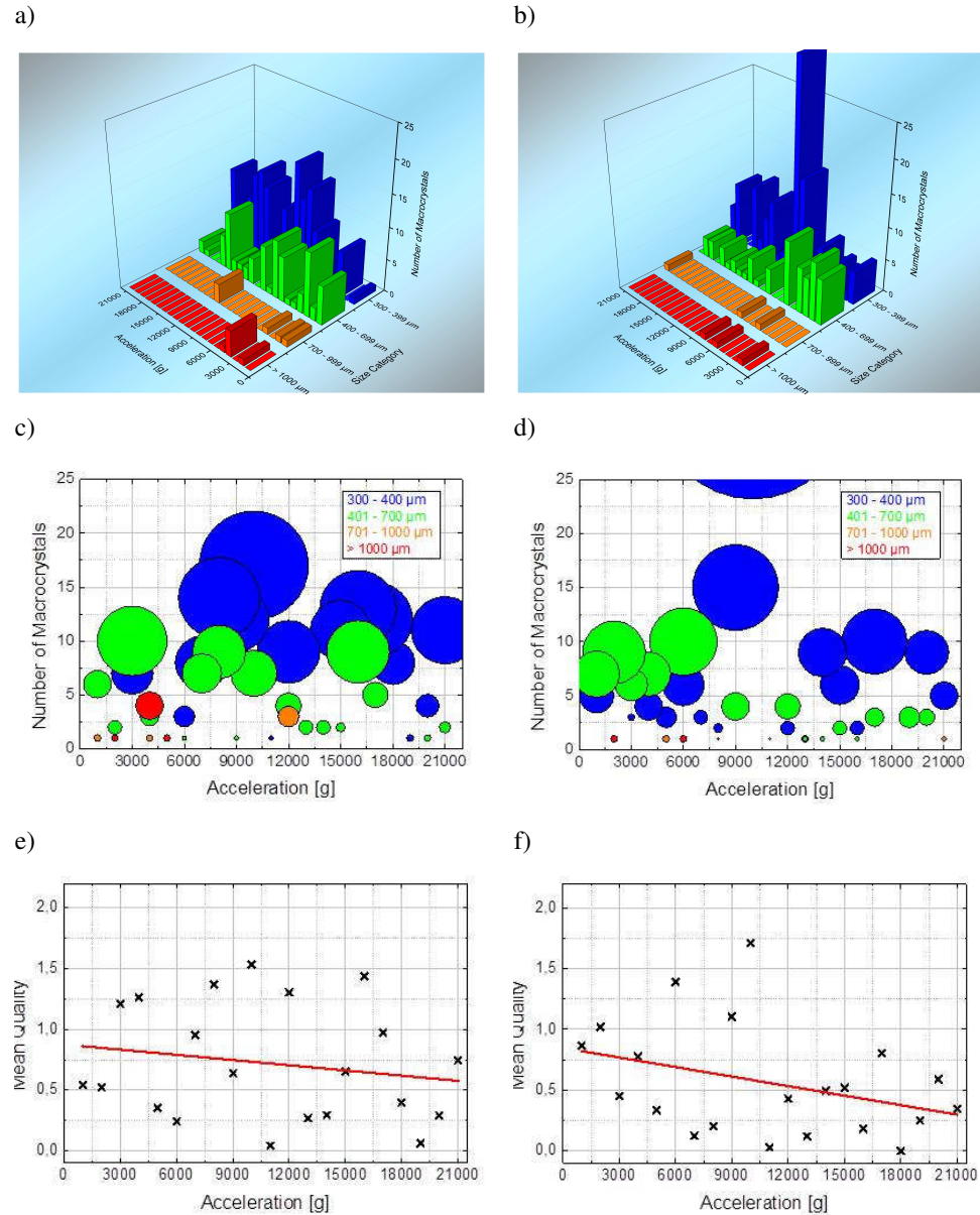
Figure 5.19: Number of macrocrystals per size category for all 21 samples centrifuged at 20°C a) without and c) with illustration of the score value S which corresponds to the dot size. e) Quality factor (black) and linear fit (red). b), d) and f) correspond to the reproduced samples.
