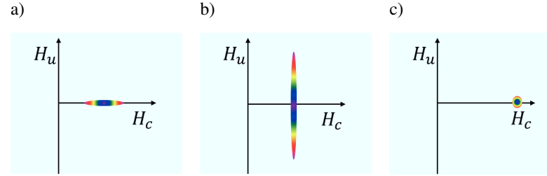
Figure 3.11: Theoretical FORC result obtained using easy axis hysterons for a) a normal coercivity distribution without interaction field and without coercivity distribution. b) Interaction field antiparallel to the magnetization direction c) Interaction field parallel to the magnetization direction.
