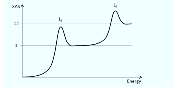
Figure 3.21: Schematic representation of a normalized XAS curve.
