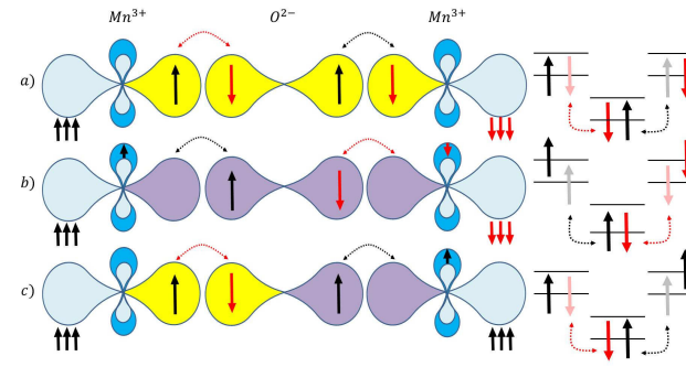
Figure 2.4: Super exchange interaction in manganese oxide for different geometries: Depending on the configuration, either antiparallel (a,b) or parallel (c) arrangement is energetically favorable. Yellow (purple) orbitals correspond to an antiparallel (parallel) coupling between oxygen and manganese, according to [59].
