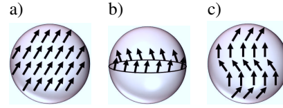
Figure 2.11: Illustration of possible magnetization reversal modes in single-domain nanoparticles: a) Coherent rotation occurs if all moments rotate in unison and always point into the same direction. b) For curling the spins are gradually wound up and in c) the buckling mode the spin structure is gradually compressed, according to [64].
