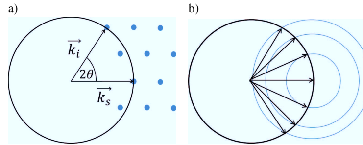
Figure 2.18: Intersection of the Ewald sphere with the reciprocal lattice for a) single crystals and b) polycrystalline powders.
