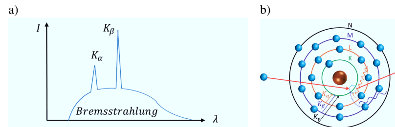
Figure 2.20: a) Schematic plot of a typical X-ray spectrum consisting of the continuous Bremsstrahlung and characteristic lines b) Illustration of electron transitions causing characteristic X-ray lines.
