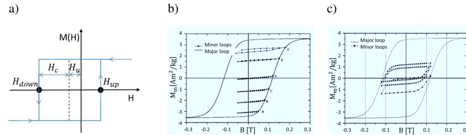
Figure 3.8: a) Graphical illustration of a hysteron displaying its threshold reversal fields H_{up} , H_{down} and offset H_u . b) Illustration of the wiping-out and c) congruency property, both reprinted with permission from [112].
