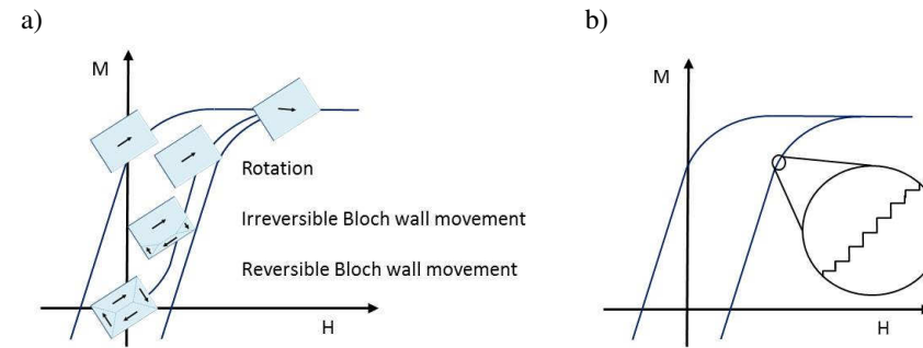
Figure 2.7: a) Illustration of the physical origin of ferromagnetic hysteresis loops. b) Barkhausen jumps.
