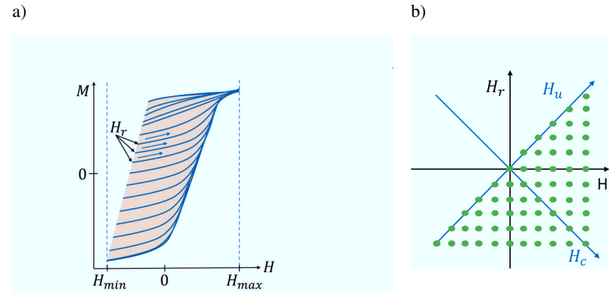
Figure 3.9: a) Example for a family of FORCs probing the interior of the corresponding major loop. b) Illustration of the relation between the H_r(H) and H_u(H_c) coordinate system. Green dots are representing single hysterons.
