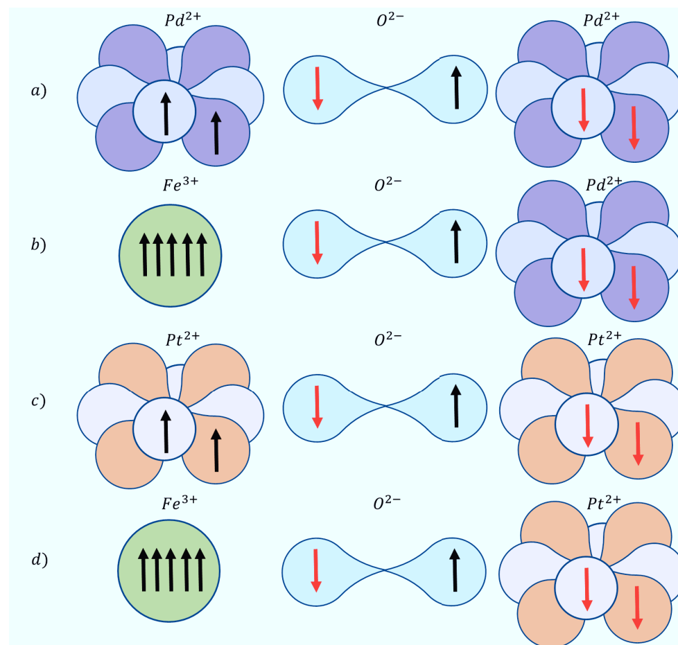
Figure 4.34: Spin arrangement for the a) -Pd-O-Pd- b) =Fe-O-Pd- c) -Pt-O-Pt- and d) =Fe-O-Pt- bond. For Pd and Pt ions only the two relevant d orbitals (one d orbital in a lighter, one in a darker shade) are shown. For the oxygen ions in the middle the relevant p orbital is depicted. Fe 3+ is spherical symmetric as 3d 5 ion and therefore depicted as sphere. In a crystal field environment the degeneracy of the d-orbitals is lifted but here the nanoparticle surface is considered where the crystal field has no defined symmetry so that the splitting is not well defined.
