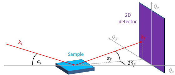
Figure 3.16: Schematical representation of the geometry required for GISAXS experiments, according to [120].
