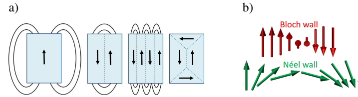
Figure 2.6: a) Domain formation and stray field reduction in ferromagnetic materials. b) Illustration of spin rotation within Bloch and Néel walls.
