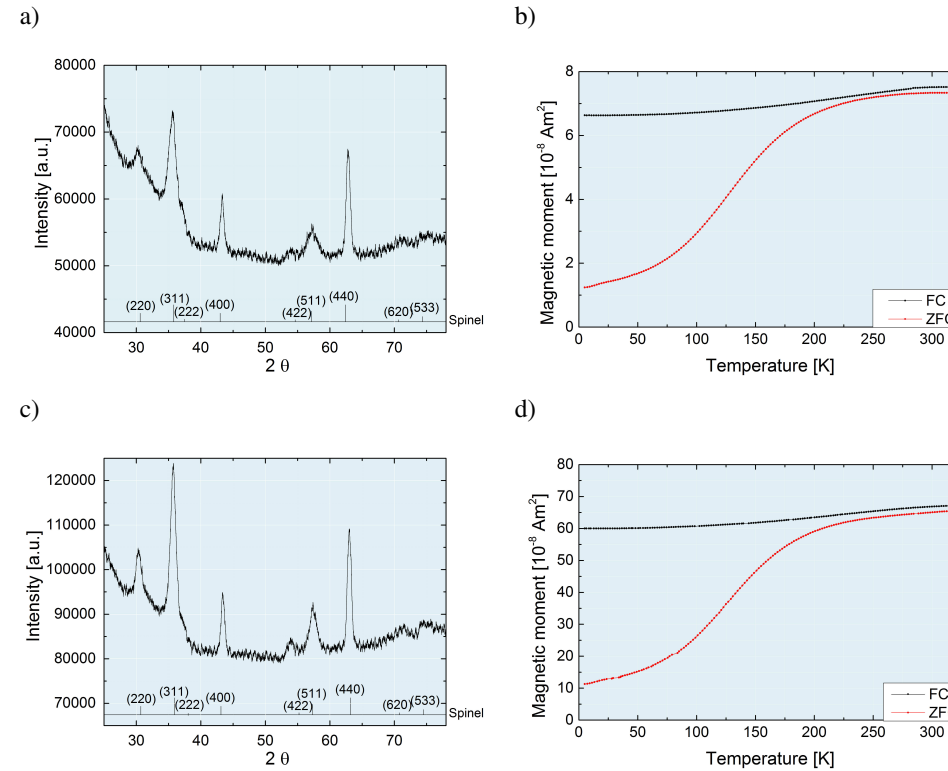
Figure 5.5: X-ray diffraction patterns together with simulated pattern for a spinel structure of a) batch O1, c) batch O2 and ZFC-FC curves obtained on a single macrocrystal consisting of nanoparticles from b) batch O1, d) batch O2.
