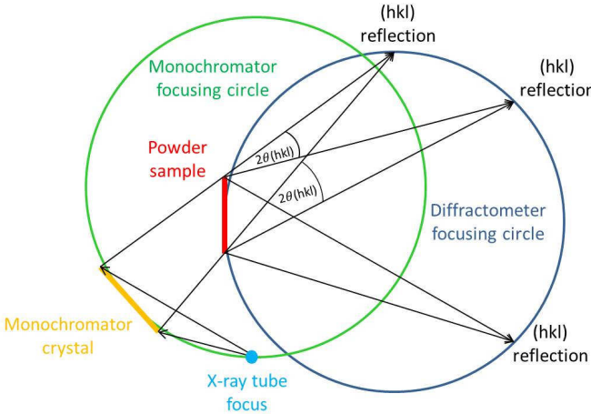
Figure 3.13: Geometrical principle of X-ray powder diffraction using the Guinier method in transmission geometry, according to [116].
