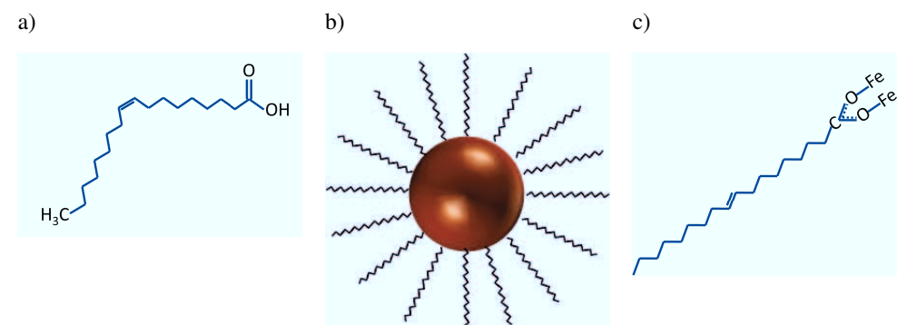
Figure 4.1: a) Chemical structure of oleic acid b) Schematic illustration of an iron oxide nanoparticle, sterically stabilized by oleic acid c) Bidentate interactions of the carboxylic head of oleic acid with iron ions on the surface of the nanoparticle, according to [138].
