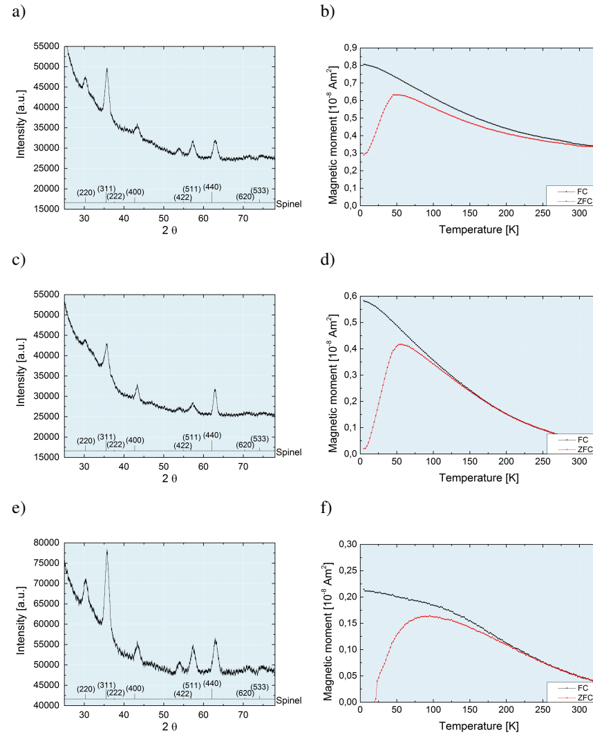
Figure 5.4: X-ray diffraction patterns together with simulated pattern for a spinel structure of a) batch C1, c) batch C2, e) batch C3 and ZFC-FC curves obtained on a nanoparticle (sub-)monolayer deposited on a silicon substrate using b) batch C1, d) batch C2, f) batch C3.
