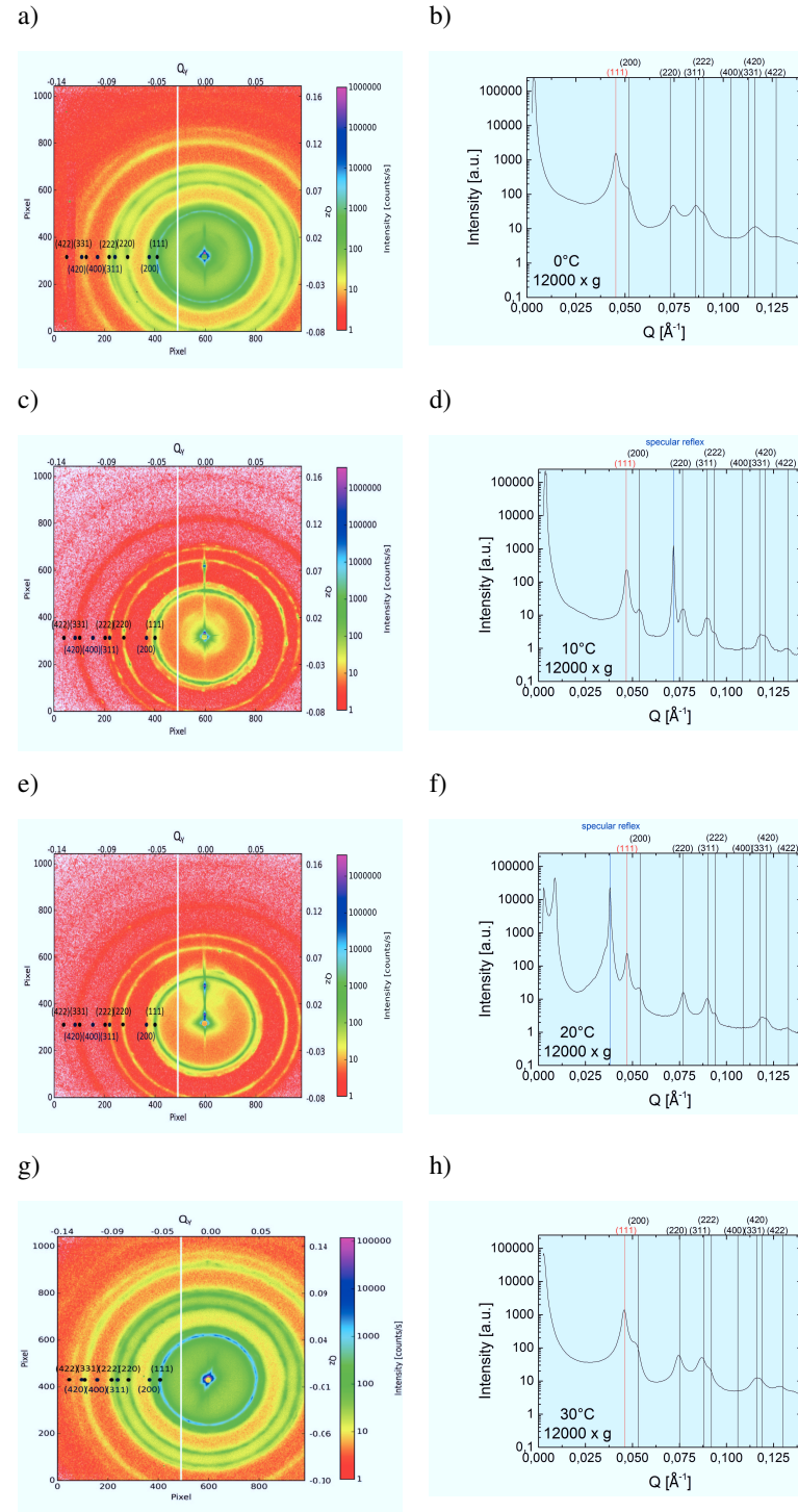
Figure 5.26: Batch O2: SAXS measurements performed on single macrocrystals removed from samples that were centrifuged at 12 000 x g (a,c,e,g) and radial integrated intensities (b,d,f,h). The measured (111) peak is labeled in red and further, calculated peak positions for a FCC lattice are shown in black. The specular reflex is highlighted in blue. The centrifugation temperature was a,b) 0°C, c,d) 10°C, e,f) 20°C, g,h) 30°C.
