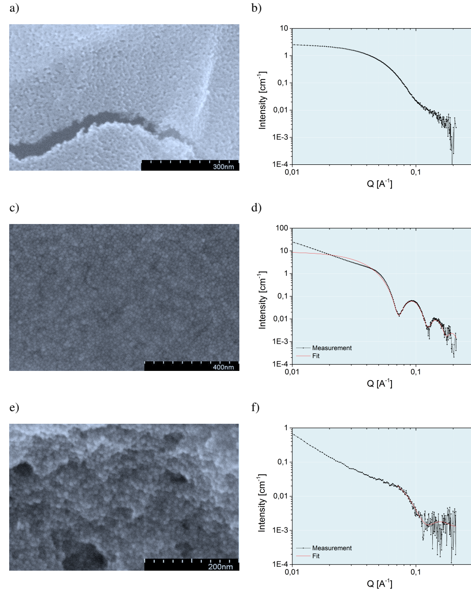
Figure 5.2: SEM images of iron oxide nanoparticles after deposition on a silicon substrate by drop casting, solvent evaporation and oxygen plasma cleaning for a) batch C1, c) batch C2, e) batch C3 and Small Angle X-ray Scattering patterns of 25/30 mg/ml dispersions obtained with GALAXI for b) batch C1, d) batch C2, f) batch C3.
