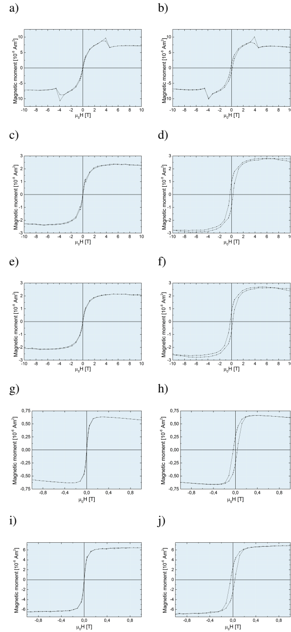
Figure 5.6: Hysteresis curves measured at 300 K (a,c,e,g,i) and 5 K (b,d,f,h,j) for batches C1 (a,b), C2 (c,d), C3 (e,f), O1 (g,h) and O2 (i,j) revealing superparamagnetic behavior.
