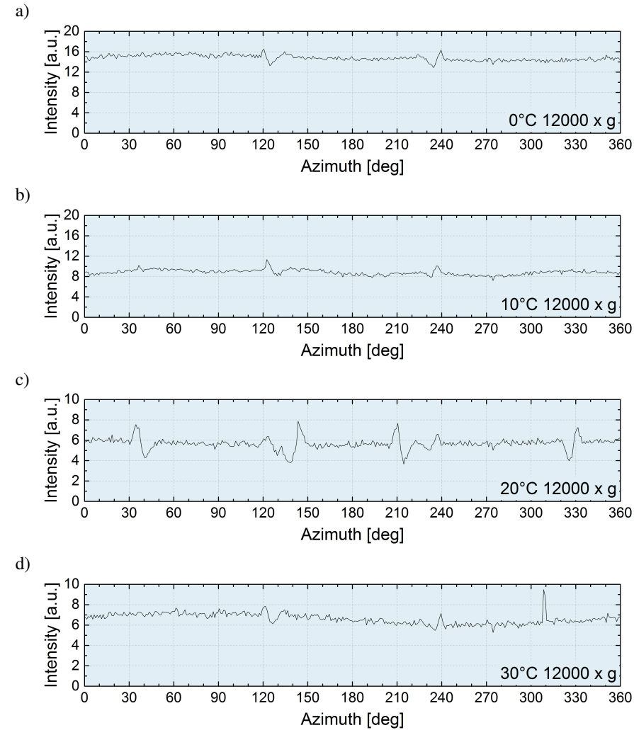
Figure 5.23: Intensities on the (111) powder ring as function of the azimuthal angle integrated over a ring width of 0.03 \text{ \AA}^{-1} for the SAXS patterns shown in figure 5.22 (batch O1).
