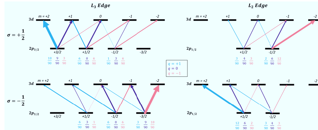
Figure 3.19: Spin-up ( \sigma = +\frac{1}{2} ) and spin-down ( \sigma = -\frac{1}{2} ) transition probabilities at the L_3 and L_2 edges for left-circular (pink, q=-1 ), linear (purple, q=0 ) and right circular polarized X-rays (blue, q=+1 ), according to [122].
