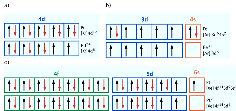
Figure 4.32: Orbital diagrams of a) palladium, b) iron, c) platinum and corresponding ions.
