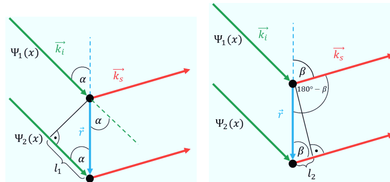
Figure 2.19: Geometrical construction for the calculation of the phase difference between two beams scattered at different particles separated by \vec{r} . The incoming and scattered waves are represented by the wave vectors \vec{k}_i and \vec{k}_s , respectively.
