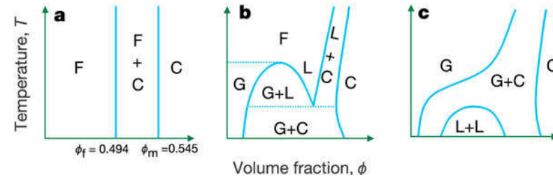
Figure 2.16: Phase diagrams for entropy driven crystallization a) without b) with long range and c) with short range interaction. The volume fraction is calculated by dividing the volume occupied by all the particles by the total volume, reprinted with permission from [76].
