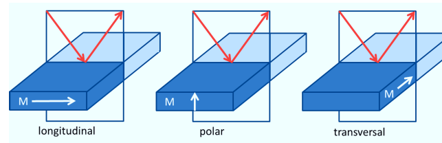
Figure 3.6: Illustration of geometric arrangement for the longitudinal, polar and transversal Kerr effect.
