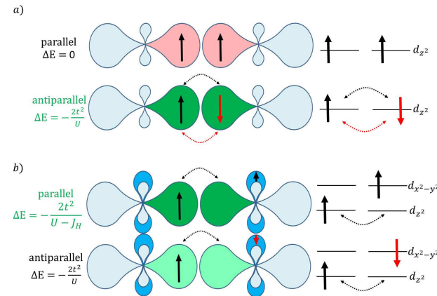
Figure 2.3: Energy gain due to hopping if a) neighboring lattice sites are both occupied, or b) every lattice site provides two degenerate energy levels and the considered one is empty. Green orbitals allow for electron hopping (darker green corresponds to larger energy gain), red orbitals not. According to [59].
