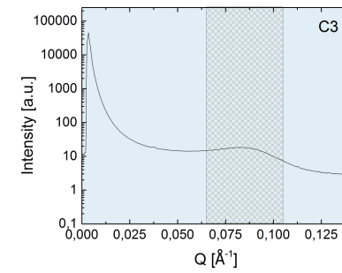
Figure 5.32: a,c,e) SAXS pattern of a single macrocrystal removed from samples centrifuged at 10°C and 21 000 x g using a) batch C1, b) batch C2, c) batch C3 and b,d,f) radial integrated intensities. The gray area marks the region over which the intensity is integrated for the plots shown in figure 5.31.
