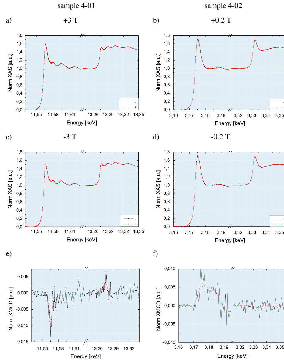
Figure 4.22: XAS measurements for a left and right circularly polarized beam after field-cooling from 300 K to 5 K for a) sample 4-01 with an angle of incidence of 1^\circ and a polarization efficiency of 85% at +3 T and c) -3 T and for b) sample 4-02 with an angle of incidence of 2.2^\circ and a polarization efficiency of 69% at +0.2 T and d) -0.2 T. The corresponding XMCD signals (black) and smoothed curves as guide to the eye (red) are respectively shown in e) for sample 4-01 and f) for sample 4-02.
