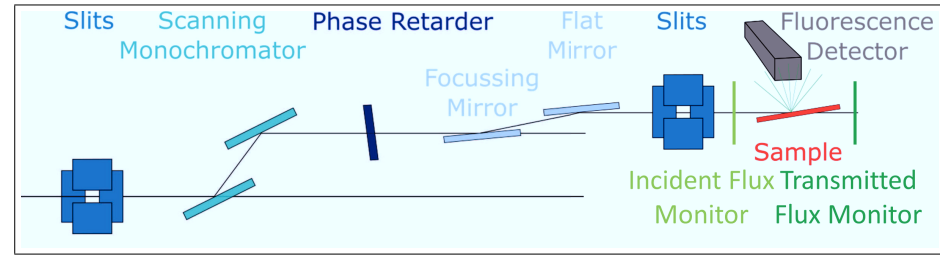
Figure 3.20: Schematic setup of the 4-ID-D Beamline at APS for XMCD measurements, inspired by [39].
