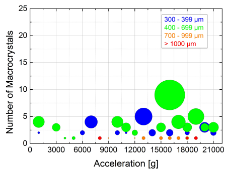
Figure 5.13: Number of macrocrystals per size category for the reproduced samples at a centrifugation temperature of 0°C a) without and b) with illustration of the score value S which corresponds to the dot size. c) Quality factor (black) and linear fit (red).
