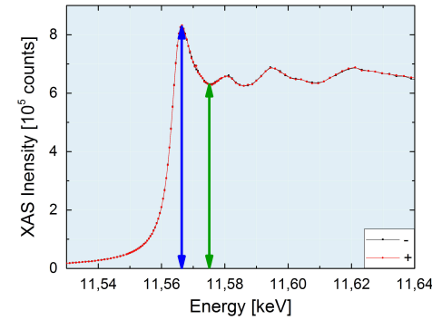
Figure 4.33: Sample 4-01: X-ray absorption spectroscopy measurement without normalization performed at the Pt L_3 edge. The edge intensity is indicated by a blue arrow. The green arrow shows the signal intensity in the XANES region.
