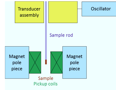
Figure 3.1: Schematic illustration of the vibrating sample magnetometer setup.
