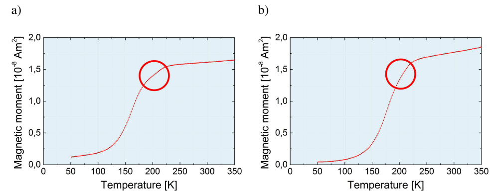
Figure 4.14: Comparison of ZFC curves (measured at \mu_0 H = 0.005 \text{ T} ) for a) a sample treated with oxygen plasma for 11 min (3-07) and b) 12 min (3-08), displaying the necessary duration for phase transition completion.
