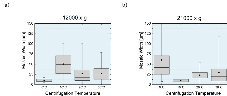
Figure 5.30: Boxplots summarizing the 'mosaic widths' determined from the FWHM of the peaks identified in azimuthal direction on the (220) powder ring for the measurements shown in figures 5.27 and 5.29. The black dots mark the average values and the whiskers indicate minimum and maximum. Bottom and top of the boxes are the first and third quartiles, respectively. The bands inside the boxes show the median values.
