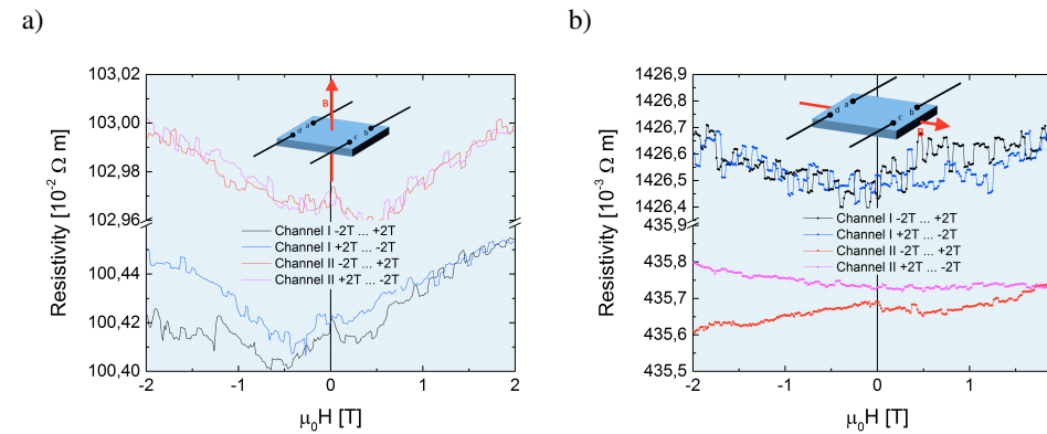
Figure 4.24: Sample 5-02 (NPs + 5 nm palladium): Resistivity measurements performed at 10 K according to the van der Pauw method with the magnetic field applied a) out-of-plane and b) in plane. For channel I the current flows between a and b and for channel II it flows between b and c.
