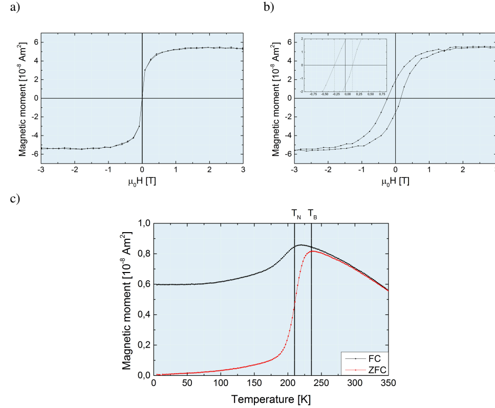
Figure 4.8: Sample 2-10: Hysteresis loops at a) 300 K and b) 5 K showing superparamagnetic behavior and exchange bias. c) ZFC (red) and FC (black) curve measured at \mu_0 H = 0.005 T revealing a blocking temperature T_B of 237 \pm 2 K and a combined ferri- and antiferromagnetic behavior with a Néel temperature T_N of 210 \pm 2 K.
