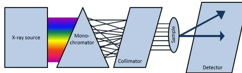
Figure 3.14: Schematic overview on the general measurement setup for (GI)SAXS experiments.
