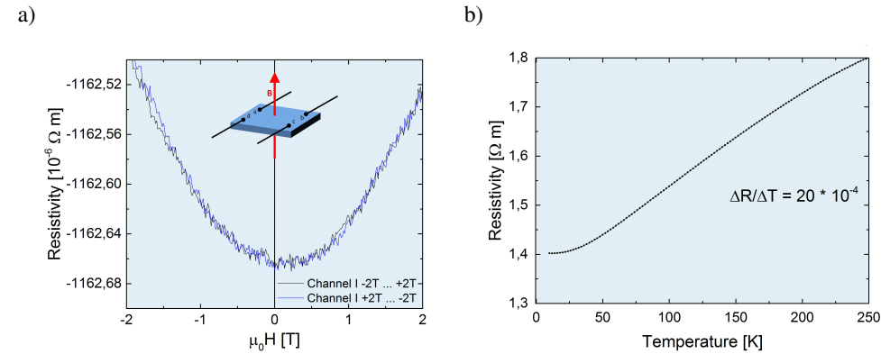
Figure 4.29: Sample 5-03: Magnetic field and temperature dependency of the resistivity for the out-of-plane geometry.
