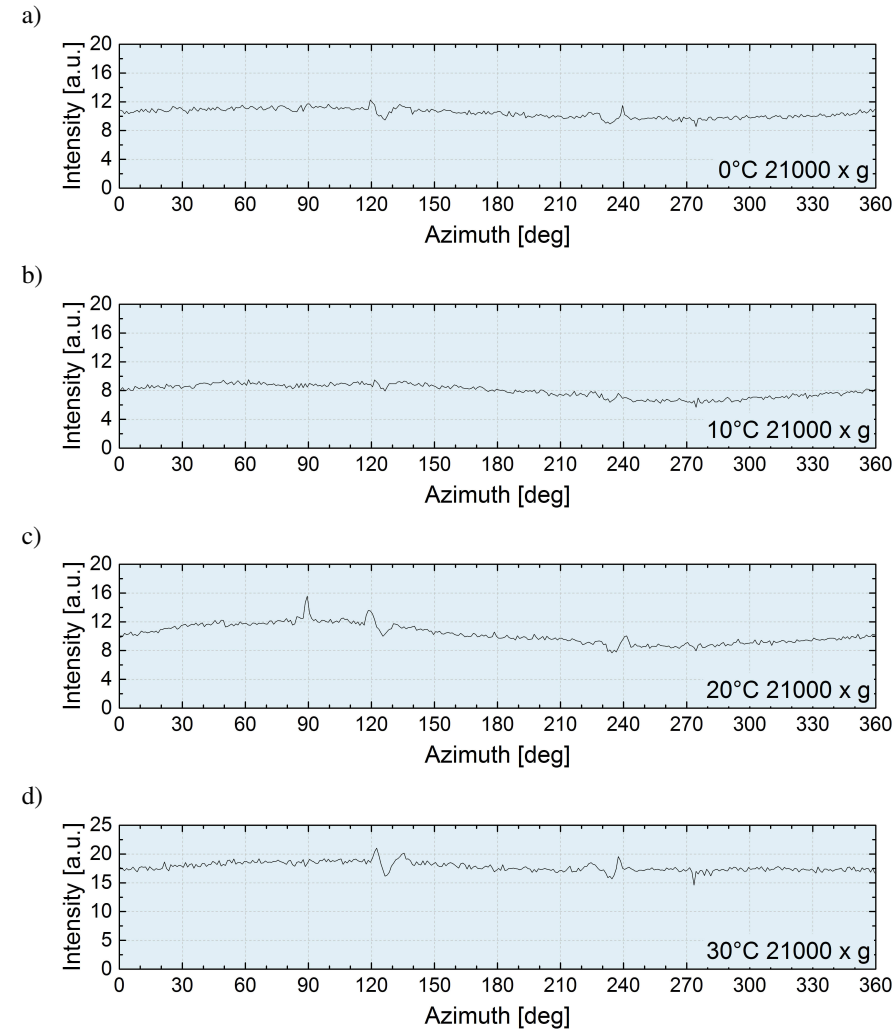
Figure 5.25: Intensities on the (111) powder ring as function of the azimuthal angle integrated over a ring width of 0.03 \text{ \AA}^{-1} for the SAXS patterns shown in figure 5.24 (batch O1).
