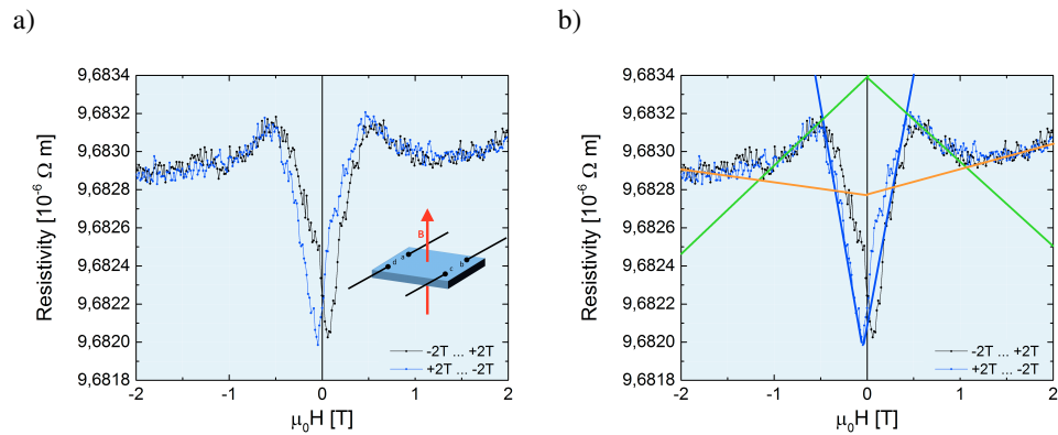
Figure 4.30: Sample 5-04: a) Magnetic field dependency of the resistivity for the out-of-plane geometry. The lines shown in b) are a guide to the eye to highlight the Lorentz (orange), spin disorder (green) and nanoparticle magnetoresistance effect (blue).
