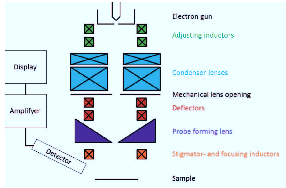
Figure 3.22: Schematical setup for a scanning electron microscope.
