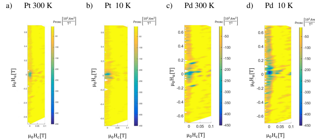
Figure 4.17: FORC distributions for a,b) sample 4-01 (Pt covered) and sample 4-02 (Pd covered) obtained at a,c) 300 K and b,d) 10 K showing significant changes in the interaction field distribution upon temperature reduction and a negligible coercivity field distribution.
