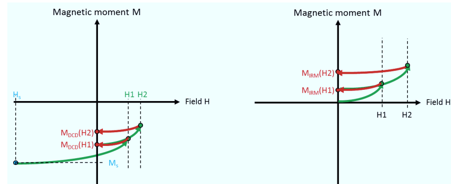
Figure 3.4: Illustration of measurement procedure for DCD (left) and IRM (right) curves.
