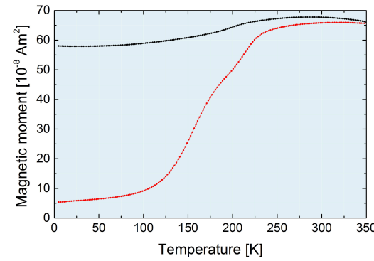
Figure 5.37: ZFC-FC curves measured on the nanoparticle/palladium multilayer revealing that the nanoparticles still contain wustite remains despite the extensive oxygen plasma treatment.
