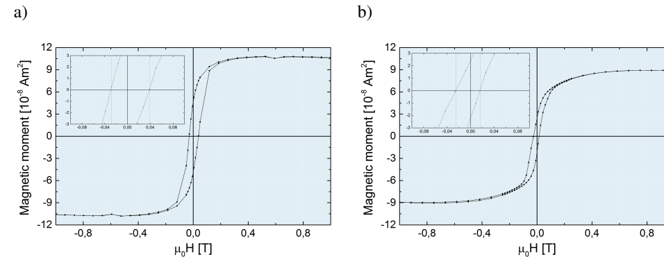
Figure 4.19: Hysteresis curves obtained at 5 K for a) the platinum covered sample 4-01 and b) the palladium covered sample 4-02 demonstrating that -1 T are sufficient for negative saturation.
