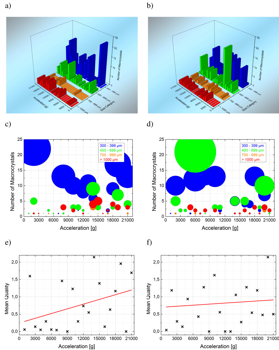
Figure 5.14: Number of macrocrystals per size category for all 21 samples centrifuged at 10°C a) without and c) with illustration of the score value S which corresponds to the dot size. e) Quality factor (black) and linear fit (red). b), d) and f) correspond to the reproduced samples.
