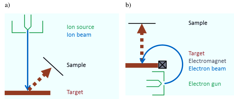
Figure 3.23: Setup illustration for a) Ion Beam Sputtering and b) Molecular Beam Epitaxy.
