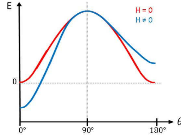
Figure 2.12: Energy of a single-domain nanoparticle in dependency of the angle \theta between the superspin and the anisotropy axis, according to the Stoner-Wohlfarth model for zero applied field (red) and a magnetic field with h = \frac{\mu_0 H M_s}{2K} = 0.2 (blue), according to [64].
