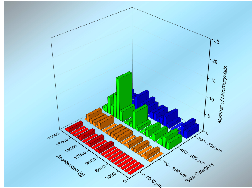
Figure 5.10: Number of macrocrystals per size category for all 21 samples prepared at a centrifugation temperature of 0 °C.
