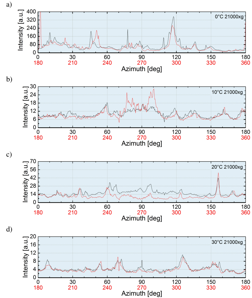
Figure 5.29: Intensities on the (220) powder ring as function of the azimuthal angle integrated over a ring width of 0.01 \text{ \AA}^{-1} for the SAXS patterns shown in figure 5.28 (batch O2).
