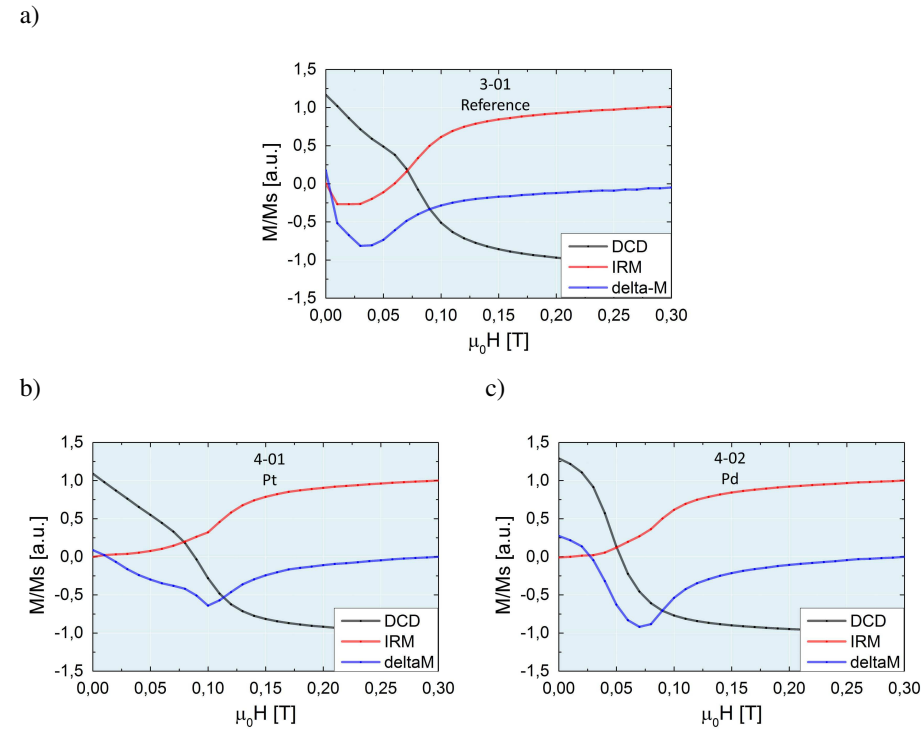
Figure 4.20: DCD (black), IRM (red) and Delta-M (blue) curves for a) the uncovered sample 3-01, b) sample 4-01 which is covered with 2 nm of platinum and c) sample 4-02 on which 5 nm of palladium showing different strengths of demagnetizing interaction.
