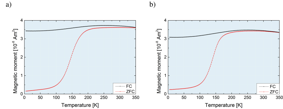
Figure 4.15: ZFC (red) and FC (black) curves (measured at 0.005 T) for a) sample 4-01 which is covered with 2 nm platinum and b) sample 4-02 where 5 nm of palladium are applied. Both curves exhibit characteristics similar to the uncovered sample 3-01 (cf. figure 4.10).
