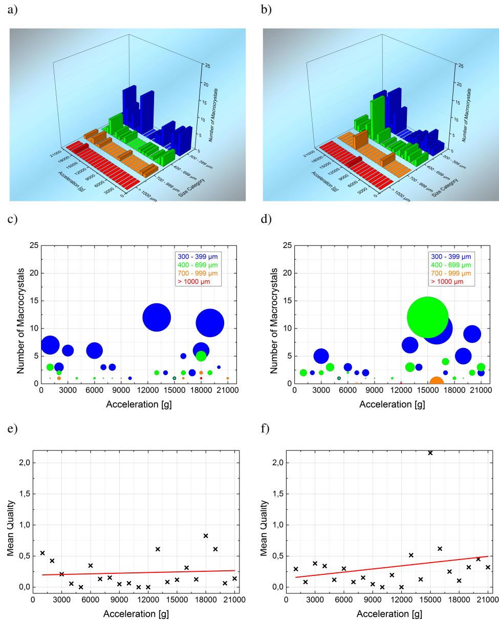
Figure 5.16: Number of macrocrystals per size category for all 21 samples centrifuged at 30°C a) without and c) with illustration of the score value S which corresponds to the dot size. e) Quality factor (black) and linear fit (red). b), d) and f) correspond to the reproduced samples.
