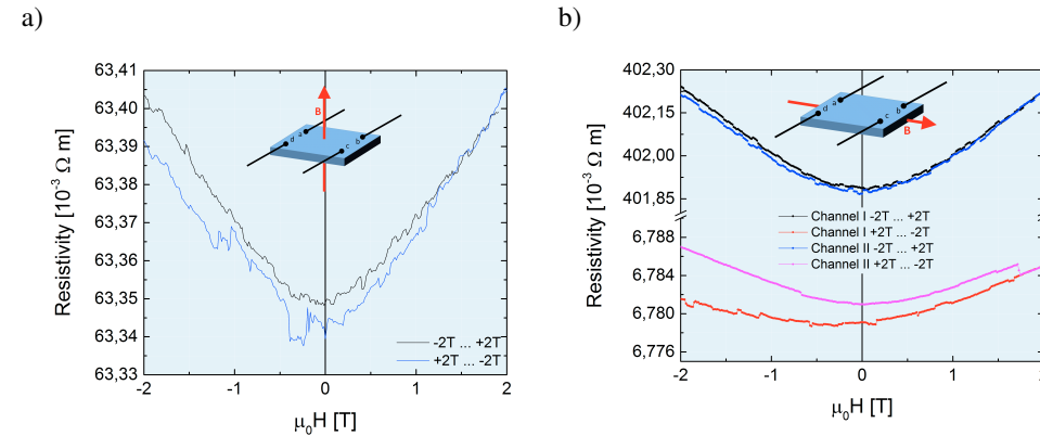
Figure 4.23: Sample 5-01 (reference sample, 5 nm palladium only): Resistivity measurements performed at 10 K according to the van der Pauw method with the magnetic field applied a) out-of-plane and b) in plane. For channel I the current flows between a and b and for channel II it flows between b and c.
