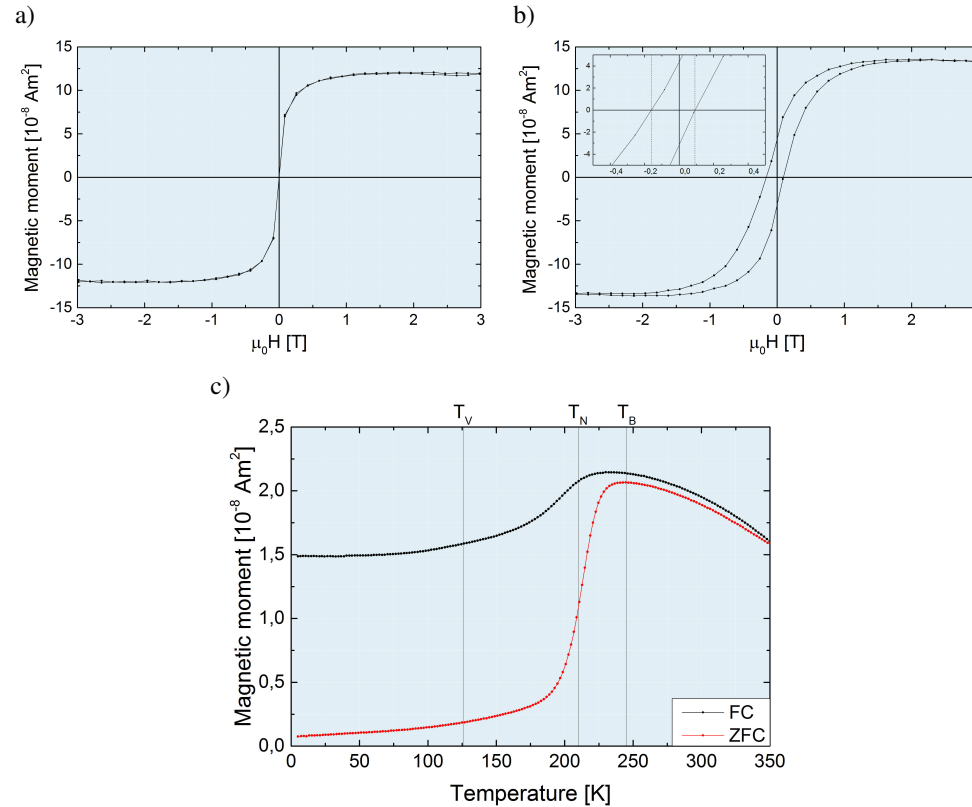
Figure 4.5: Sample 1-01: Hysteresis loops at a) 300 K and b) 5 K showing superparamagnetic behavior and exchange bias. c) ZFC (red) and FC (black) curve measured at \mu_0 H = 0.005 \text{ T} revealing a blocking temperature T_B of 245 \pm 2 \text{ K} and a combined ferri- and antiferromagnetic behavior with a Néel temperature T_N of 210 \pm 2 \text{ K} .
