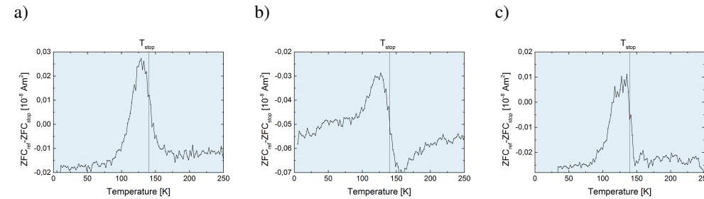
Figure 4.16: Memory effect measurements performed with an aging stop at 140 K for 10000 s on a) the uncovered sample 3-01, b) sample 4-01 which is covered with 2 nm of platinum and c) sample 4-02 on which 5 nm of palladium are applied.
