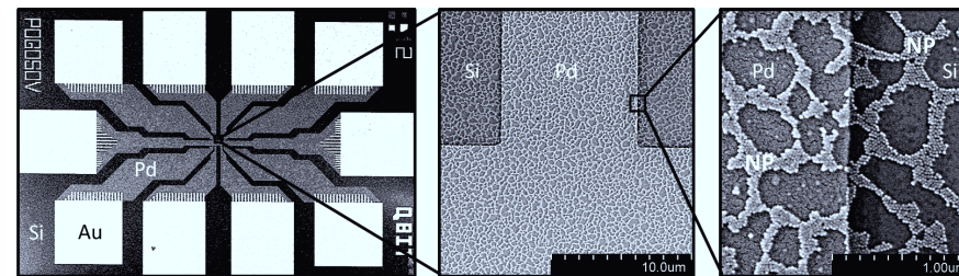
Figure 4.28: Sample 5-03: SEM image of the Hall bar structure manufactured by a two step lithography process. The enlarged section on the right shows that the nanoparticles still remain on the surface, covered by a thin, homogeneous Pd film.
