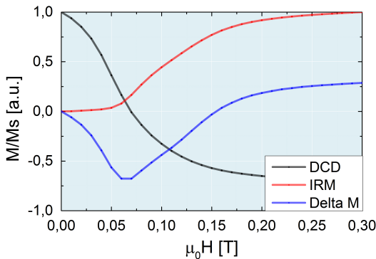
Figure 5.40: Nanoparticle/palladium multilayer: IRM (red), DCD (black) and Delta-M (blue) curves indicating a polarization effect.
