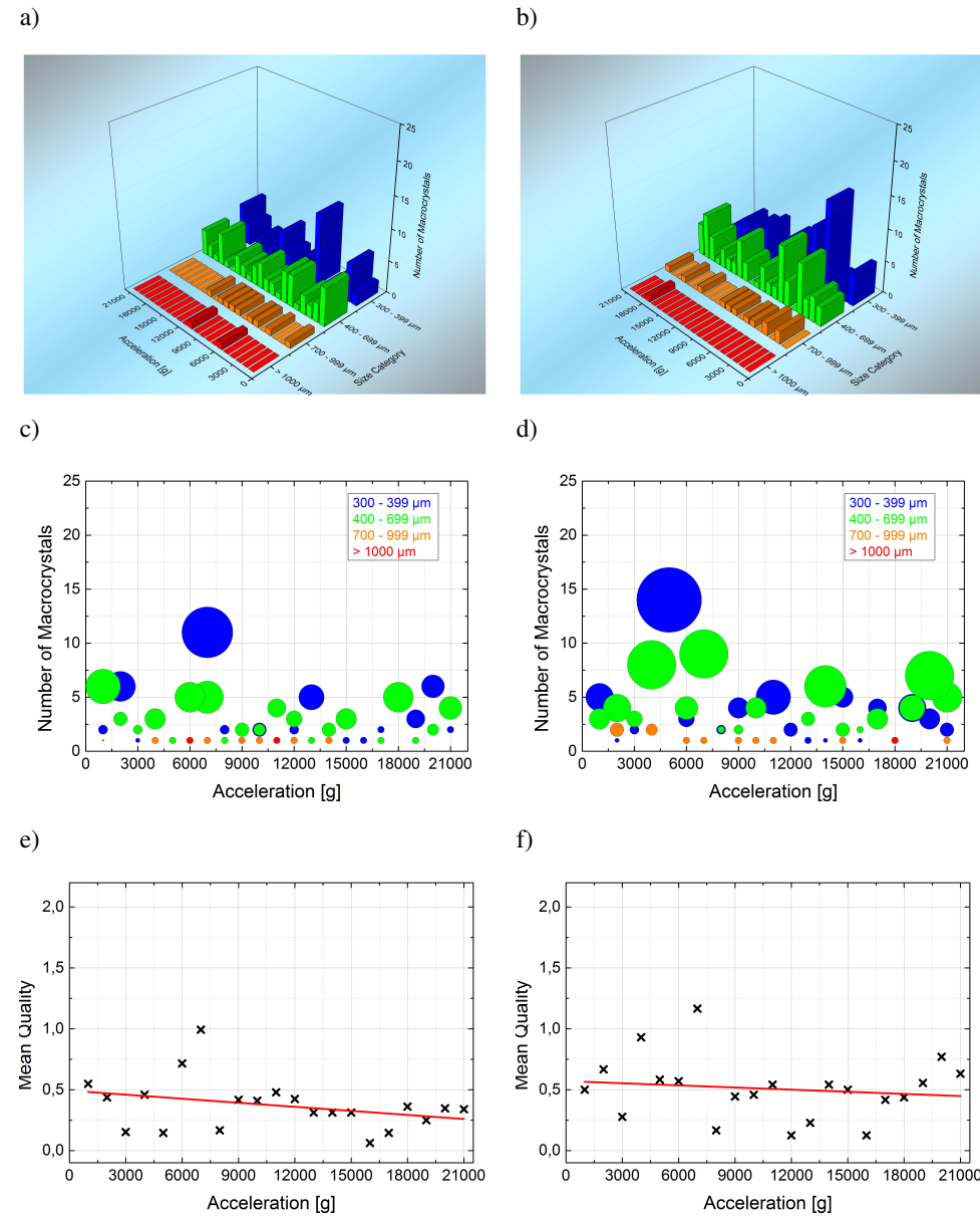
Figure 5.15: Number of macrocrystals per size category for all 21 samples centrifuged at 20°C a) without and c) with illustration of the score value S which corresponds to the dot size. e) Quality factor (black) and linear fit (red). b), d) and f) correspond to the reproduced samples.
