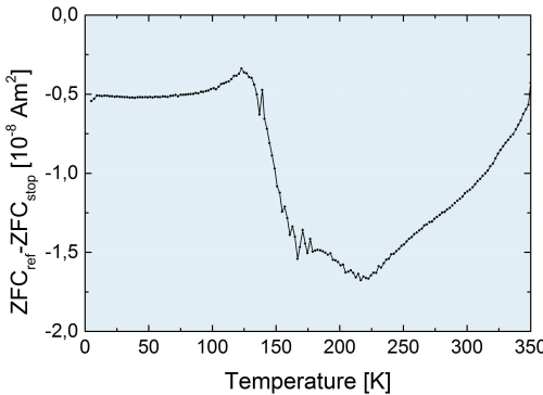
Figure 5.39: Nanoparticle/palladium multilayer: Memory effect measurement performed with an aging stop at 140 K for 10 000 s demonstrating the superspin glass state of the system. The peak broadening is assigned to the mixed wustite/maghemite iron oxide phase inside the nanoparticles.
