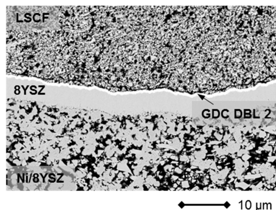
Figure 13. SEM image of a cross-section through an MSC highlighting the GFS applied 8YSZ electrolyte and the GDC diffusion barrier after operation. The cell was activated in situ for 100 h in a dual gas atmosphere at 850 ^{\circ}\text{C} and operated for 100 h at 750 ^{\circ}\text{C} .
