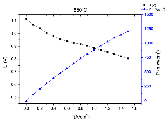
Figure 1. I–V curve of a planar 5 \text{ cm} \times 5 \text{ cm}^2 single cell MSC with a 4 \mu\text{m} thin layer 8YSZ electrolyte, a Ni/8YSZ anode and an LSCF cathode at 850^\circ\text{C} in 3% humidified hydrogen after 10 h of in-situ activation. For more details about the manufacturing refer to Section 3.
