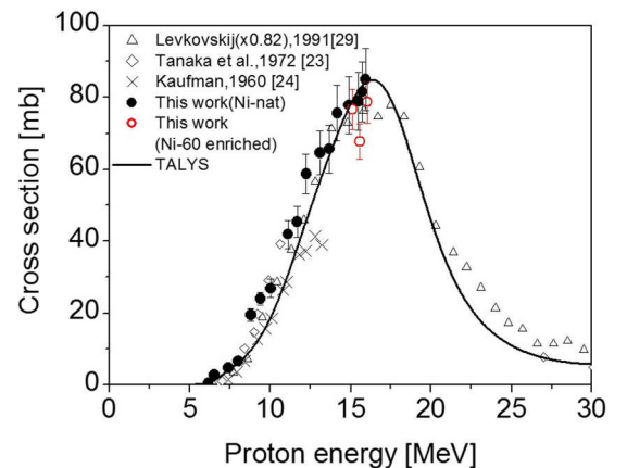
FIG. 3. Measured and calculated excitation function of the ^{60}\text{Ni}(p, \alpha)^{57}\text{Co} process.
