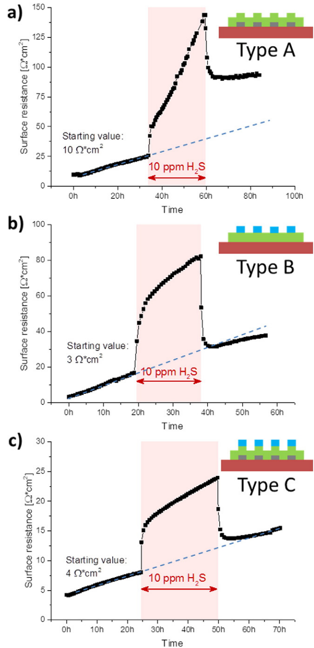
Fig. 10. Long term evolution of the surface polarization resistance during sulphur poisoning experiments of different electrode types, see Fig. 4, a) Type A, b) Type B and c) Type C, the GDC layers were of 200 nm thickness, the current collector of A is 100 nm Pt, the oxide current collectors of electrodes B and C were made of 200 nm of STN-982. Measurements were performed at 750 ^{\circ}\text{C} in a symmetrically heated setup in a gas atmosphere of humidified \sim 2.5 vol% \text{H}_2 in Ar, with a ratio of hydrogen to water of 1:1.
