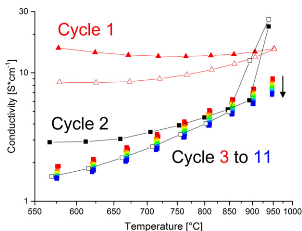
Fig. 3. Multiple total conductivity measurements of a 200 nm thick layer of Sr 0.9 Ti 0.8 Nb 0.2 O 3 on a magnesia single crystal using the van der Pauw method. Measurements were performed in humidified ~2.5 vol% H 2 in Ar, with a ratio of hydrogen to water of 1:1. Previous to the measurements of cycle 1 and 2 the sample was measured in a dry hydrogen atmosphere. Cycles 3 to 11 were recorded consecutively without previous reduction in dry hydrogen, the arrow indicates a successive decline in the conductivity.
