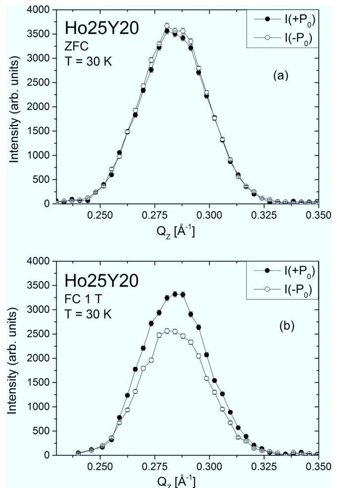
FIG. 2. The Q dependence of the neutron-scattering intensity (reflectivity profile) for the samples Ho25/Y20, taken for two polarizations of the incident beam at T = 30 K after the ZFC procedure (a) and FC procedure at an applied field H = 1 T (b).
