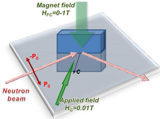
FIG. 1. (Color online) The schematic drawing of the experiment.
