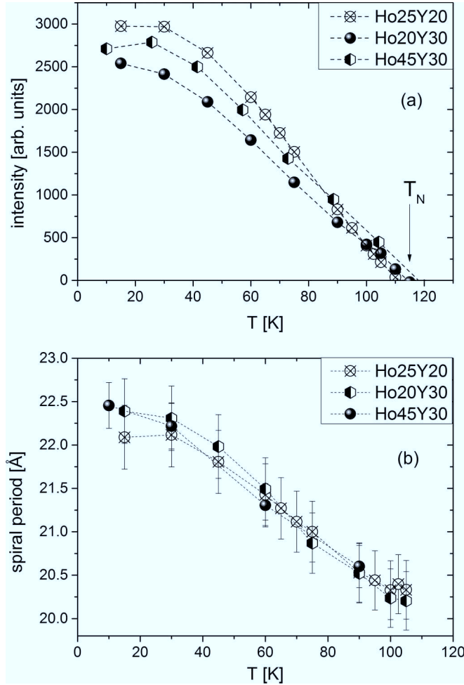
FIG. 3. Temperature dependence of magnetic intensity (a) and the spiral period in the Ho layer (b).
