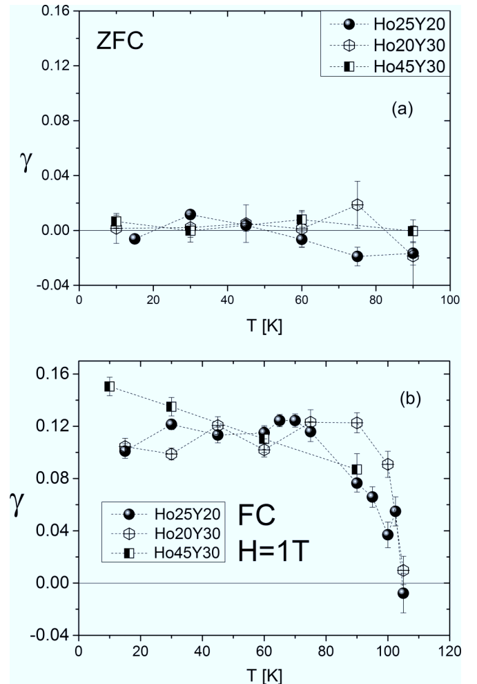
FIG. 4. The chirality for the samples Ho25Y20, Ho20Y30, and Ho45Y30 in dependence on temperature prehistory: (a) T dependence after ZFC, and (b) T dependence after FC under an applied field H = 1 T.
