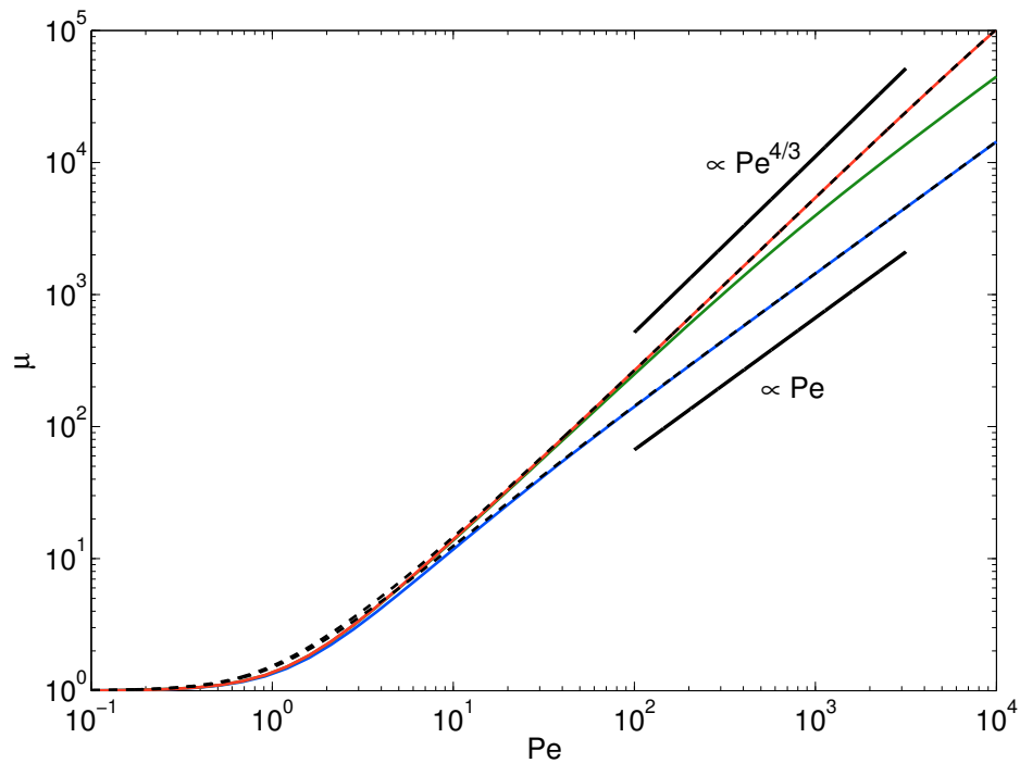
Figure 3. Normalized stretching coefficient \mu = 2\lambda/3p as function of the Péclet number for pL = 10^1, 10^2 and 10^3 (bottom to top). In all cases, we set l = 1/p , which corresponds to L/l = pL and \Delta = 1/3 . The dashed lines represent the solution of the asymptotic Equation (31). The straight lines indicate the power-law dependencies \mu \sim Pe^{4/3} for N = 10^3 and \mu \sim Pe for N = 10 (cf. Equations (32) and (33), respectively).
