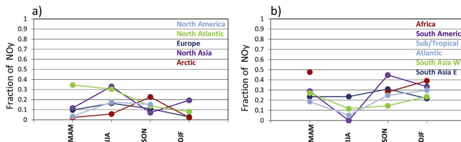
Fig. 4. Fraction of \text{NO}_y measured in high CO air masses in the northern ( >40^\circ\text{N} , a) and southern ( <40^\circ\text{N} , b) regions. See text for more information.
