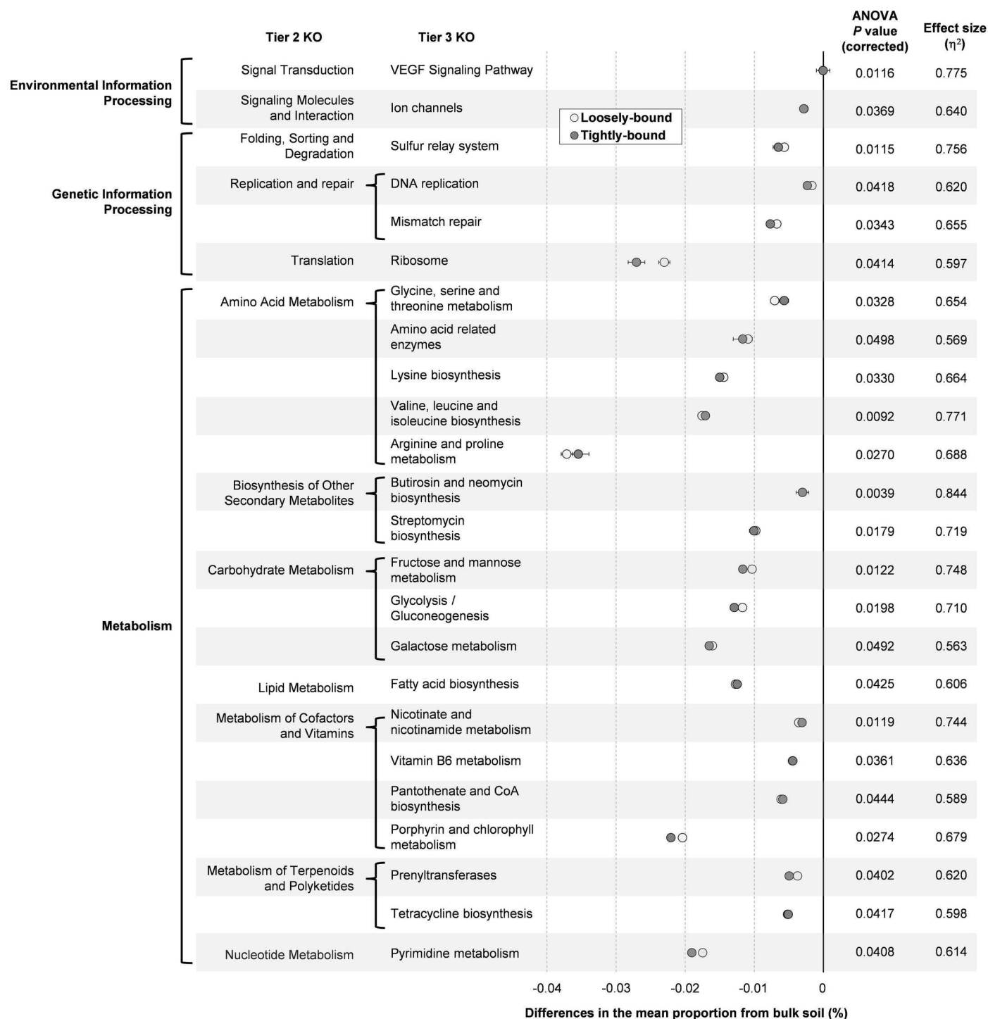
Fig 5. PICRUSt predicted bacterial functional gene content that was decreased in the Brachypodium rhizosphere. Differences in the abundance of categorized gene functions (tier 3 KO) in the loosely-bound and tightly-bound rhizospheres are plotted against the bulk soil (= 0 on the x-axis). Only categories that were significantly decreased in the rhizospheres (both loosely-bound and tightly-bound) compared to bulk soil are shown (ANOVA, Benjamini-Hochberg FDR corrected P < 0.05 ). Data are means \pm SE ( n = 4-5 ).
