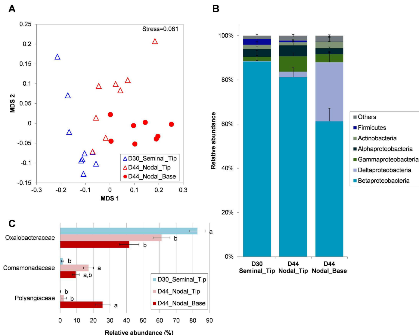
Fig 3. 16S pyrosequencing revealed the bacterial communities colonizing the seminal root tip at day 30, and the root tip and base of nodal roots at day 44. (A) NMDS ordination plot (based on Bray-Curtis similarity) where each point represents the bacterial community in one root sample. (B) Abundance of bacterial phyla in each root type (Proteobacteria further classified into classes). (C) Bacterial families significantly different in abundance between root types (different lower case letters indicate ANOVA P < 0.05 ). Only Orders with >10\% relative abundance in any root type are shown. Data are means \pm SE ( n = 8-9 ).
