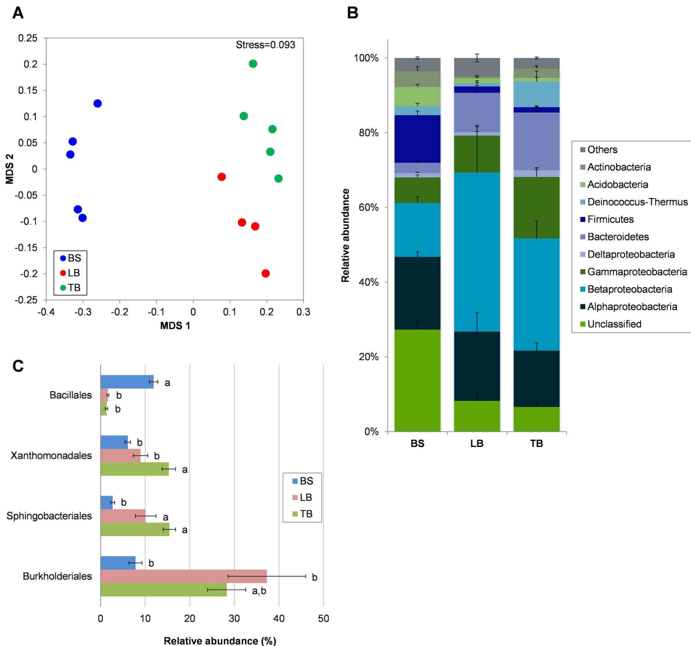
Fig 1. Bacterial community in the bulk soil (BS) and in the loosely-bound (LB) and tightly-bound (TB) fractions of the Brachypodium Bd21-3 rhizosphere, revealed with 16S pyrosequencing. (A) NMDS ordination plot (based on Bray-Curtis similarity), where each point represents the bacterial community in a soil/rhizosphere fraction for one plant. (B) Abundance of bacterial phyla in the bulk soil and rhizosphere (Proteobacteria is further classified into classes). (C) Bacterial Orders that are significantly different in abundance between the sample groups (different lower case letters indicate ANOVA P < 0.05 ). Only Orders with > 10\% relative abundance in any sample type are shown. Means are shown \pm SE ( n = 4-5 ).
