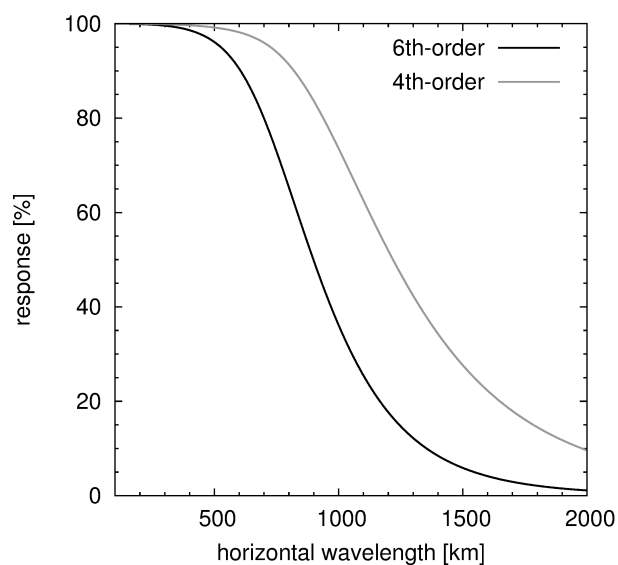
Figure 2. Amplitude response of the AIRS 15 \mu\text{m} brightness temperature data set for gravity waves with different across-track wavelengths. The plot shows the response using a 4th- or 6th-order polynomial fit to estimate background signals.
