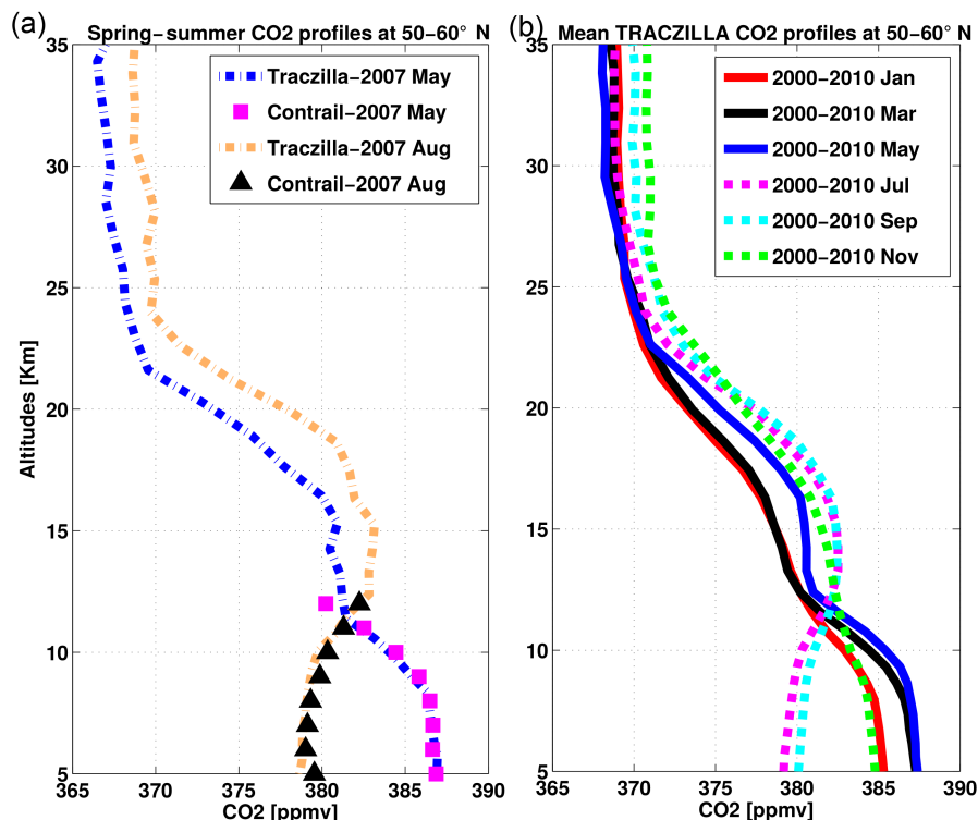
Figure 7. (a) Reconstructed vertical profiles of the mean CO 2 compared with CONTRAIL measurements for 2007 at 50–60° N. Dotted and dashed lines show vertical profiles of CO 2 from TRACZILLA (blue: May, orange: August). Symbols show in situ aircraft measurements from the CONTRAIL campaign (magenta square: May, black triangle: August). (b) Averaged monthly profiles of the reconstructed CO 2 over the period 2000–2010 after removal of the mean CO 2 trend at each level and centred on 2007. Red is January, black is March, blue is May, magenta is July, cyan is September, and green is November.
