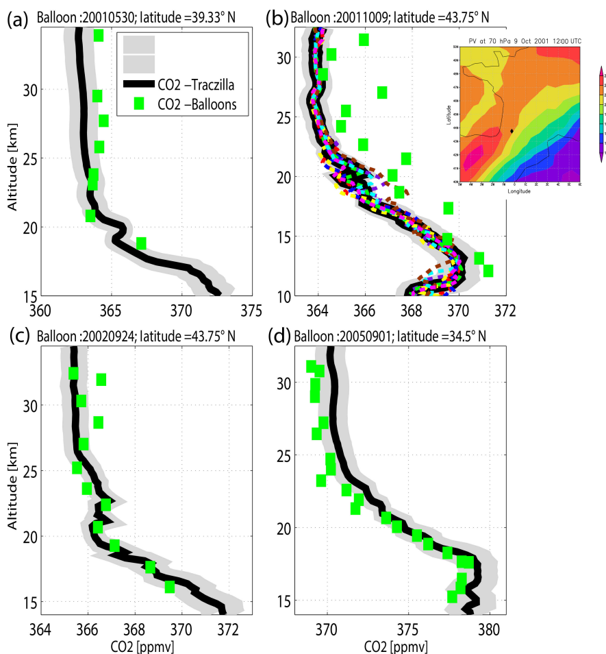
Figure 4. Reconstructed vertical profiles of the monthly mean CO 2 compared with each in situ stratospheric balloon observation of CO 2 (Engel et al., 2009). Black curves show reconstructed vertical profiles of mean CO 2 . Green squares show in situ balloon measurements of mean CO 2 . Grey shading shows the 95 % confidence interval from the reconstruction. The measurements were taken from Sanriku, Japan (39.33 °N), on 30 May 2001 (a); Aire sur l'Adour, France (43.75 °N), on 9 October 2001 (b) and on 24 September 2002 (c); and Fort Sumner, New Mexico, USA (34.5 °N), on 1 September 2005 (d), respectively. The different dashed lines show the other eight reconstructed profiles surrounding the measurement on 9 October 2001. The insert on the upper right panel shows the potential vorticity (in PVU) on the 70 hPa surface for 9 October 2001 at 12:00 UTC over France from ERA-Interim. The location of Aire sur l'Adour is indicated by a diamond.
