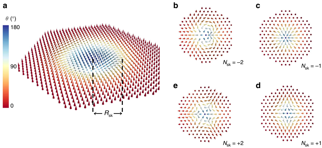
Figure 3 | Skyrmionic magnetic structures. (a) Hexagonal unit cell for the tight-binding model, containing 961 magnetic sites. It is 8.4 nm wide, using the lattice constant of the Pd/Fe/Ir(111) system. The cones show the orientation of the spin moments and are coloured by their polar angle. The skyrmion radius, R_{sk} , is defined by \theta(R_{sk}) = 90^\circ . (b–e) Top view of structures with different skyrmion numbers, N_{sk} = -2, -1, +1, +2 , respectively (equation 2; here \gamma = 0 ). The chiral skyrmions in Pd/Fe/Ir(111) correspond to N_{sk} = -1 . Achiral skyrmions have N_{sk} = +1 .
