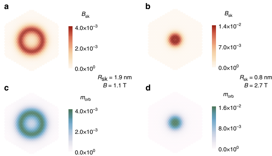
Figure 4 | Chirality-driven orbital moments in skyrmions of different sizes ( N_{sk} = -1 ). (a,b) Emergent magnetic flux per site, B_{sk} (equation (2)), for the skyrmion profiles characterized by R_{sk} = 1.9 nm and R_{sk} = 0.8 nm, corresponding to applied magnetic fields of B = 1.1 T and B = 2.7 T, respectively. (c,d) Orbital moment per site in \mu_B , m_{orb} , generated by the respective emergent magnetic fluxes shown in a,b, without SOC, computed using the tight-binding model for Pd/Fe/Ir(111).
