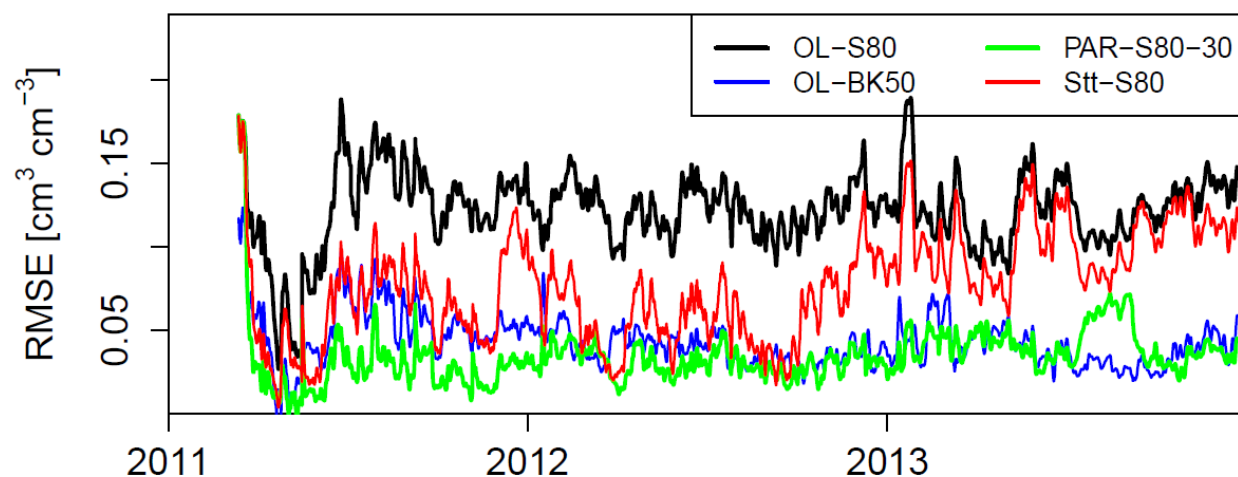
Fig. 4. Temporal evolution of root mean square error ( E_{\text{RMS}} ) for hourly SWC retrievals. E_{\text{RMS}} is calculated hourly for nine CRP's for open loop runs for soil maps S80 and BK50, joint state-parameter updates (PAR-S80-30) and state updates only (Stt-S80) during the assimilation period (2011 and 2012) and verification period (2013).
