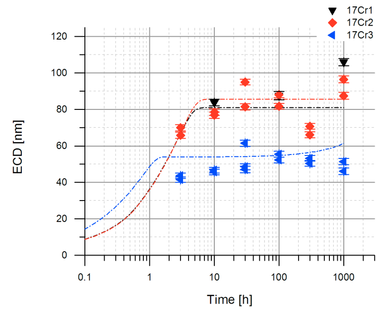
Figure 4.63: Precipitation of Laves phase particles in 17Cr1, 17Cr2, and 17Cr3 HiperFer steels during long term annealing at 650 °C
