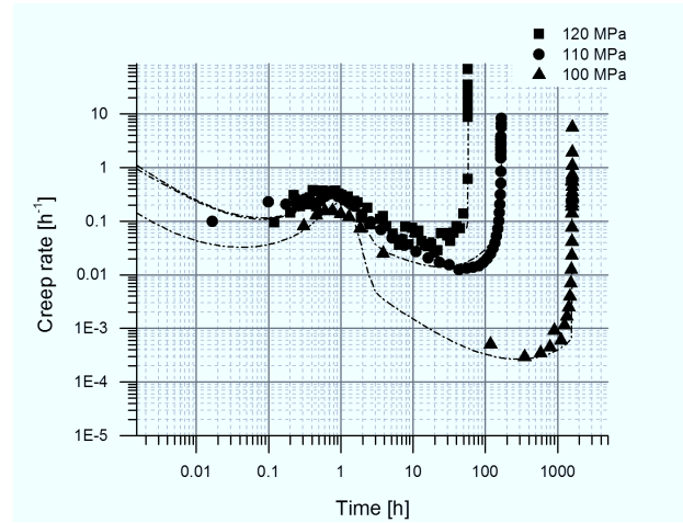
Figure 4.37: Creep rate curves of 17Cr1_1 specimens at 650 °C
