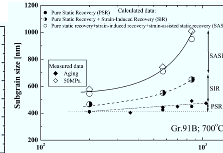
Figure 2.35: Subgrain coarsening of Gr. 91 steel due to three types of recovery mechanisms during long-term creep at 700 °C and 50 MPa [17]
