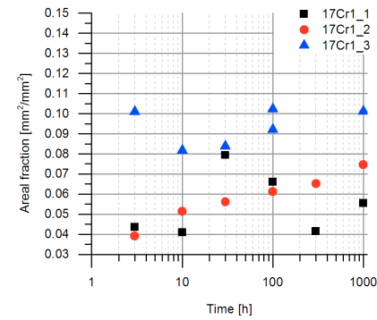
Figure 4.18: Areal fraction development of rolled 17Cr1 samples during isothermal annealing at 650 °C
