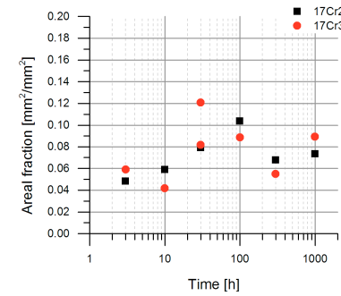
Figure 4.21: Laves phase particles areal fraction development of rolled 17Cr2 and 17Cr3 samples during isothermal annealing at 650 °C
