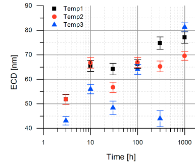
Figure 4.29: Laves phase particles equivalent circular diameter development of the tempered 17Cr1 samples during isothermal annealing at 650 °C
