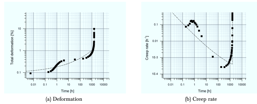
Figure 4.56: Creep deformation and creep rate curves of 17Cr1_1 steel at 100 MPa evaluated by the original model
