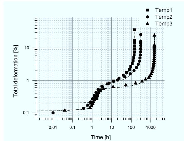
Figure 4.45: Creep deformation curve of recrystallized and low-temperature tempered 17Cr1 specimen at 650 °C/100 MPa
