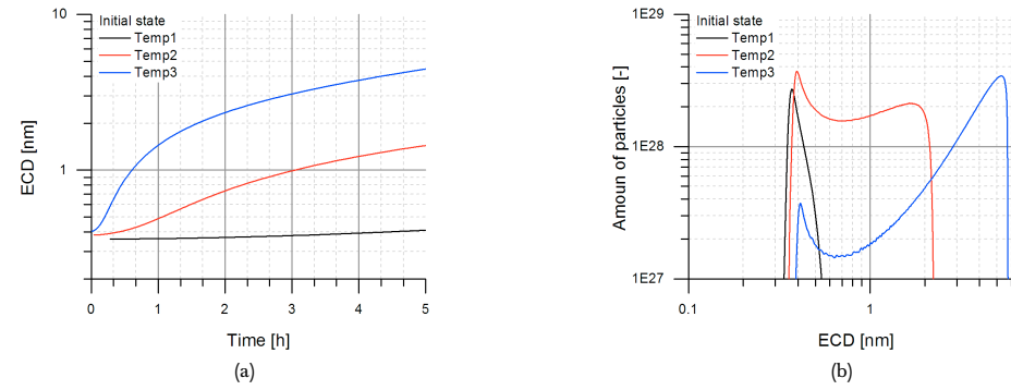
Figure 5.7: (a) Evolution of ECD and (b) size distribution of particles after 5 h of tempering at different temperatures: Temp1 - 475 °C, Temp2 - 510 °C, Temp3 - 540 °C
