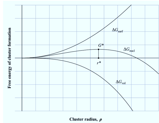
Figure 2.5: Schematic course of a function of the thermodynamic barrier [5]
