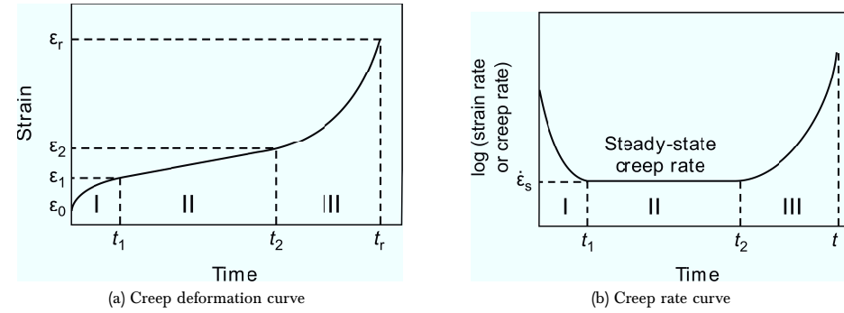
Figure 2.20: Typical creep deformation (a) and creep rate (b) curves showing the typical three stages [11]
