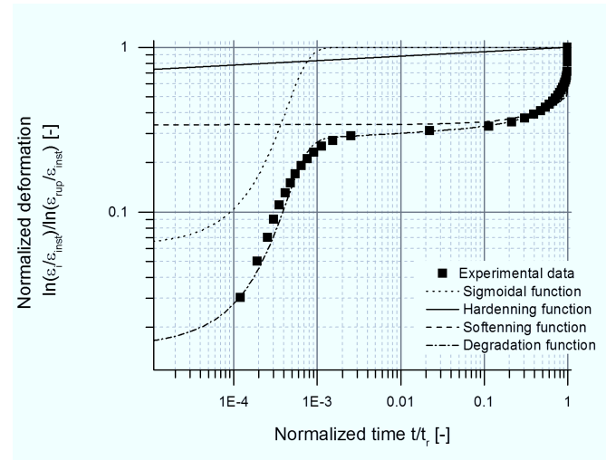
Figure 4.58: Creep curve of 17Cr1_1 steel at 100 MPa and 650 °C evaluated by the original model in double logarithmic plot
