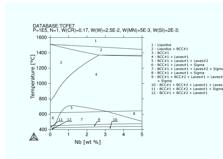
Figure 4.2: Phase fields as a function of Nb, nominal composition in wt% 17Cr, 2.5W, 0.5Mn, 0.2Si, XNb (ThermoCalc calculations utilizing TCFE7)
