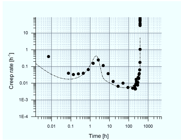
Figure 4.43: Creep rate curve of a recrystallized 17Cr1 specimen at 650 °C/100 MPa
