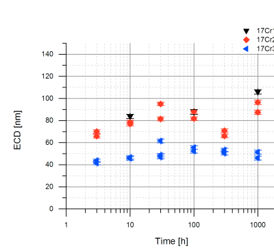
Figure 4.24: Equivalent circular diameter development of recrystallization annealed 17Cr1, 17Cr2, and 17Cr3 samples during isothermal annealing at 650 °C
