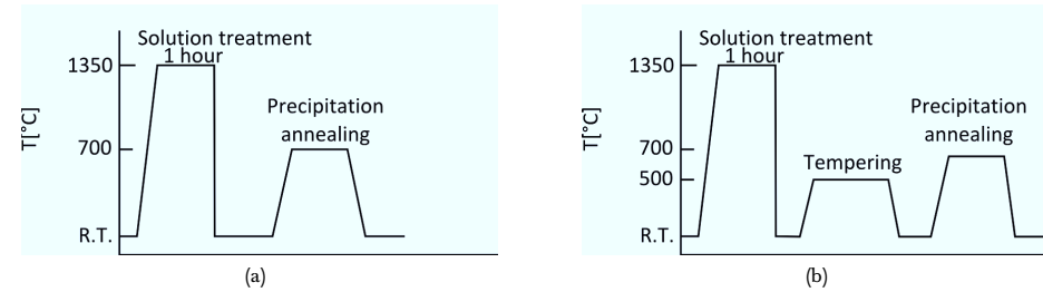
Figure 2.14: Schematic sketch of heat treatment procedures; (a) one step precipitation annealing, (b) two step annealing
