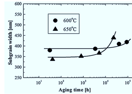
Figure 2.34: Coarsening of subgrains during aging at 600, and 650 °C [18]
