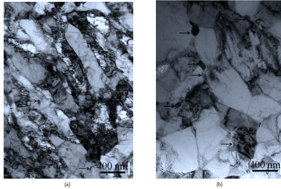
Figure 2.33: Typical TEM images of Gr. 91A steel aged at 650 °C for (a) 41, and (b) 23,000h. Arrows indicate precipitates [17]
