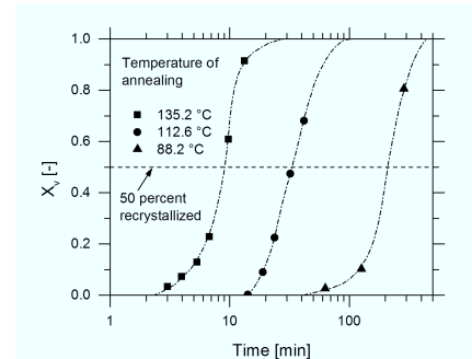
Figure 2.1: Isothermal recrystallization curves for pure copper cold rolled 98 % [4]
