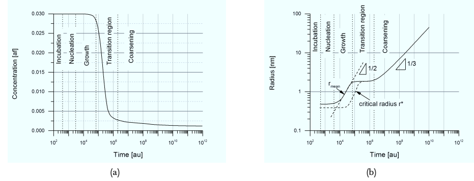
Figure 2.4: Evolution of matrix B-content (a), and (b) mean/critical radius during precipitation [5, 6]
