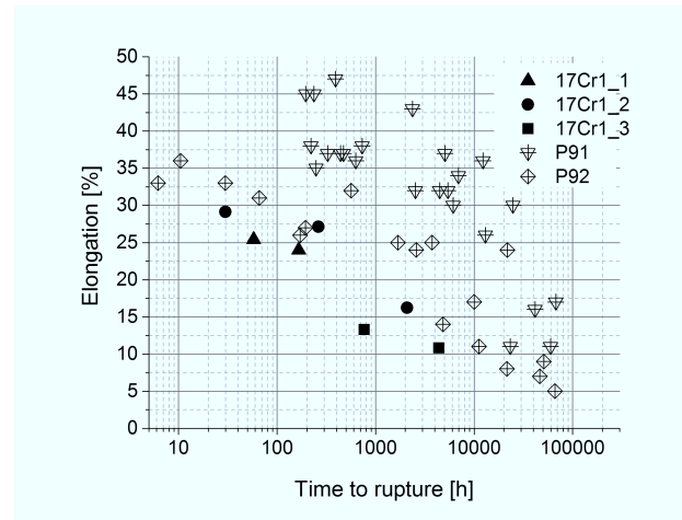
Figure 4.35: Time to rupture of rolled 17Cr1_1, 17Cr1_2, and 17Cr1_3 HiperFer steel at 650 °C
