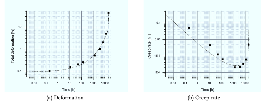
Figure 4.54: Creep deformation and creep rate curves of 1Cr05Mo025V steel tested at 500 °C and 177 MPa
