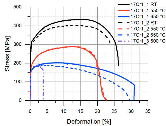
Figure 4.9: Tensile stress-strain curves of 17Cr1 steels at temperatures between ambient temperature and 650 °C
