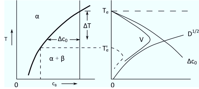
Figure 2.12: Influence of temperature T and oversaturation \Delta c_0 on the position and growth rate of a precipitate [7]
