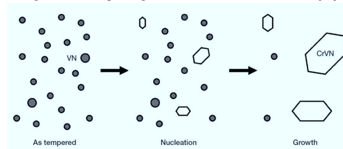
Figure 2.38: Transformation of finely distributed VN to coarse Z phase particles [20]
