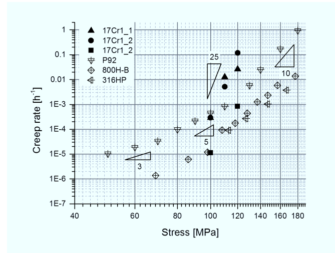
Figure 5.2: Creep strength of rolled 17Cr1 steel at 650 °C in comparison to 9-12 wt% Cr ferritic-martensitic, and austenitic steels
