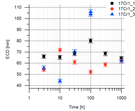
Figure 4.17: Equivalent circular diameter development of rolled 17Cr1 samples during isothermal annealing at 650 °C
