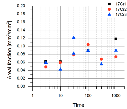
Figure 4.25: Areal fraction development of recrystallization annealed 17Cr1, 17Cr2, and 17Cr3 samples during isothermal annealing at 650 °C
