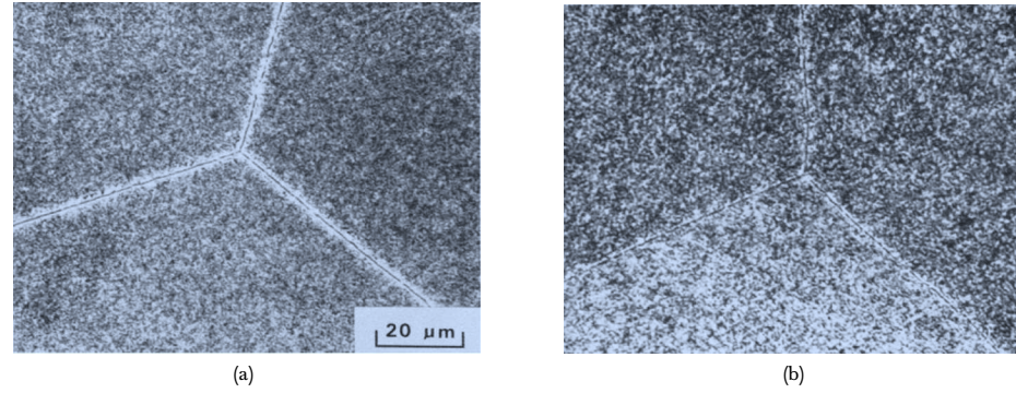
Figure 2.15: Macrostructure of the precipitation treated samples without (a) and with (b) tempering [9]
