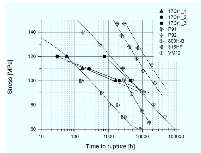
Figure 5.1: Creep strength of rolled 17Cr1 steel at 650 °C in comparison to 9-12 wt% Cr ferritic-martensitic, and austenitic steels
