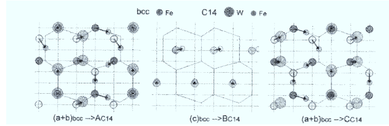
Figure 2.17: Diagrams presenting possible atomic displacements from bcc to C14 lattice. a, b, and c relate to the atomic planes along \langle 111 \rangle in the bcc lattice and A, B, C to the \{11\cdot 20\} planes in the C14 lattice [10]
