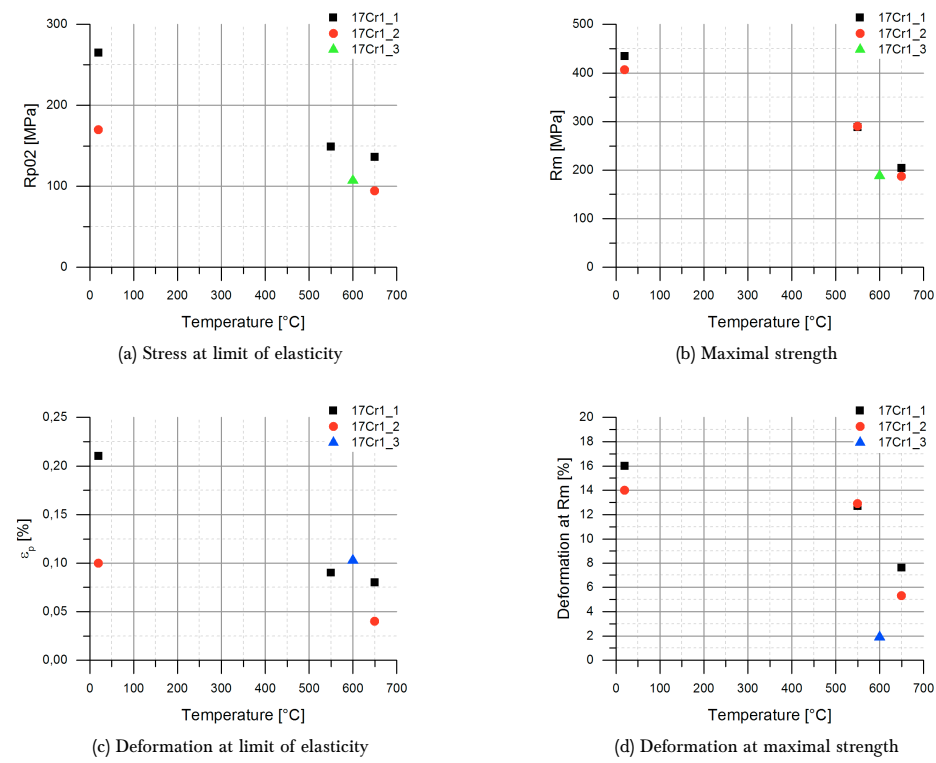
Figure 4.10: Tensile properties of 17Cr1 materials
