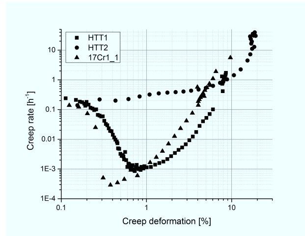
Figure 5.12: Creep rate curves of 17Cr1 materials in different initial thermo-mechanical treatment states: HTT1 - RA + 800 °C/15 min, HTT2 - RA+850 °C/15 min, rolled 17Cr1_1
