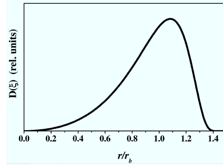
Figure 2.13: Predicted stationary size distribution for diffusion controlled coarsening according to the classical LSW theory [8]
