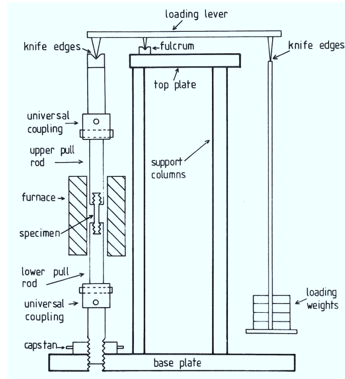
Figure 2.42: Sketch of a uniaxial top-lever creep machine [22]
