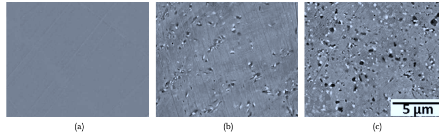
Figure 2.18: Backscattered electron images of AFA steel aged at 700 °C and 240 h; (a) without cold working; (b) after 50% of cold work; and (c) after 90 % of cold work
