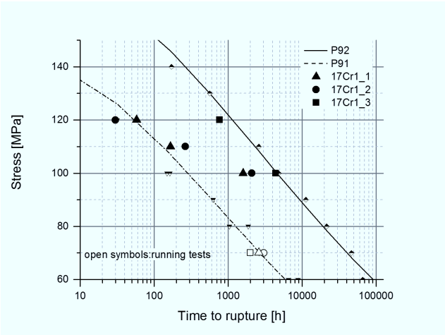
Figure 4.34: Time to rupture of rolled 17Cr1_1, 17Cr_2, and 17Cr_3 HiperFer steel at 650 °C
