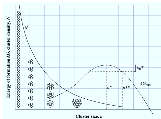
Figure 2.6: Equilibrium cluster distribution (solid line) and free energy of nucleus formation (dashed line) at the beginning of precipitation [5]
