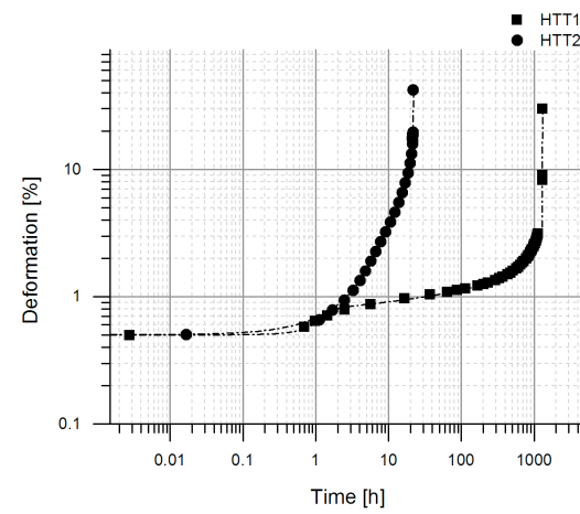
Figure 4.50: Creep deformation curves of the high temperature tempered 17Cr1 specimens at 650 °C/100 MPa
