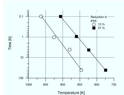
Figure 2.2: Temperature-time relationships for recrystallization of zirconium corresponding to two different degrees of prior cold work [4]
