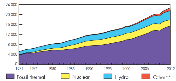
Figure 1.2: World electricity generation from 1971 to 2012 by fuel (TWh) [2]
