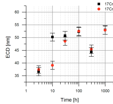
Figure 4.20: Laves phase particles equivalent circular diameter development of rolled 17Cr2 and 17Cr3 samples during isothermal annealing at 650 °C
