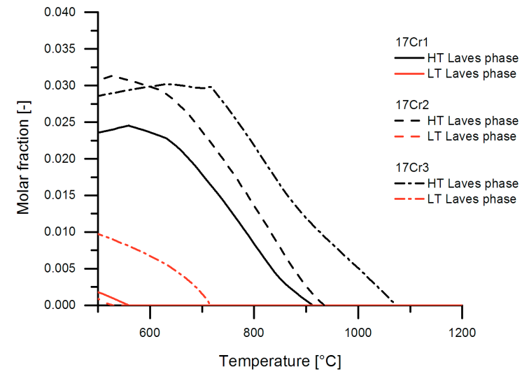
Figure 4.5: Stability regions of the High Temperature (\text{Fe,Cr,Si})_2(\text{Nb,W}) , and Low Temperature (\text{Fe,Cr,Si})_2(\text{Nb,W}) Laves phase (ThermoCalc calculations utilizing TCFE7)
