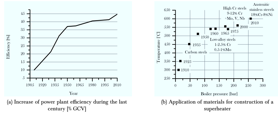
Figure 1.3: Change of efficiency of thermal power plants and materials used for their construction [3]
