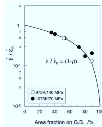
Figure 5.9: Decrease of minimum creep rate with increased grain boundary precipitation in Fe20Cr30Ni2Nb austenitic heat resistant steels [24]
