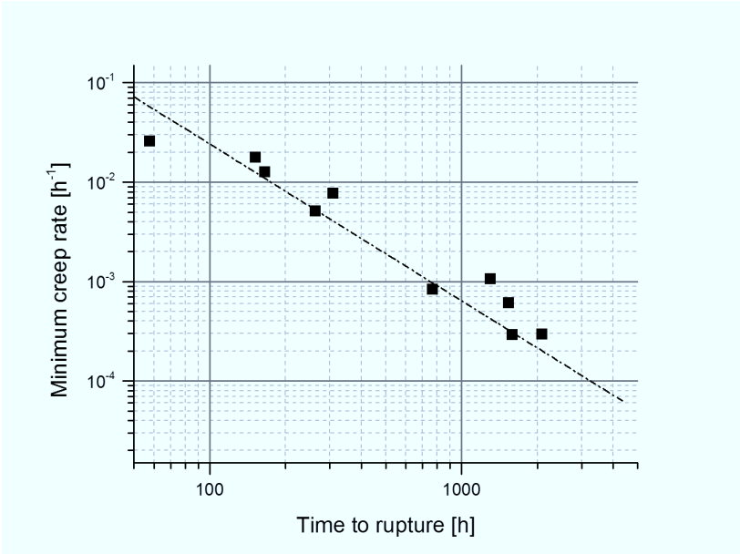
Figure 5.13: Relation of time to rupture and minimum creep rate of 17Cr1 creep experiments
