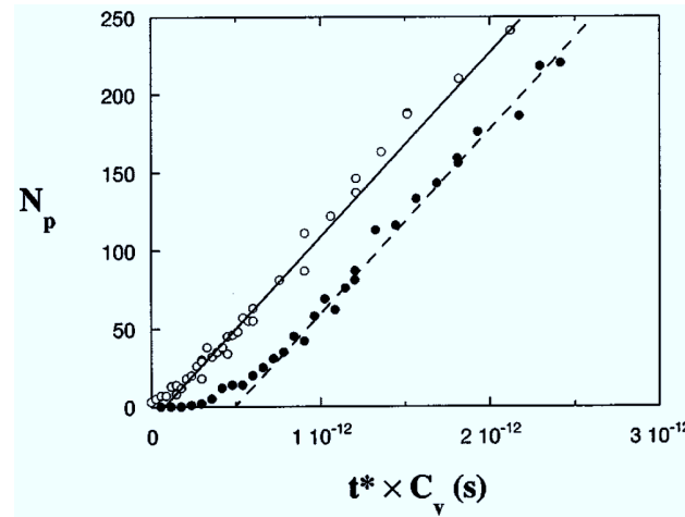
Figure 2.7: Analysis of solid-state nucleation kinetics—evolution of the number of supercritical clusters N_p at the beginning of the precipitation process [6]
