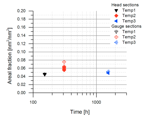
Figure 4.49: Areal fractions of particles in the low-temperature tempered 17Cr1 creep specimens
