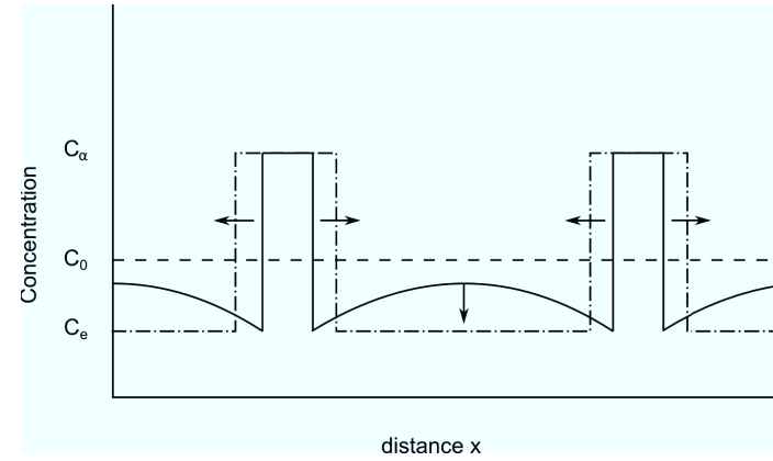
Figure 2.11: Interference of overlapping diffusion fields of simultaneously growing precipitates (full line), and after the end of particles growth (broken line)
