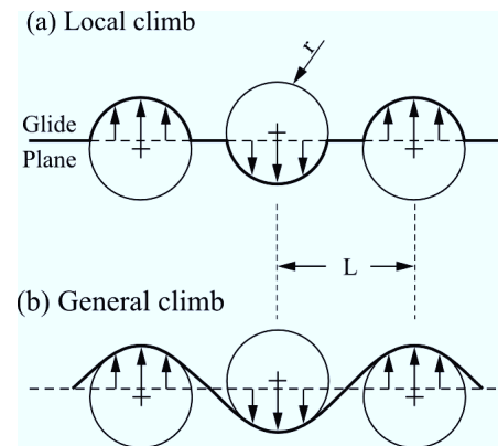
Figure 2.26: (a) Local, and (b) general climb over particles [15]
