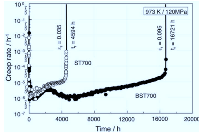
Figure 5.10: Creep rate curves of solution treated ST700, and boron doped BST700 austenitic steels [24]
