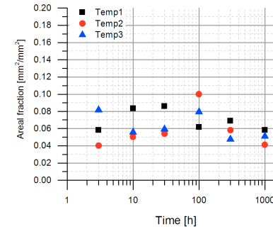
Figure 4.30: Precipitates areal fraction development of the tempered 17Cr1 samples during isothermal annealing at 650 °C
