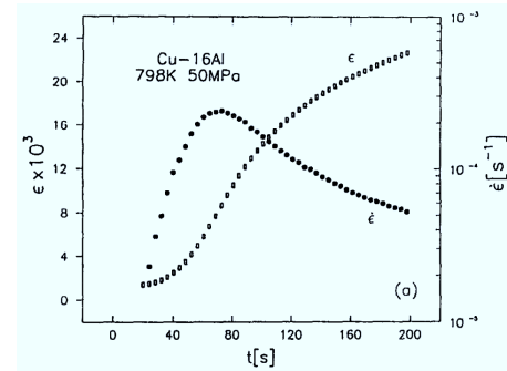
(a) Sigmoidal creep deformation and creep rate curves of a Cu-16Al solid solution alloy [33]
