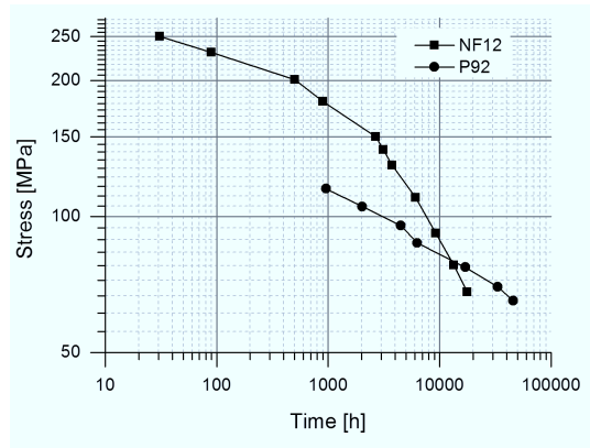
Figure 2.37: Creep strength of P92 and NF12 steel at 650 °C [20]
