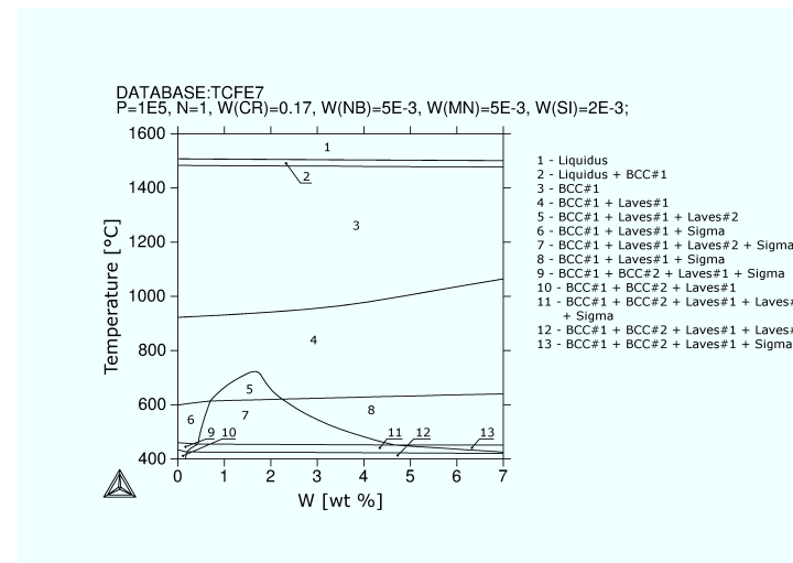
Figure 4.1: Phase fields as a function of W, nominal composition in wt% 17Cr, 0.5Nb, 0.5Mn, 0.2Si, XW (ThermoCalc calculations utilizing TCFE7)
