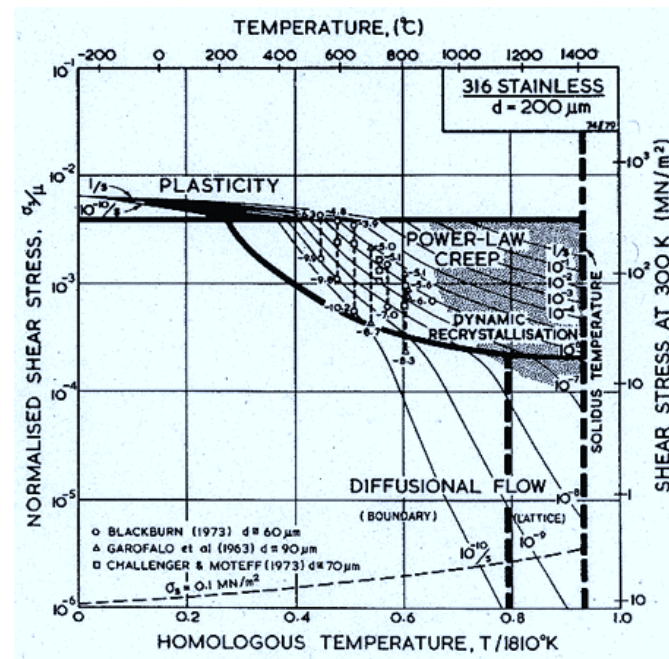
Figure 2.23: Creep deformation map of 316 stainless steel [12]
