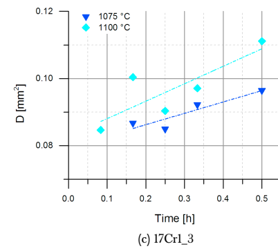
Figure 4.14: Coarsening of grains of 17Cr1 steels at 1075 and 1100 °C
