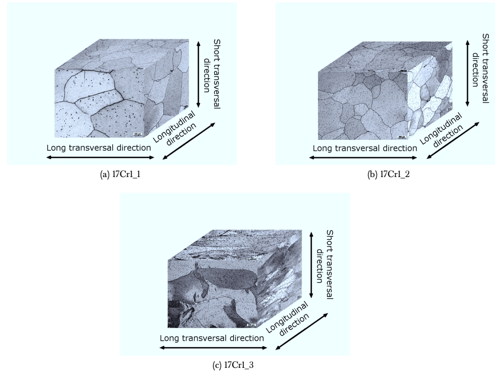
Figure 4.7: Grain structure of rolled 17Cr1 steel in different rolling directions
