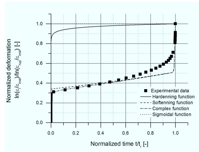
Figure 4.57: Normalized creep deformation data of 17Cr1_1 steel at 100 MPa and 650 °C evaluated by the modified model
