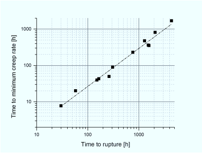
Figure 5.15: Relation of time to rupture to time to minimum creep rate
