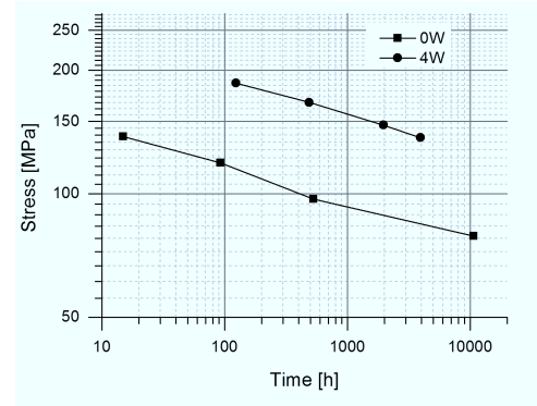
Figure 2.39: Influence of W addition on creep strength of 9 wt. % Cr steel [21]
