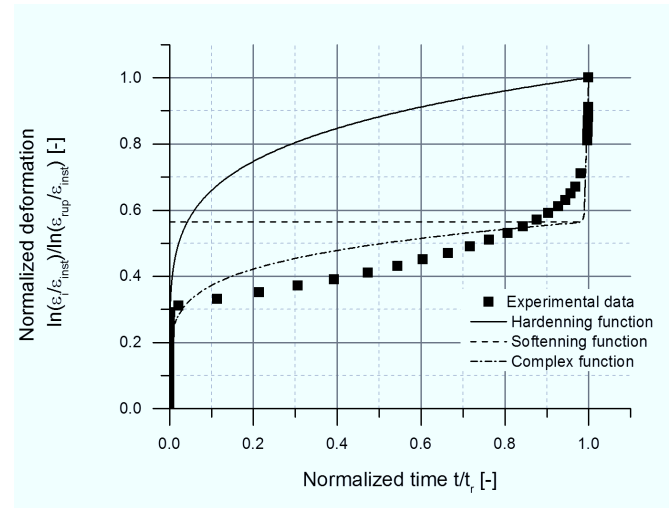
Figure 4.55: Normalized creep deformation data of 17Cr1_1 steel at 100 MPa evaluated by the original model
