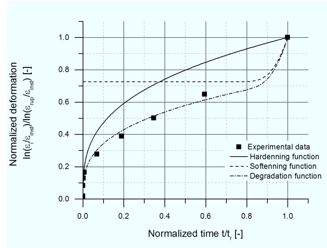
Figure 4.53: Normalized creep deformation data of 1Cr05Mo025V steel tested at 500 °C and 177 MPa
