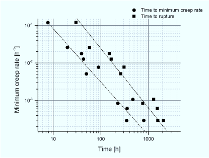
Figure 5.14: Monkman-Grant graph for time to rupture and time to minimum creep rate
