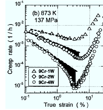
Figure 2.40: Influence of W addition on creep rate curves of 9 wt. % Cr steel [21]
