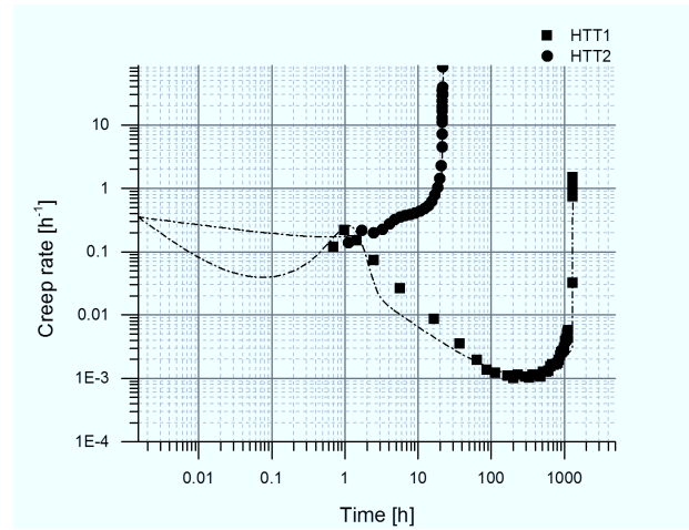
Figure 4.51: Creep rate curves of the high temperature tempered 17Cr1 specimens at 650 °C/100 MPa
