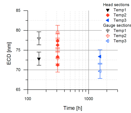
Figure 4.48: ECD of particles in the low-temperature tempered 17Cr1 creep specimens
