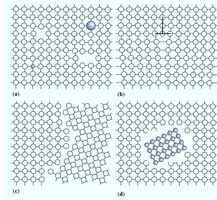
Figure 2.8: Lattice defects acting in heterogeneous precipitation; (a) a mono- and a divacancy, larger and smaller atoms, (b) edge dislocation, (c) high angle grain boundary, and (d) incoherent inclusion [5]
