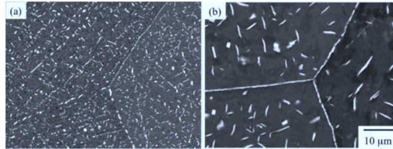
Figure 5.8: Microstructures of model austenitic steels after annealing at 800 °C/1,200 h: (a) original ST700, (b) modified BST700 [24]
