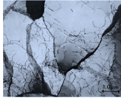
(a) Subgrains in AISI 304 stainless steel torsionally deformed at 865 °C at \dot{\epsilon} = 3.2 \times 10^{-5} \text{ s}^{-1} to a strain of 0.38 [32]
