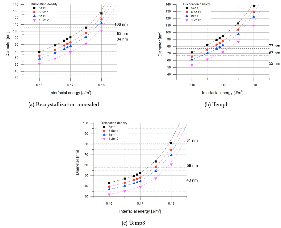
Figure 4.61: Influence of interfacial energy and dislocation density on the predicted size of Laves phase particles in 17Cr1 steel in different initial heat treatment states: (a) recrystallization annealed (RA), (b) Temp1 state - RA + 475 °C/5 h, (c) Temp3 state - RA + 540 °C/5 hours
