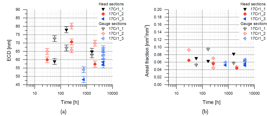
Figure 4.41: Evaluated ECD (a) and areal fraction (b) of Laves phase particles in ruptured creep specimens
