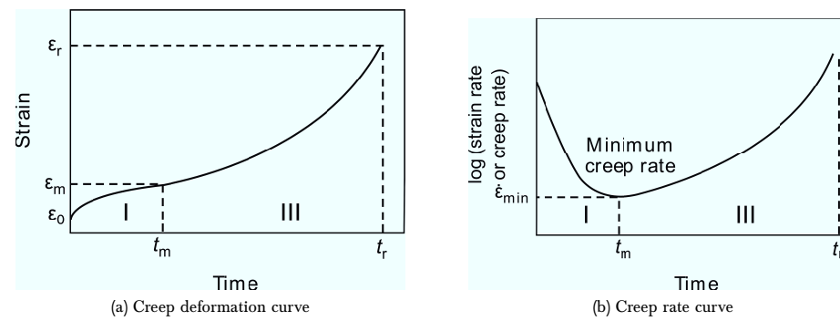
Figure 2.21: Creep deformation (a) and creep rate (b) curves without the secondary stage [11]
