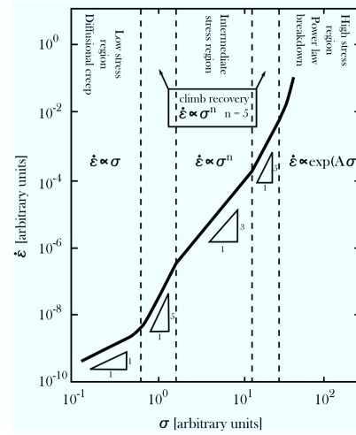
Figure 2.30: Schematic representation of stress dependence of creep rate showing Class M \rightarrow Class A \rightarrow Class M transition [16]
