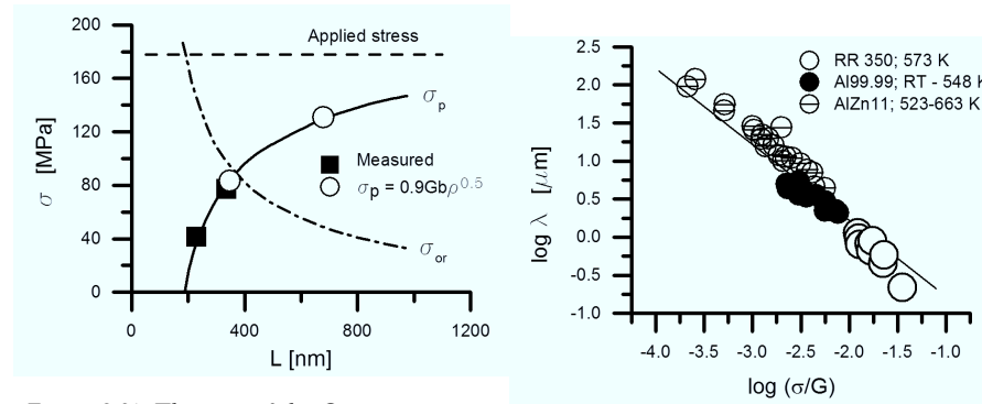
Figure 2.31: The sum of the Orowan stress in the \gamma' -strengthened stainless steel A-286 and the stress \sigma_{or} available for dislocation generation equals to the applied stress and varies with interparticle distance L .
