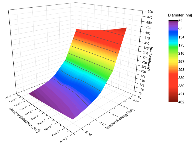
Figure 4.60: Influence of dislocation density and interfacial energy on predicted size of Laves phase particles in 17Cr1 steel (recrystallized state)
