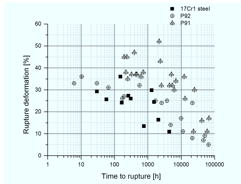
Figure 5.16: Rupture deformation of all the 17Cr1 creep specimens in comparison to P91 and P92 steels
