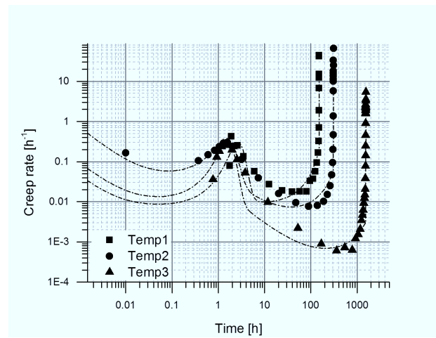
Figure 4.46: Creep rate curve of recrystallized and low-temperature tempered 17Cr1 specimen at 650 °C/100 MPa
