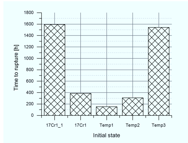
Figure 5.4: Time to rupture of 17Cr1 steel in different initial states - rolled 17Cr1_1, recrystallized (1075 °C/15 min) 17Cr1, and tempered Temp1 (1075 °C/15 min + 475 °C/5 h), Temp2 (1075 °C/15 min + 510 °C/5 h) and Temp3 (1075 °C/15 min + 540 °C/5 h)
