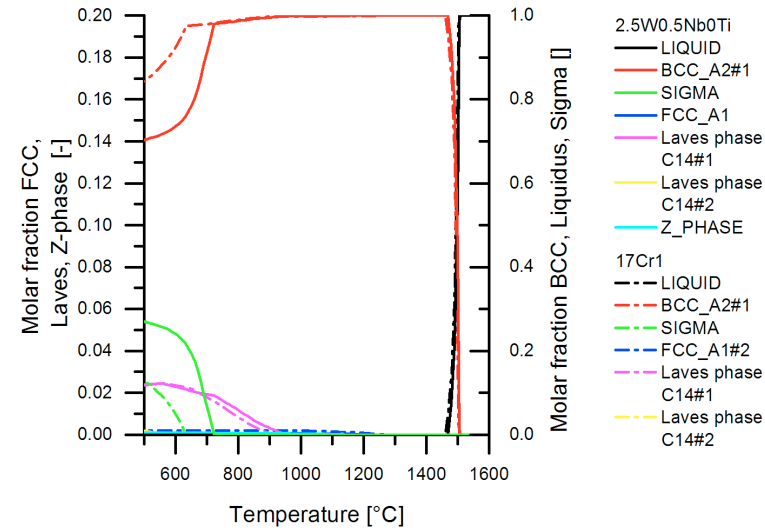
Figure 4.4: Phase diagram of the 2.5W0.57Nb0Ti, and 17Cr1 steel (ThermoCalc calculations utilizing TCFE7)
