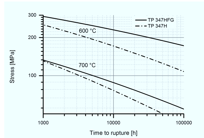
Figure 2.27: Creep rupture strength of austenitic steels TP347H, and TP347HFG [14]
