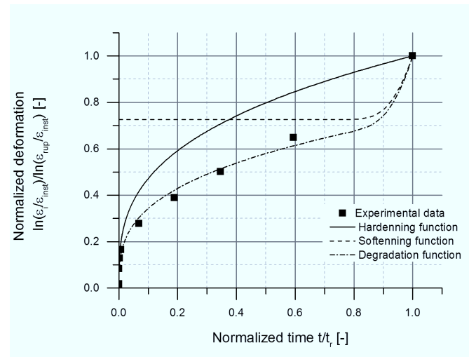
Figure 2.41: Normalized creep deformation data of 1Cr0.5Mo0.25V steel tested at 500 °C and 177 MPa
