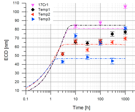
Figure 5.6: Observed (points) and modeled (curves) change of ECD of Laves phase particles in HiperFer 17Cr1 steel in different initial states: recrystallization annealed 17Cr1 (RA, 1075 °C/15 min), and tempered Temp1 (RA+475 °C/5 h), Temp2 (RA+510 °C/5 h), and Temp3 (RA+540 °C/5 h)
