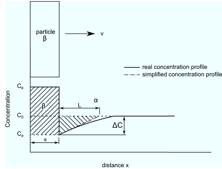
Figure 2.10: Diffusion-controlled growth of the precipitate \beta from supersaturated solution \alpha
