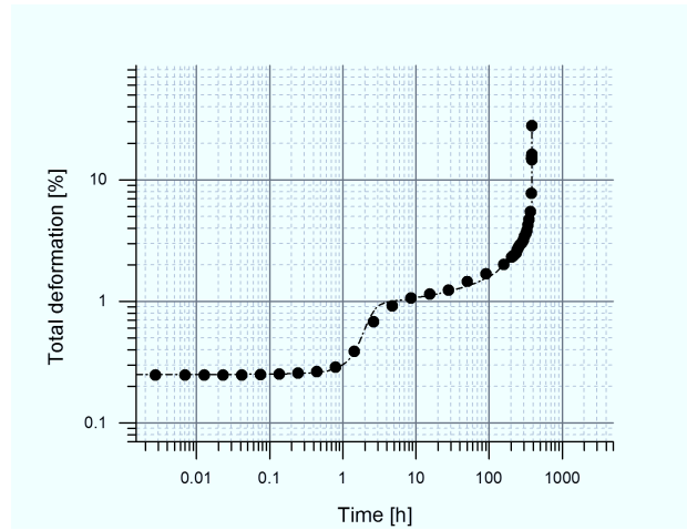
Figure 4.42: Creep deformation curve of a recrystallized 17Cr1 specimen at 650 °C/100 MPa
