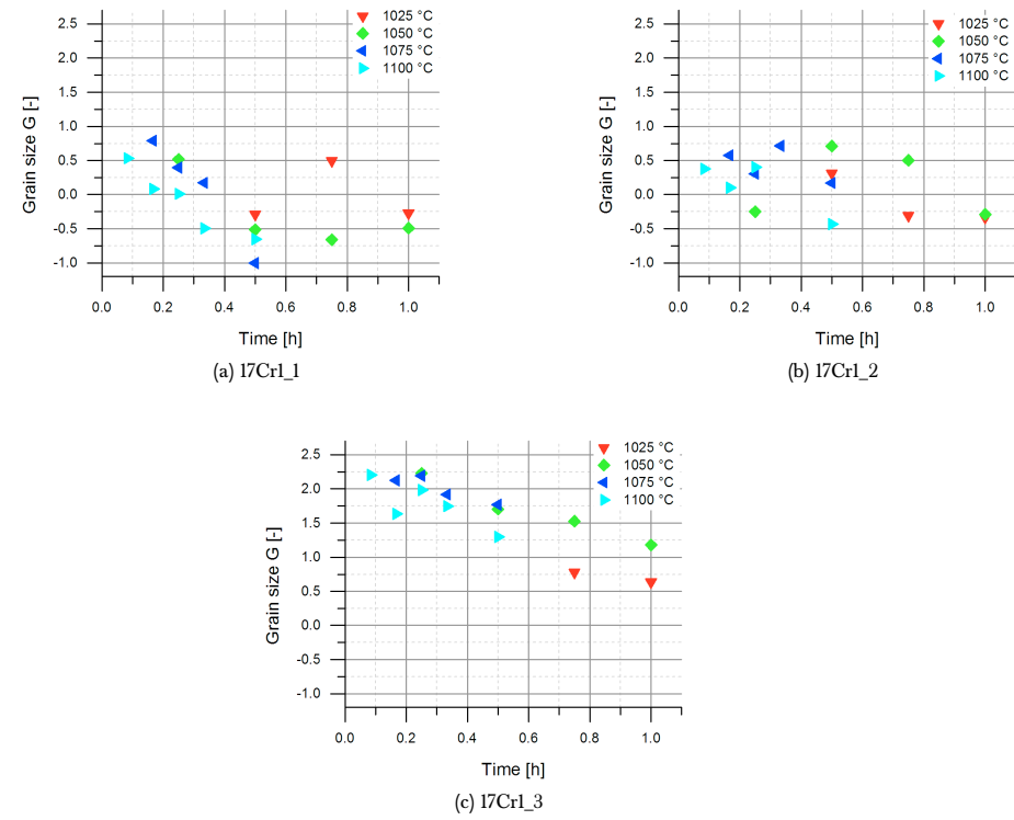
Figure 4.13: Grain size development of 17Cr1 steel during annealing at temperatures 1,025-1,100 °C
