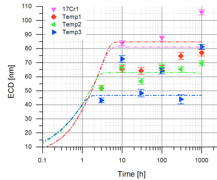
Figure 4.62: Precipitation of Laves phase particles in 17Cr1 steel with different initial heat treatments during long term annealing at 650 °C; comparison of observed (points) and modeled (curves) values
