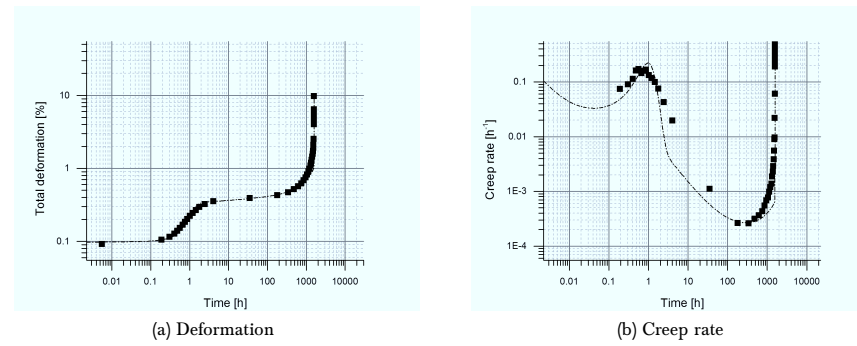
Figure 4.59: Creep deformation and creep rate curves of 17Cr1_1 steel at 100 MPa and 650 °C evaluated by the modified model
