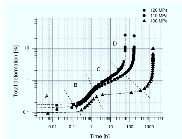
Figure 4.36: Creep deformation curves of 17Cr1_1 specimens at 650 °C
