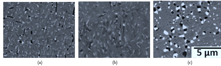
Figure 2.19: Backscattered electron images of AFA steel aged at 800 °C and 240 h; (a) without cold working; (b) after 50% of cold work; and (c) after 90 % of cold work
