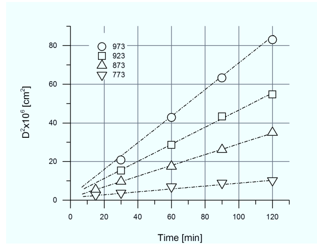
Figure 2.3: Grain-growth isotherms for brass [4]
