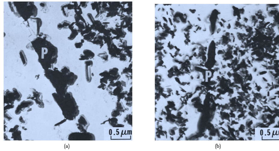
Figure 2.16: TEM image of an extraction replicas taken from a grain boundary of material without (a) and with (b) tempering prior to precipitation annealing [9]
