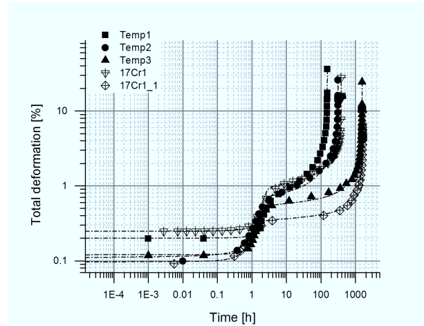
Figure 5.5: Evolution of creep deformation of 17Cr1 steel in different initial states - rolled 17Cr1_1, recrystallized (1075 °C/15 min) 17Cr1, and tempered Temp1 (1075 °C/15 min + 475 °C/5 h), Temp2 (1075 °C/15 min + 510 °C/5 h) and Temp3 (1075 °C/15 min + 540 °C/5 h)
