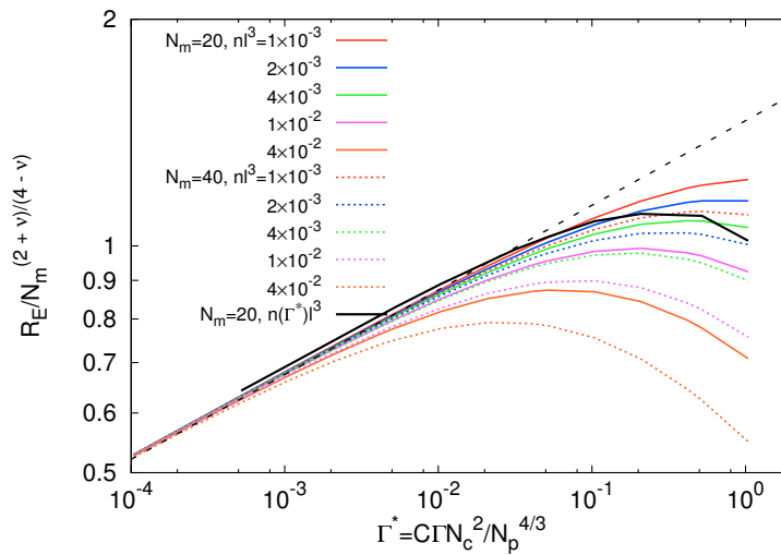
Figure 2. Theoretical prediction of the dependence of the polymer extension on the effective interaction strength \Gamma^* for various ion concentrations n and the polymer lengths N_m = 20 and 40 . The thick black line is the simulation result for N_m = 20 , N_c = 147 and L/l = 200 [26].
