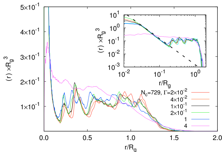
Figure 9. Normalized radial distribution functions P(r) of monomers, with respect to the microgel center of mass, for various interaction strengths of nanogels with N_c = 729 and L/l = 400 . The inset shows the distribution function on a log-log scale. The dashed lines is proportional to r^{-2} . The radii of gyration of the microgels are R_g/l = 75.1, 77.1, 81.7, 82.1, 78.2 and 40.2 with increasing \Gamma .
