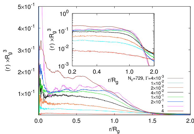
Figure 13. Normalized radial counterion distribution functions P(r) , with respect to the microgel center of mass, for various interactions strengths and the microgel of size N_c = 729 and L/l = 400 . The inset shows the same quantities in a semilogarithmic representation. The radii of gyration of the microgels are R_g/l = 56.7, 67.7, 75.1, 77.1, 81.7, 78.2 and 40.2 with increasing \Gamma .
