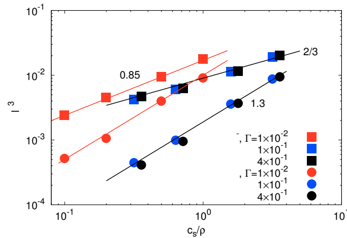
Figure 6. Density of ions inside a microgel as a function of the salt concentration for microgels with N_c = 147 and L/l = 200 and the indicated interaction strengths. The squares represent the total concentration of negatively-charged ions, i.e., counterions plus salt ions. The bullets represent the positively-charged salt ions.
