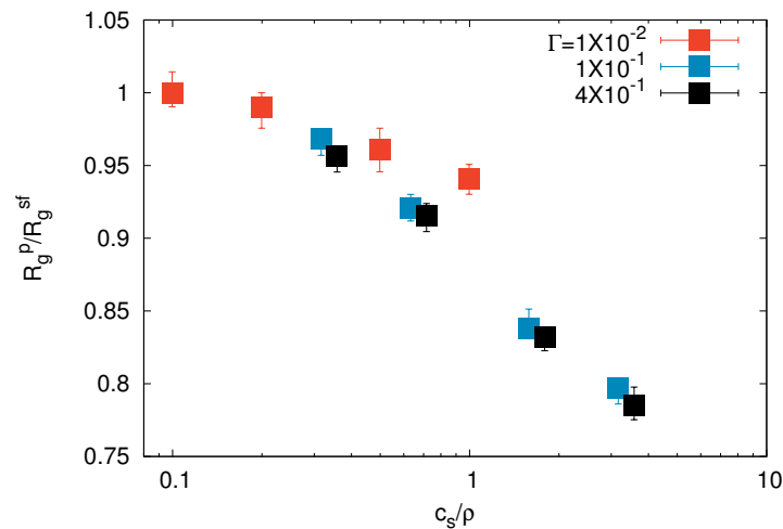
Figure 5. Dependence of the average radius of gyration of individual polymers R_g^p on the ratio of the salt concentration c_s and network charge density \rho for N_c = 147 and L/l = 200 . R_g^{sf} is the polymer radius of gyration of the salt-free system.
