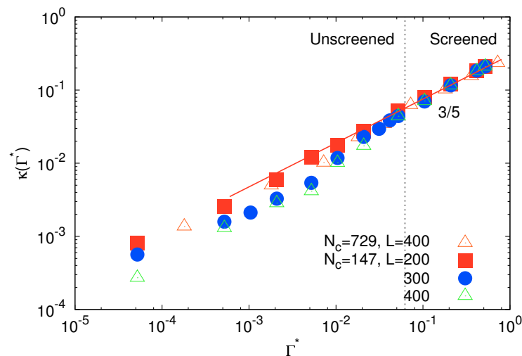
Figure 4. Inverse Debye screening length as a function of the scaled interaction strength for microgels with N_c = 147 and 729 crosslinks. For the larger microgel, the size of the simulation box is L/l = 400 , and for the smaller one with N_c = 147 , the boxes are L/l = 200, 300 and 400.
