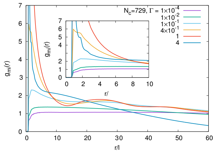
Figure 15. Monomer-counterion pair correlation functions for various interaction strengths \Gamma . The number of crosslinks is N_c = 729 , and the box size L/l = 400 . The inset shows the correlation functions over a smaller range r/l .
