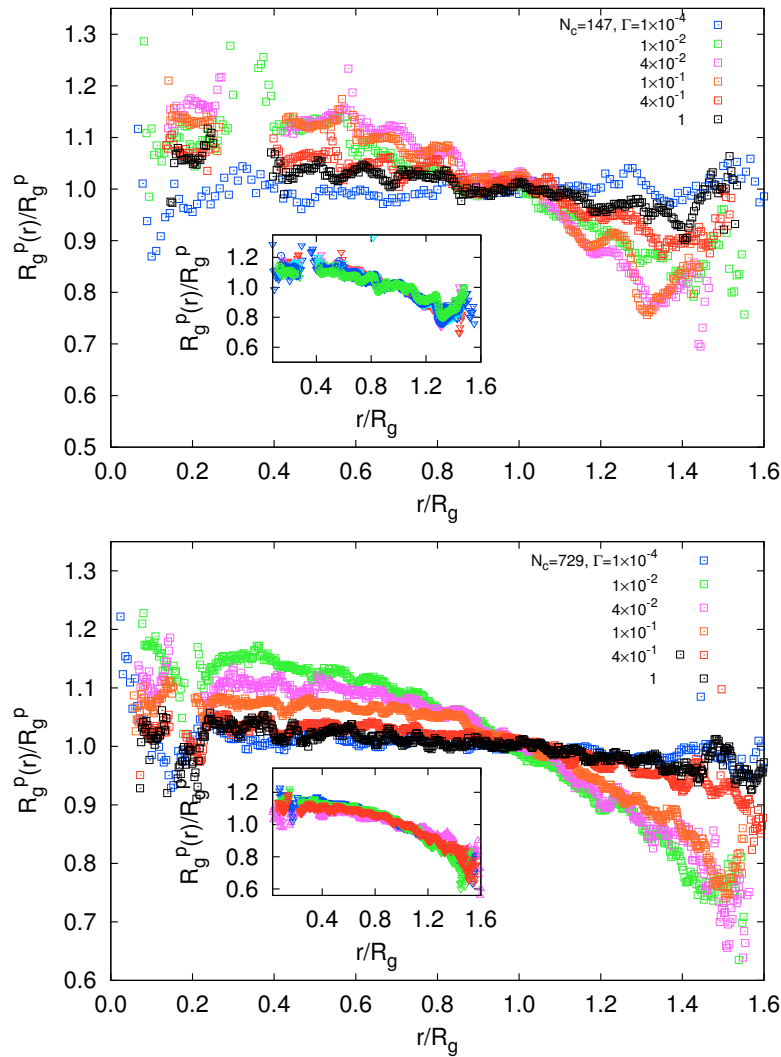
Figure 10. Dependence of the polymer radius of gyration on its radial center-of-mass position r for (top) N_c = 147 and L/l = 300 , and (bottom) for N_c = 729 and L/l = 400 . The insets show radii of gyration in the unscreened regime. The radii of gyration of the microgels are (top) R_g/l = 17.9, 31.7, 40.5, 44.6, 45.7 and 44.0 , and (bottom) R_g/l = 33.9, 67.7, 77.1, 81.7, 80.7 and 40.2 with increasing \Gamma .
