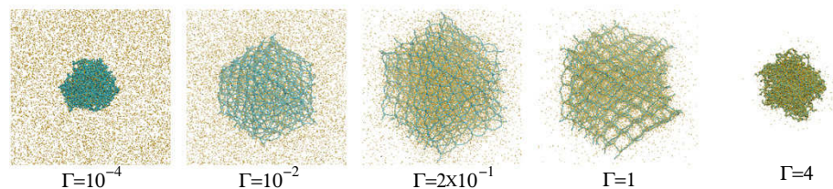
Figure 1. Snapshots of gel particles (blue) with N_c = 729 crosslinks in the presence of counterions (yellow) for various Coulomb interaction strengths \Gamma as indicated.
