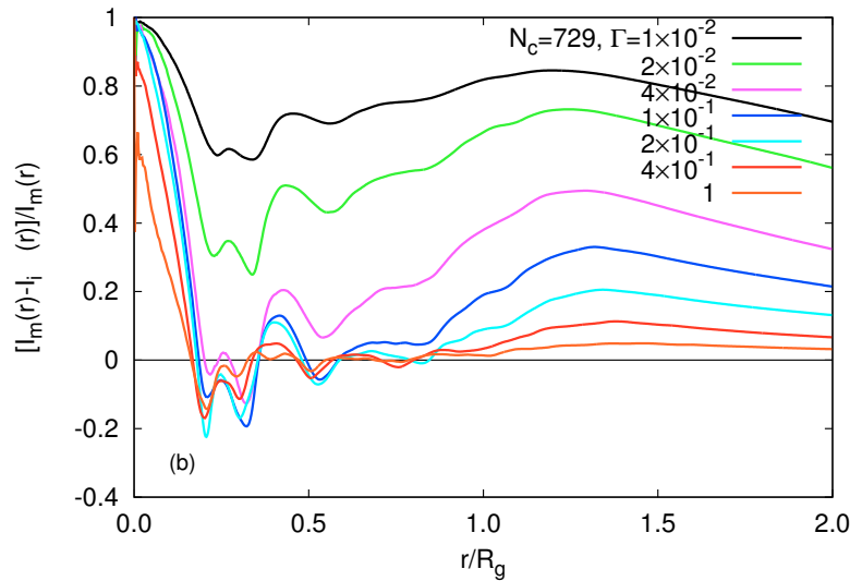
Figure 14. Ratio of the monomer-counterion charge difference and the monomer charge (cf. Equation (16)) as a function of the radial distance from the microgel center for the indicated interaction strengths and the microgel of size N_c = 729 with L/l = 400 . The radii of gyration of the microgels are R_g/l = 67.7, 75.1, 77.1, 81.7, 82.2, 80.7 and 78.2 with increasing \Gamma .
