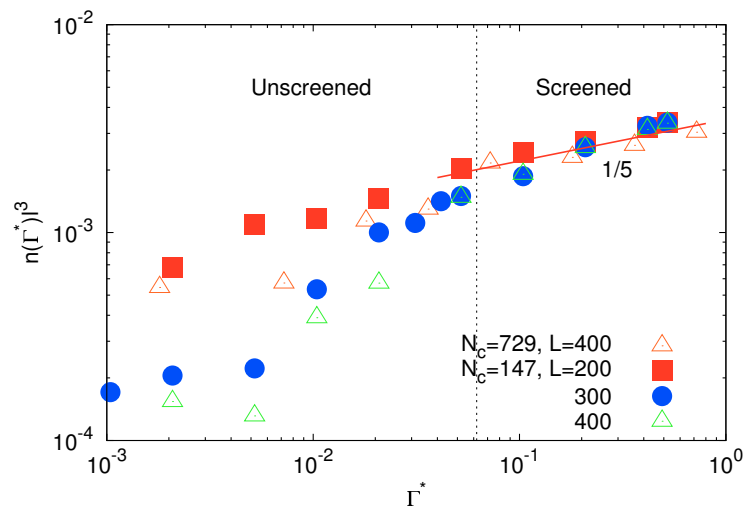
Figure 3. Density of counterions inside a microgel as a function of the scaled interaction strength for microgels with N_c = 147 and 729 crosslinks. For the larger microgel, the size of the simulation box is L/l = 400 , and for the smaller one with N_c = 147 , the boxes are L/l = 200, 300 and 400.
