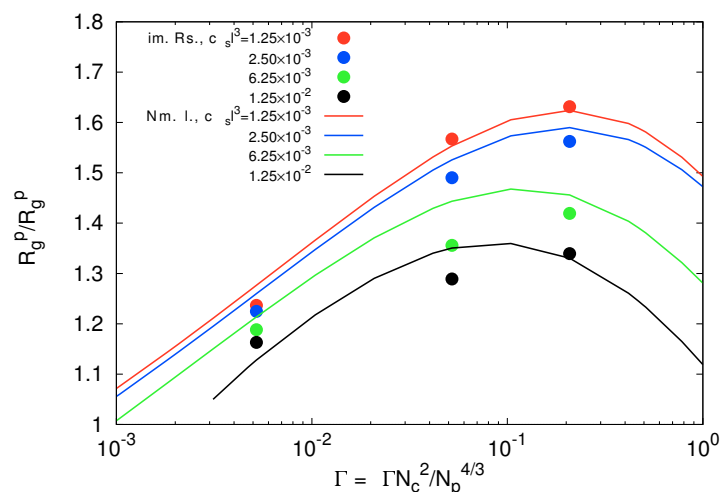
Figure 8. Average radii of gyration R_g^p of individual polymers as a function of the interaction strength \Gamma^* for microgels with N_c = 147 and various salt concentrations c_s . The average radius of gyration of the neutral system is R_g^{pm}/l = 2.6 . The theoretical curves follow for the parameters C = 0.032 and \hat{C} = 1.5 .
