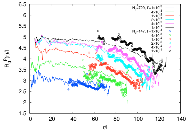
Figure 11. Dependence of the polymer radius of gyration on its radial center-of-mass position r for microgels with N_c = 729 and L/l = 400 (lines), and N_c = 147 and L/l = 300 (circles). The latter are radially shifted to match the respective microgel surface.
