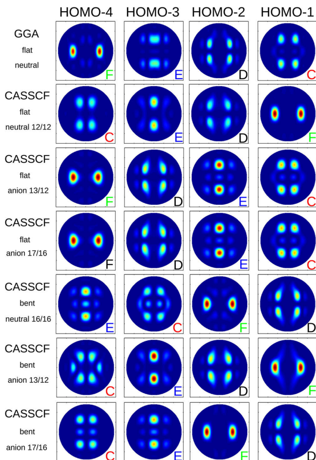
Figure 4. Theoretical photoelectron angular distributions (PADs) for the PTCDA orbitals C, D, E, and F ordered according to the binding energy from right to left. The top row depicts PADs of the Kohn–Sham orbitals using a GGA, while the remaining rows are based on natural orbitals of various CASSCF calculations.
