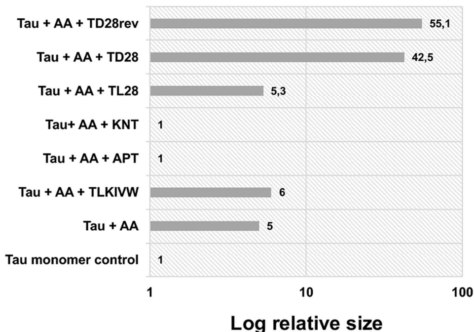
Fig 4. Effect of the selected peptides on tau aggregation, measured by DLS. Recombinant tau was dissolved in PBS to a concentration of 21.8 \mu M (1 mg/ml). As positive control, AA was added to a concentration of 100 \mu M. The peptides were added in a ratio of 1:10 (tau:peptide) and 100 \mu M AA. All samples were incubated for 24 hours. DLS was performed with an acquisition time of 5 seconds for 3 minutes at room temperature. The ratio of the hydrodynamic radii of tau protein in the presence of the peptides to tau fibrils (positive control) was calculated. The error was below 10% for all measurements, the mass was \geq 99\% .
