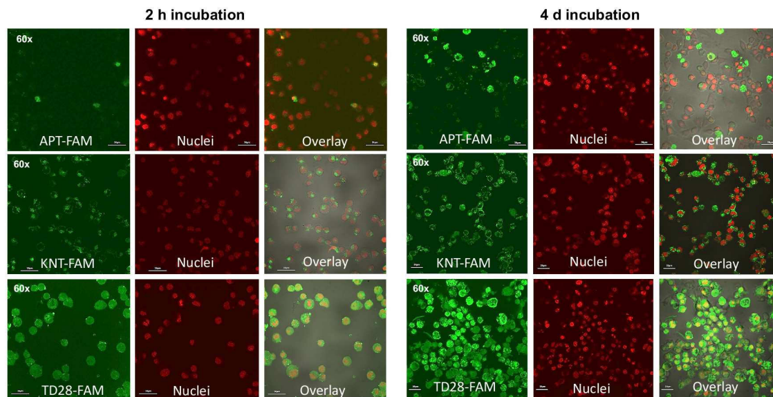
Fig 5. Inducible N2aTau 4RΔK280 cells were incubated with 60 μM of the respective, FAM-labeled peptide for two hours and four days. After incubation, the cells were fixed on glass cover slips and the locations of the respective peptide were detected by the FAM-label (green). In addition, cell nuclei were stained with TOPRO3 dye (red). Here, representative pictures for APT-FAM, KNT-FAM and TD28-FAM are shown in 60 times magnification. Scale bar: 30 μm.
