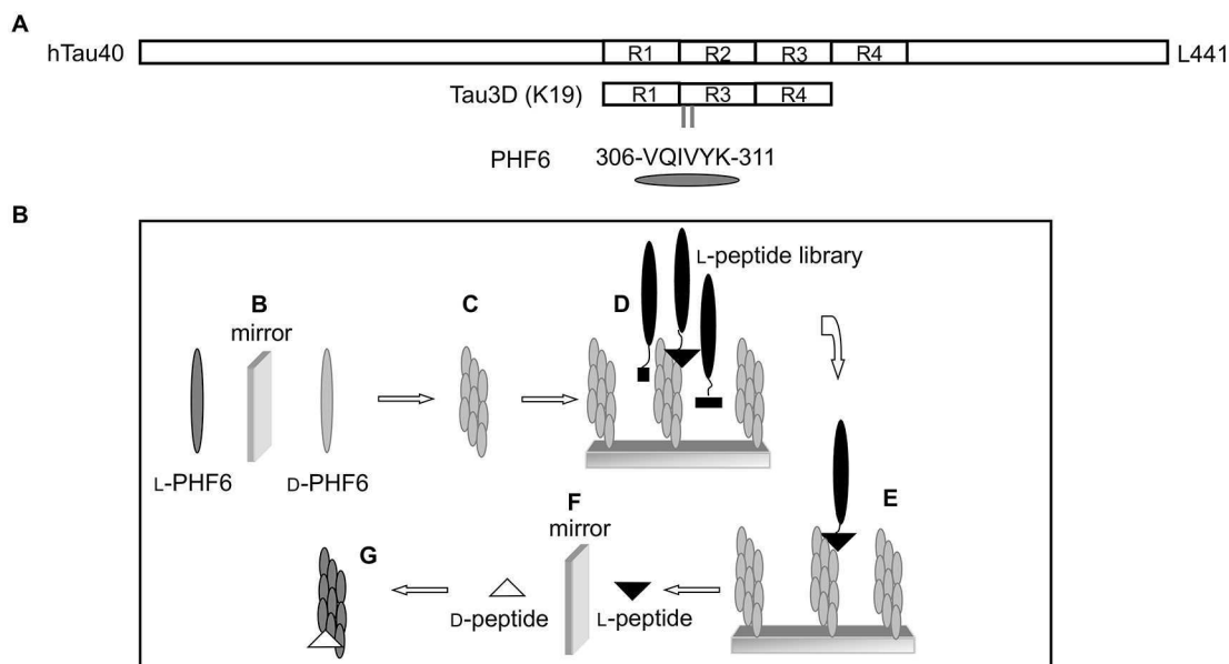
Fig 1. Tau constructs and principle of the mirror image phage display selection. (A) The largest human tau isoform in the central nervous systems contains four microtubule binding repeats, whereas the tau construct tau 3RD (K19) lacks repeat 2 [42]. PHF6, consisting of amino acids 306 to 311, is located at the beginning of repeat three. (B) The D-enantiomeric form of PHF6 was synthesized. (C) After fibrillization, the D-enantiomeric fibrils were used for phage display (D). (E) An L-peptide, binding to the D-enantiomeric PHF6 fibrils, was selected. (F) The D-enantiomeric version of the selected L-peptide was synthesized, which (G) will bind to the L-enantiomeric form of the target, regular PHF6 fibrils.
