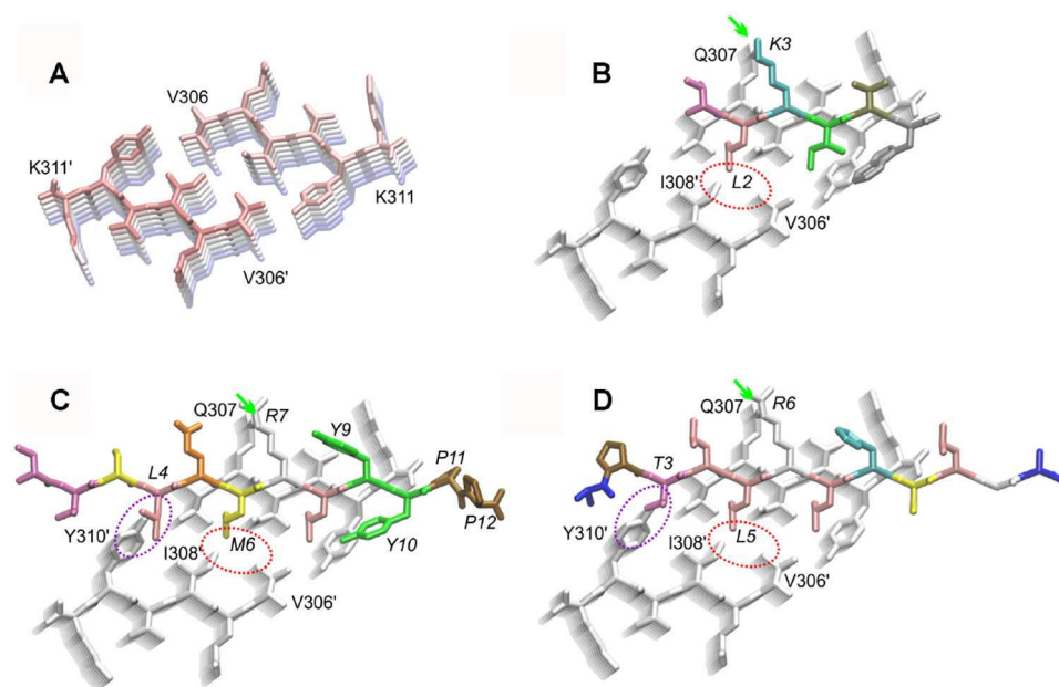
Fig 6. Structure of the tau fibril and binding mode of different \alpha -peptides. (A) Crystal structure of the steric zipper formed by the PHF6 peptide. The first and last residue for each of the two stacks of interacting \beta -sheet is labeled. The individual layers of \beta -sheet within each stack are gradually colored from red to blue. (B) Binding mode of the TLKIVW peptide according to Sievers et al. [19]. The side chain interaction between K3 and Q307 is marked by a green arrow. The red ellipse denotes steric repulsion between L2 of TLKIVW and V306/I308 of the second stack of \beta -strands. Peptide residues are labeled in italic. (C) Binding mode of the TD28 peptide. Same type of presentation as in (B); an additional repulsive interaction formed between L4 and Y310 is highlighted by a magenta ellipse. (D) Binding mode of the APT peptide. Same type of presentation as in (B); an additional repulsive interaction formed between T3 and Y310 is highlighted by a magenta ellipse.
