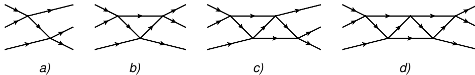
FIG. 1: Examples of diagrams contributing to the particle-bound state scattering amplitude at leading order.
